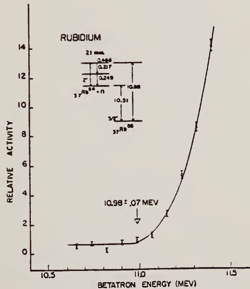
FIG. 6. Relative activity of the 21-minute isomeric state of Rb^{86} as a function of betatron energy.
