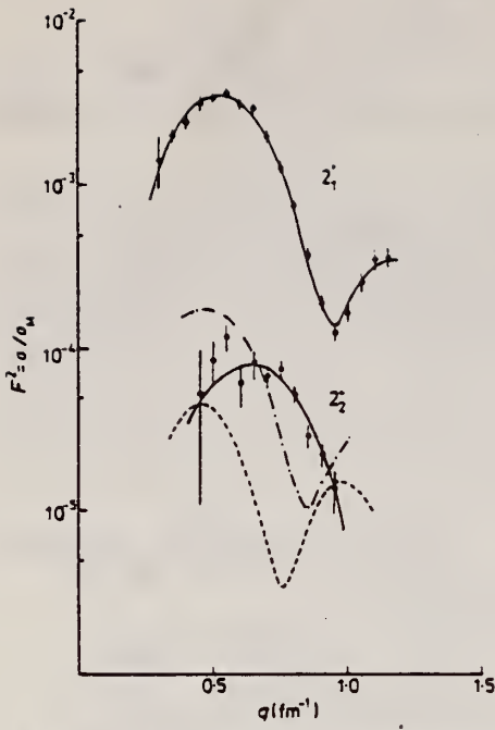
Figure 4. 2_1^+ and 2_2^+ form factors—anharmonic model fits. The fits to the 2_2^+ are respectively \cos \phi = -1 (—), \cos \phi = +1 (—) and pure harmonic two-phonon (---).
