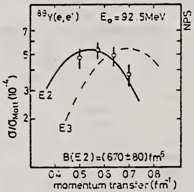
FIG. 9. Relative DWBA cross section using the Goldhaber-Teller model as compared with the resonance at 28 MeV assuming a width of \Gamma=9 MeV. The comparison shows that the cross section in this region is predominantly E2 with the possibility of some E3 contribution.
