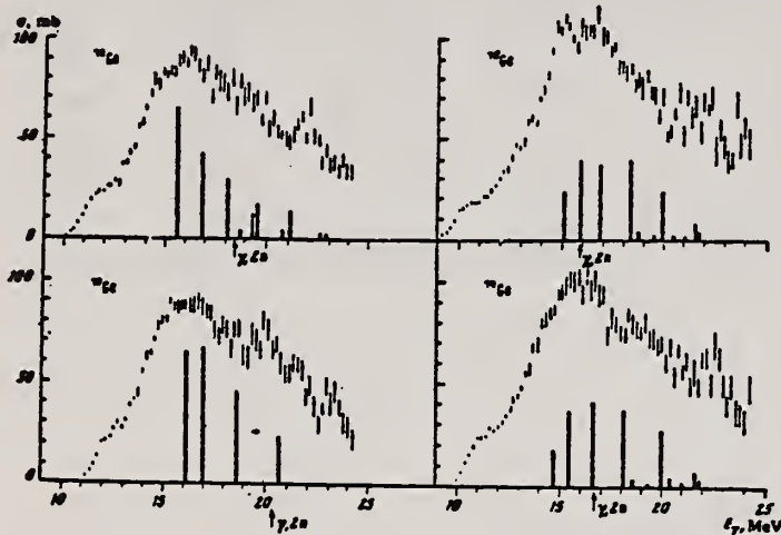
Fig. 2. The same as in Fig. 1, but for 70,72,74,76 Ge.
