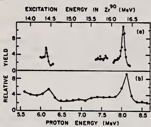
Fig. 1. Excitation function for the reaction Y^{89}(p, \gamma)Zr^{90} .
