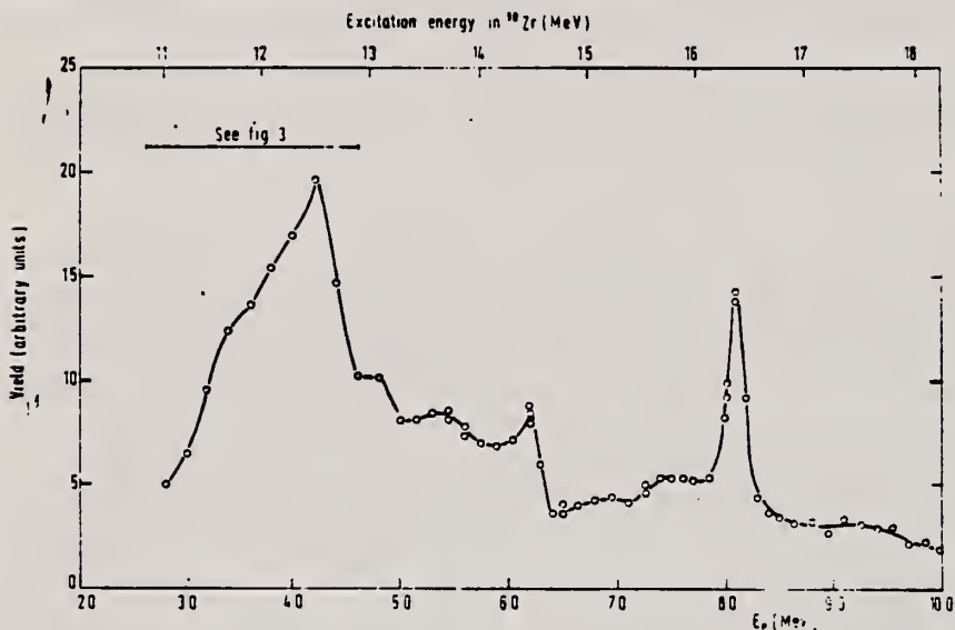
Fig. 2. The excitation function for the reaction ^{89}\text{Y}(p, \gamma)^{90}\text{Zr} measured at \theta = 90^\circ with an energy resolution of 150 to 200 keV.
