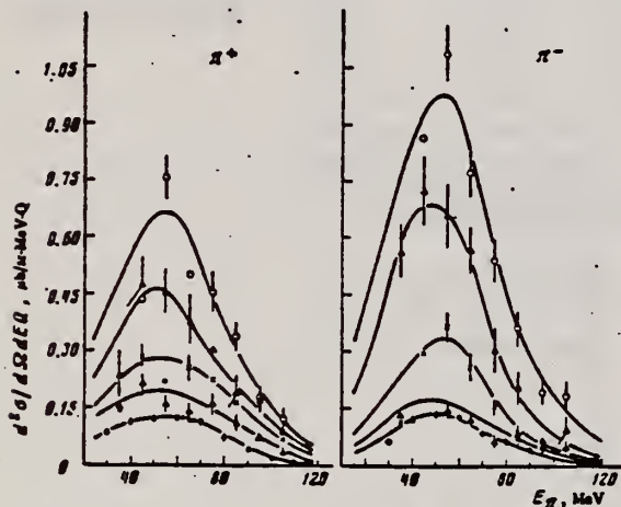
FIG. 1. Energy spectra of \pi^+ and \pi^- mesons. E_{\text{max}} = 300 MeV, \theta_{\text{lab}} = 90 \pm 7^\circ . Points: \circ - ^{12}\text{C} , \Delta - ^{28}\text{Si} , \times - ^{40}\text{Ca} , \Delta - ^{93}\text{Nb} , \circ - ^{181}\text{Ta} .
