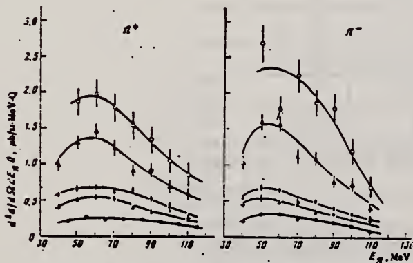
FIG. 2. Energy spectra of \pi^+ and \pi^- mesons. E_{\text{max}} = 400 MeV, \theta_{\text{lab}} = 90 \pm 7^\circ . The points are the same as in Fig. 1.
