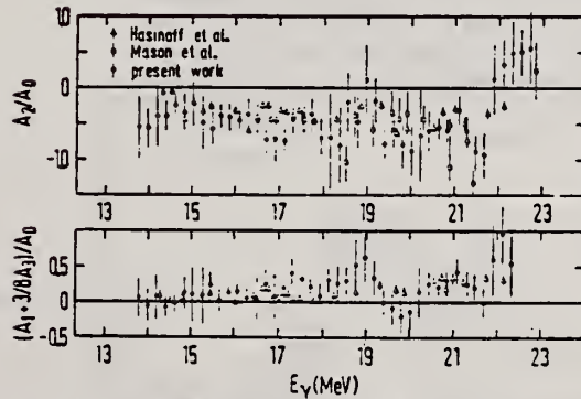
FIG. 5. A comparison of present results for the Legendre polynomial coefficients of the reaction ^{90}\text{Zr}(\gamma, p)^{89}\text{Y}_{x} with the data of Refs. 3 and 8.
