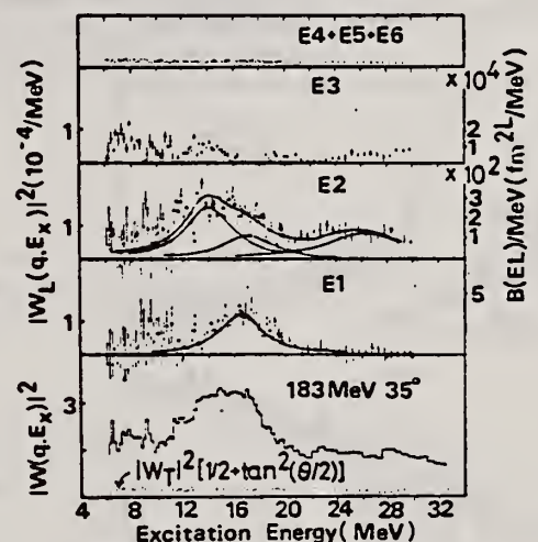
Fig. 1. Differential total form factor |W(q, E\chi)|^2 at 183 MeV 35^\circ , transverse part |W_T|^2(1/2 + \tan^2\theta/2) , and |W_L(q, E\chi)|^2 corresponding to E1, E2, E3 and E4 + E5 + E6 are shown, where |W|^2 , |W_L|^2 , and |W_T|^2 are defined in ref. [16]. The scale at the right-hand side indicates B(EL) values in units of \text{fm}^2L/\text{MeV} and at the left-hand side form factors in units of 10^{-4}/\text{MeV} .
