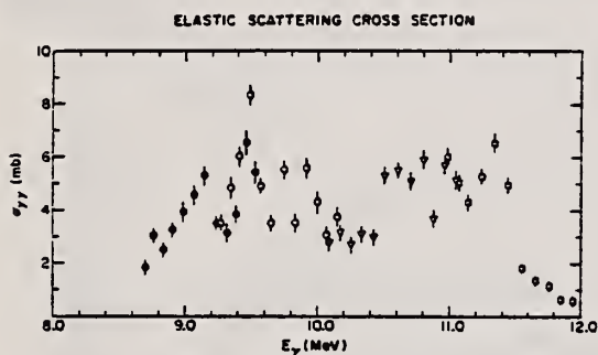
FIG. 1. The elastic scattering cross section of monochromatic photons on ^{88}\text{Sr} . The different symbols represent four sets of experimental data.
