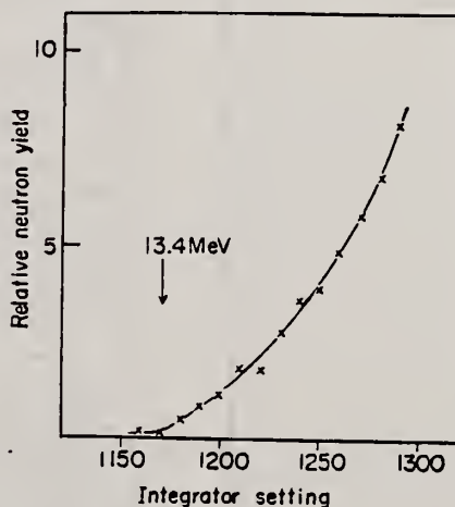
Fig. 3-2. Activation curve near threshold for Mo 92 (γ, n)Mo 91 .
