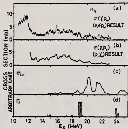
Fig. 12. Comparison of photoproton cross sections of 89 Y. (a) Present result. (b) Ref. 7). (c), (d) Theoretical estimates, refs. 13, 16) respectively.
