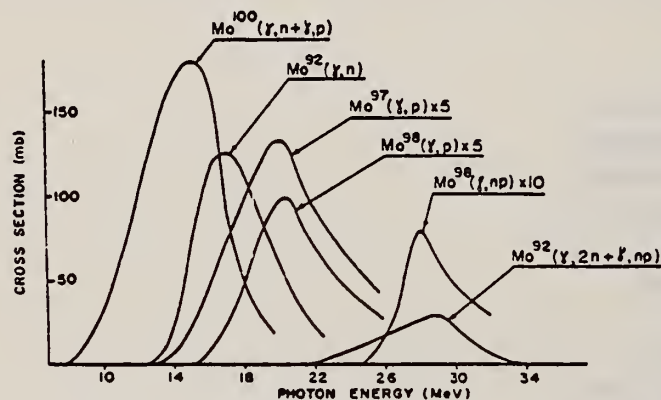
Fig. 2. Cross sections for photoreactions in molybdenum isotopes
