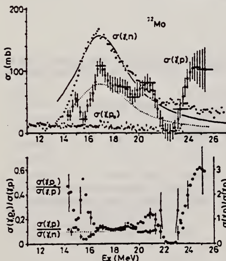
Fig. 5. Upper figure: open circles, σ(γ, p); closed circles, σ(γ, n) [ref. 18)]; closed points, σ(γ, p 0 ) [ref. 18)]; solid line, Lorentz line fit to the T < region of σ(γ, n) [ref. 18)]; dotted line, Lorentz line fit to the T < region of σ(γ, p) with Γ i and E R equal to those of σ(γ, n). Lower figure: ratio between cross sections. Dotted line: constant for σ(γ, p)/σ(γ, n) determined around T < GDR.
