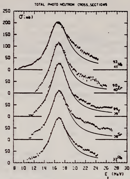
Fig. 6. Total photonutron cross sections \sigma_T of Rb, Sr, ^{89}\text{Y} , ^{90}\text{Zr} and ^{93}\text{Nb} and best one Lorentz line fit corresponding to parameters given in table I.
