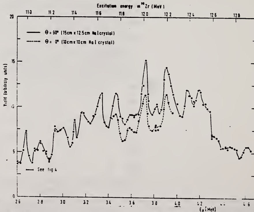
Fig. 3. The excitation functions for the reaction ^{89}\text{Y}(p, \gamma)^{90}\text{Zr} measured at \theta = 90^\circ and \theta = 0^\circ with an energy resolution of 25 keV. The curves are not normalized to one another.
