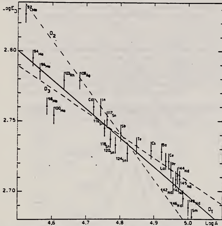
Fig. 13. Experimental results of the average energy E_D of the GDR versus the mass number A with the best fit E_D = 41.8 A^{-1/4.8} (line D_1 ). Two fits with A^{-1/3} and A^{-1/4} laws are also shown as lines D_2 and D_3 respectively.
