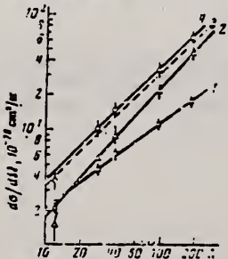
FIG. 2. Energy spectra of \pi^+ and \pi^- mesons. E_{\text{max}} = 400 MeV, \theta_{\text{lab}} = 90 \pm 7^\circ . The points are the same as in Fig. 1.
