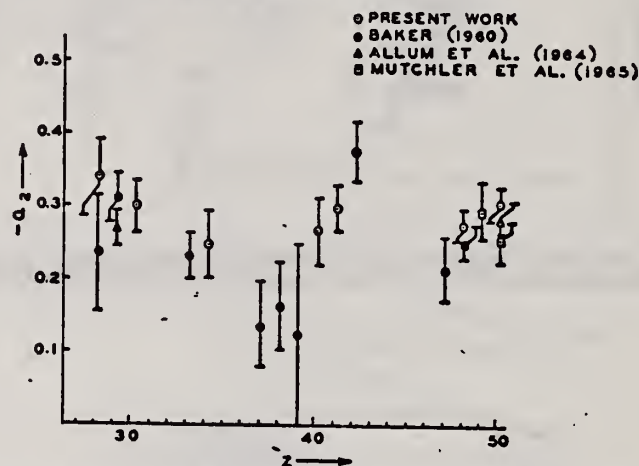
FIG. 2. The anisotropy coefficients a 1 , in the formula W(θ) = a 0 (1 + a 1 P 1 + a 2 P 2 ), obtained in the present work, and those obtained by other workers in the same part of the Periodic Table.
