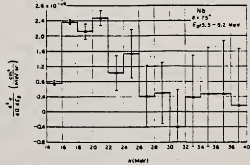
Fig. 17. Differential cross section for producing protons from Nb as a function of photon energy. The histogram was drawn by a photon-difference analysis of fig. 14.
