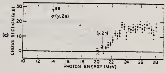
FIG. 8 (a) Total photoneutron cross section \sigma[(\gamma,n) + (\gamma,pn) + (\gamma,2n)] for Y 89 . The solid curve is a Lorentz-line fit to the giant-resonance data (14 to 19 MeV). The thresholds (arrows), except when otherwise noted, are from Ref. 10. In this case, the (\gamma,2n) threshold is taken from the data. (b) Single photoneutron cross section \sigma[(\gamma,n) + (\gamma,pn)] for Y 89 . The dashed line represents the maximum possible systematic error owing to the uncertainty in the normalization constant for the bremsstrahlung subtraction (see text). (c) The (\gamma,2n) cross section for Y 89 . The threshold determination of 20.8 \pm 0.1 MeV determines the mass of Y 87 (see text). The threshold value is taken from the data. The cross-section scale has been doubled for clarity.
