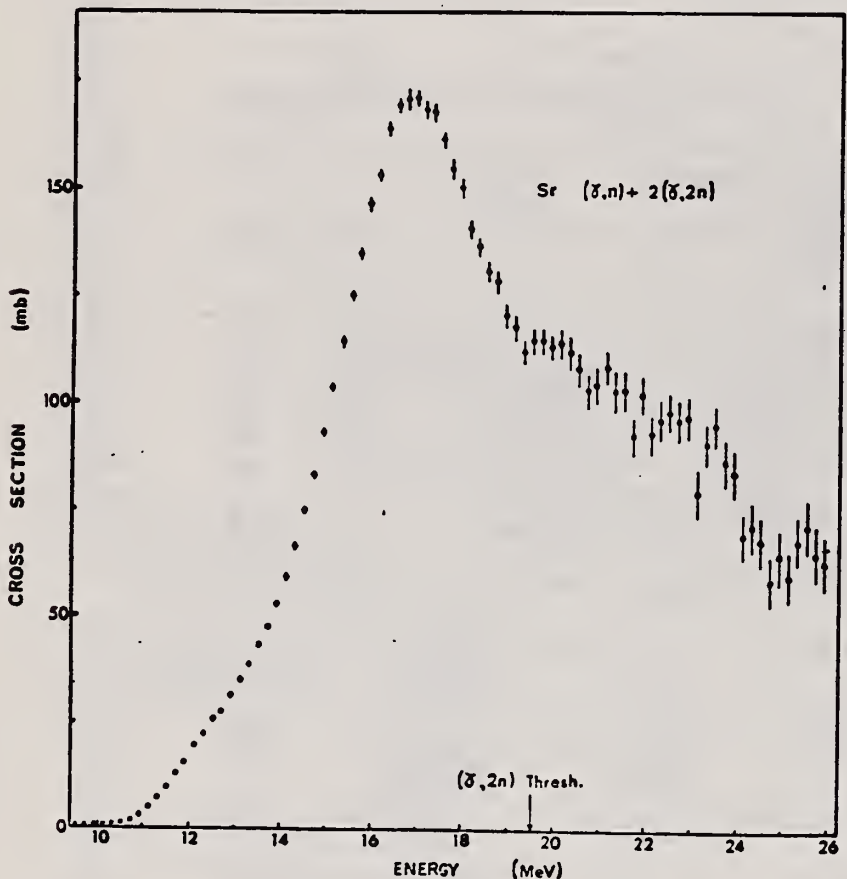
Fig. 1. The [Sr(\gamma, n) \rightarrow 2Sr(\gamma, 2n)] cross section obtained by analysis of the yield curve using three interleaving second difference calculations. The resolution applied is 1.08 MeV.
