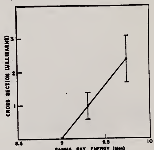
FIG. 6. Cross section vs energy Nb 92 ( \gamma, n )Nb 92 (10 day). The line indicates a possible extrapolation to threshold.
