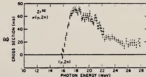
FIG. 11. (a) Total photoneutron cross section for Zr^{92} . (b) Single photoneutron cross section for Zr^{92} . (c) The (\gamma,2n) cross section for Zr^{92} .
