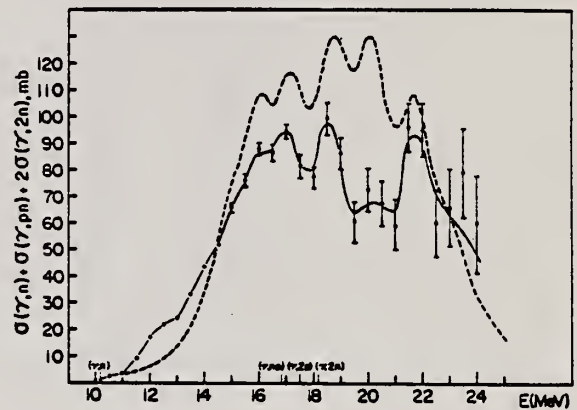
FIG. 1. Solid line: photoneutron production cross section of \text{As}^{75} ; dashed line: total photoabsorption cross section.
