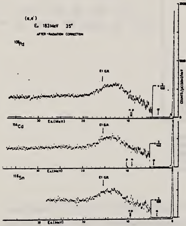
Fig. 6. Spectra of ^{116}\text{Sn} , ^{114}\text{Cd} and ^{106}\text{Pb} obtained at 183 MeV and 35^\circ .
