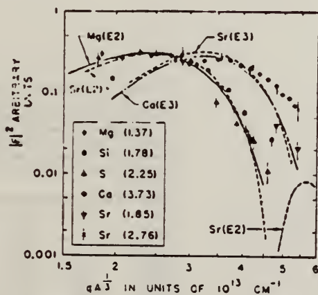
FIG. 7. Inelastic "universal curves." A composite plot of inelastic data from Mg, Si, S, Ca, and Sr against q \Delta \frac{1}{2} . The various form factors are arbitrarily normalized to minimize the spread of points. The point from sulfur and the point from silicon which seem to deviate from the "universal curve" are assumed to contain undetected experimental errors. The curves labeled Mg(E2), Sr(E2), Ca(E3), and Sr(E3) are calculated for electric-quadrupole and -octupole transitions using the "smeared \delta -function" transition charge densities of Sec. V, and are arbitrarily normalized.
