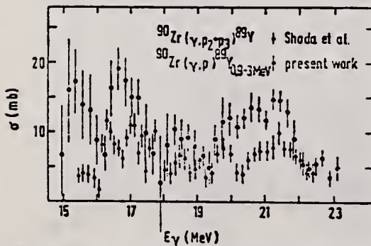
FIG. 8. A comparison of present results for the ^{90}\text{Zr}(\gamma, p)^{89}\text{Y}_{0-3} cross section with the data of Shoda et al. (Ref. 4).
