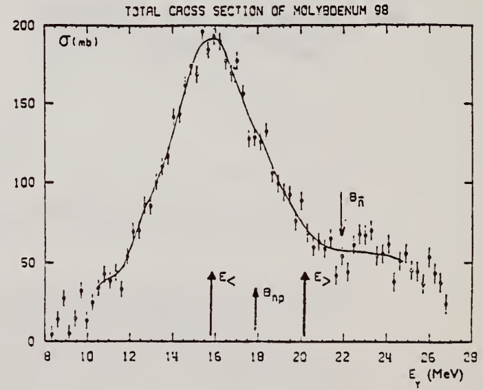
Fig. 10. Same as fig. 7, for 98 Mo.
