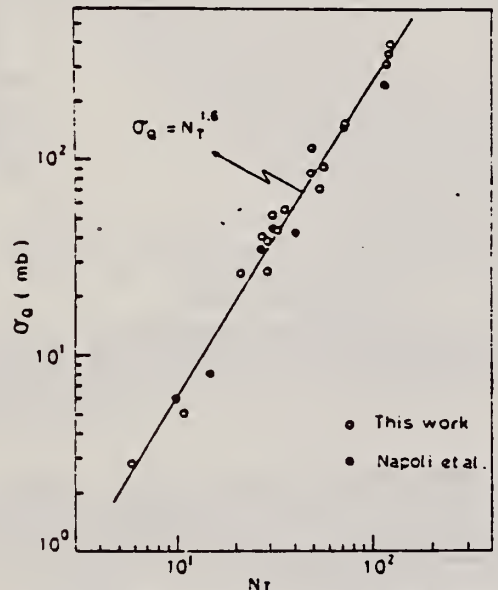
Fig. 2. Yield per equivalent quanta versus target neutron number.
