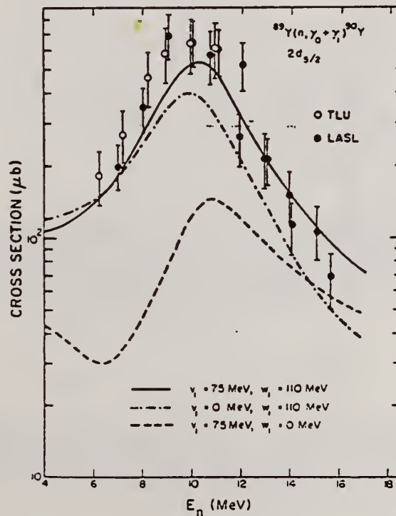
Fig. 5. Detailed comparison of the experimental (n, \gamma ) cross sections for \gamma -ray transitions to the ground-state doublet of ^{90}\text{Y} . The data are compared to the predictions of the DSD model using various particle-vibration interaction functions.
