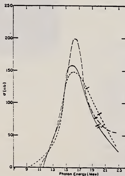
FIG. 2. Cross sections for the (\gamma, n) reactions in strontium isotopes. Full curve Sr^{88} , short dashes Sr^{87} , long dashes Sr^{86} . The single and double slash marks on each curve represent the locations of the (\gamma, pn) and (\gamma, 2n) thresholds, respectively. The units of the ordinate are 10^{-27} \text{ cm}^2 .
