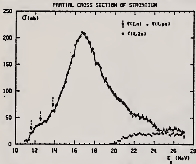
Fig. 2. Partial photonuclear cross sections \sigma(\gamma, n) and \sigma(\gamma, 2n) of Sr.
