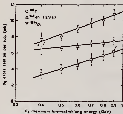
FIG. 7. - Behaviour of cross sections per equivalent quantum \sigma_q , as a function of \log_{10} E_0 (maximum bremsstrahlung energy) for reactions ^{102}\text{Rh}(\gamma, n)^{102}\text{Rh}(t, 2.9 y) , ^{102}\text{Rh}(\gamma, 2n)^{101}\text{Rh} and ^{88}\text{Y}(\gamma, 6p 9n)^{88}\text{Y} . The straight lines through the experimental points were obtained by using the least-squares method
