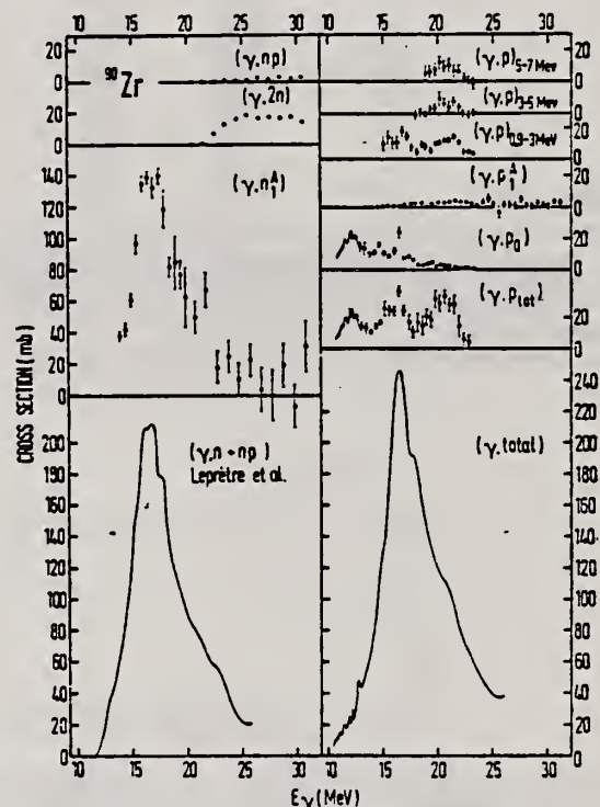
FIG. 14. Cross sections integrated over angles for processes studied in the present work (data points) are displayed with the exception of the total photon-neutron cross section (solid curve in the bottom left corner of the diagram) for which the results of Leprêtre et al. (Ref. 6) are shown. The low-energy parts of the ground state and total photoproton cross sections are taken from Ref. 3 (solid curves). In the bottom right corner the sum of the total photoproton, the (\gamma, 2n) cross sections from the present experiment and (\gamma, n + np) cross section of Ref. 6, is displayed. It represents to a good accuracy the total photoabsorption cross section.
