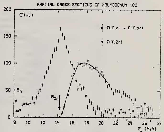
Fig. 5. Same as fig. 1, for ^{100}\text{Mo} .
