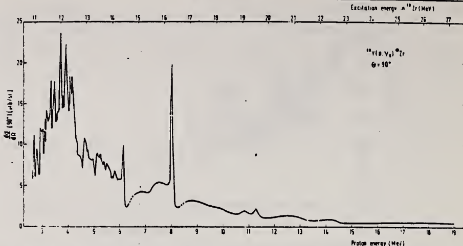
Fig. 9. Combined lower and higher energy excitation functions at \theta = 90^\circ with inclusion of some data from refs. 6, 10 . The cross section is normalized to the values given in the text. For the energy regions E_p = 6.5-7.8 MeV and E_p = 8.6-9 MeV, the data from the 150 keV excitation function (fig. 2) were used.
