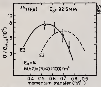
FIG. 8. Relative DWBA cross section, calculated using the Goldhaber-Teller model, as fitted to the experimental cross sections for the resonance at 14 MeV with a width of \Gamma=4.5 MeV. The comparison rules out any assignment other than E2.
