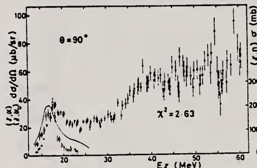
FIG. 6. Photoalpha differential cross section of 90 Zr (closed points) analyzed from the (e,α) cross section in Fig. 5 and 90 Zr(γ,α 0 ) differential cross section (open circles), at θ=90°. E1 interaction only was considered in these analyses. The value of χ 2 for the total (γ,α) cross section was calculated for the cross section smoothed by eye. Solid line shows 90 Zr(γ,α) cross section.
