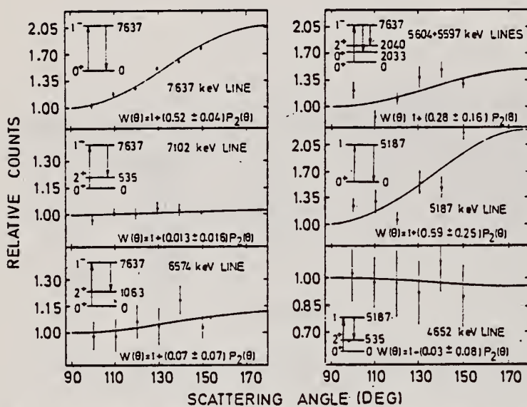
Fig. 3. Angular distributions of the elastic and some inelastic transitions de-exciting the 7637 keV level in ^{100}\text{Mo} as measured using a 20\text{ cm}^3 Ge(Li) detector. The solid lines have the form W(\theta) = 1 + AP_2(\cos \theta) and are least square fits to the experimental distributions. In each case the corresponding \gamma\gamma cascade is indicated.
