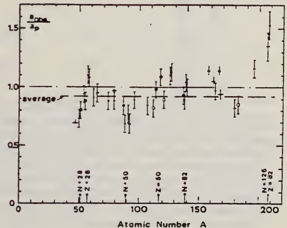
Fig. 15. Ratio a_{obs}/a_p versus atomic number A . Here a_{obs} is the level density parameter taken from the neutron resonance work of refs. 1-2, and a_p is the level density parameter derived from the present (\gamma, n) work. Filled circles represent points where nuclei in the neutron resonance and in the (\gamma, n) experiment were the same. Open circles represent points where the respective nuclei were approximately matched. Triangles represent points which are based on measurement of neutron mean energies at two bremsstrahlung energies only.
