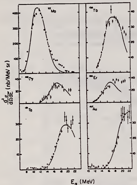
FIG. 2. The α-particle energy spectra at 50° in the laboratory for the four new nuclei studied as well as for two nuclei in which additional data have been obtained. The solid curves are the evaporation model fits described in text.
