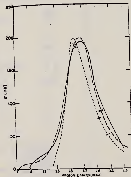
FIG. 5. Cross sections for the (γ, n) reactions in zirconium isotopes. Short dashes Zr 20 , long dashes Zr 21 , full curve Zr 22 . The previously published Zr 40 and Zr 21 results have been recomputed, taking into account the present Zr 22 measurements. The single and double slash marks on each curve represent the locations of the (γ, p)n and (γ, 2n) thresholds respectively. The units of the ordinate are 10 -27 cm 2 .
