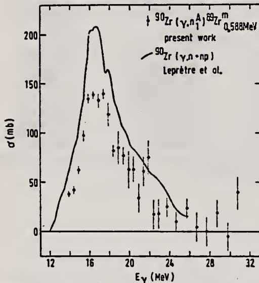
FIG. 12. The (\gamma, n_1^+) cross section represented by data points contains, in addition to the ^{90}\text{Zr}(\gamma, n_1^+)^{89}\text{Zr}_{0.588} contribution, also contributions of all photon-neutron cross sections involving those residual ^{89}\text{Zr} states which subsequently decay to the first-excited state. For comparison the (\gamma, n + np) data of Leprêtre et al. (Ref. 6) (continuous curve) are also shown.
