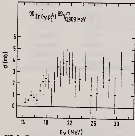
FIG. 7. The summed cross section (\gamma, p_1^A) for the ^{90}\text{Zr}(\gamma, p) reactions leading to the 0.909 MeV first-excited isomeric state of ^{89}\text{Y} . The cross section is obtained from a Penfold-Leiss analysis of the 0.909 MeV \gamma -ray activation yield. Here, besides the direct (\gamma, p_1) cross section, also contributions from states decaying to the 0.909 MeV state are contained. In particular, \sigma(\gamma, p_1^A) incorporates \sigma(\gamma, p_{s+6+\gamma+p}) and 70% of \sigma(\gamma, p_1) , involving ^{89}\text{Y} states at 2.529, 2.568, 2.622, 2.871, and 2.220 MeV, respectively.
