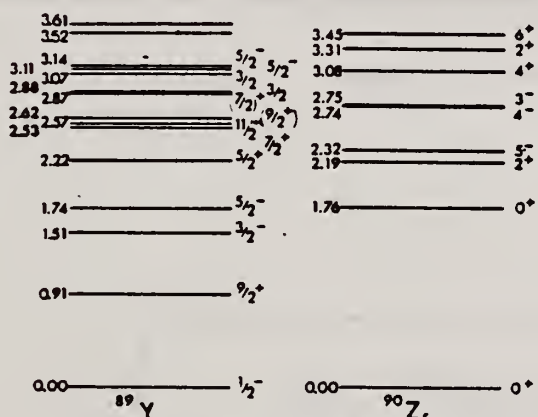
FIG. 1. Presently accepted level schemes for ^{89}\text{Y} and ^{90}\text{Zr} taken from the data of Van Patter (Ref. 8) and Ball (Ref. 9), respectively.
