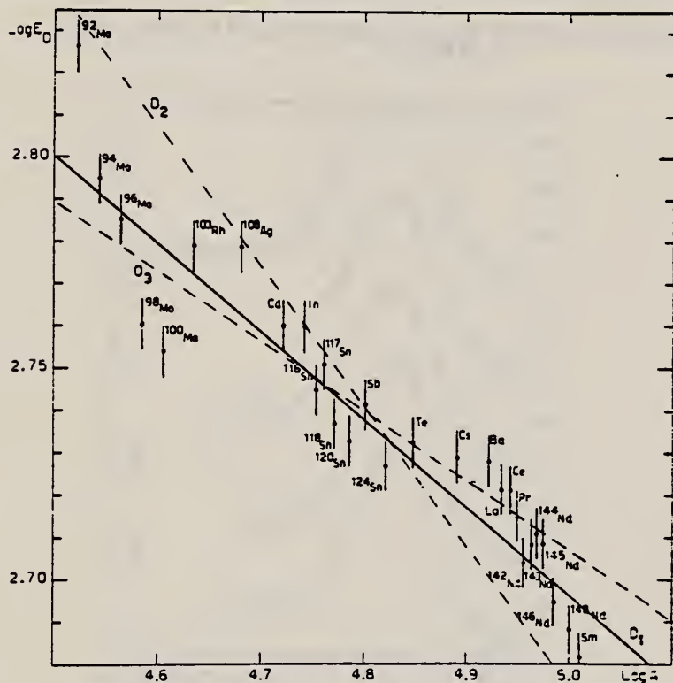
Fig. 13. Experimental results of the average energy E_D of the GDR versus the mass number A with the best fit E_D = 41.8 A^{-1/4.8} (line D_1 ). Two fits with A^{-1/2} and A^{-1/4} laws are also shown as lines D_2 and D_3 respectively.
