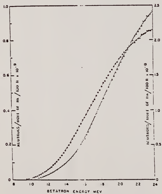
FIG. 1. Photon-neutron yield versus betatron energy. ○ manganese; □ rhodium.
