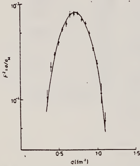
Figure 5. 3_1^- form factor. The full curve is the best fit assuming the level to be a single octupole phonon vibration.
