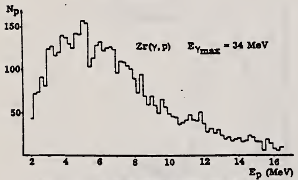
Fig. 3c. Energy distribution of photoprotons at E_{\gamma\max} = 34 MeV.
