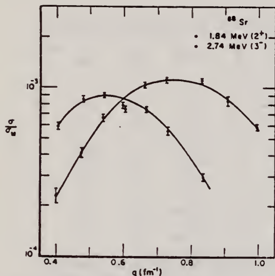
FIG. 5. Tassie-model fits to 88 Sr 2 + and 3 - form factors.
