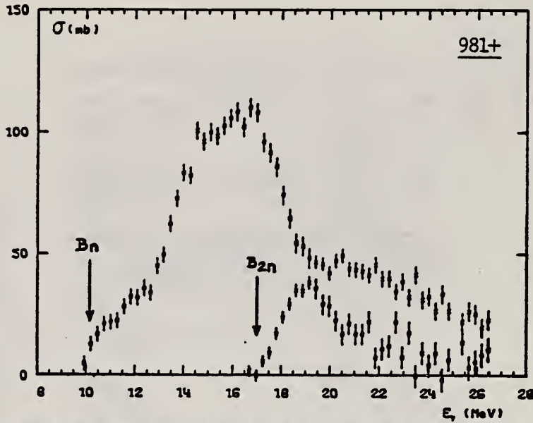
Fig. 5. Partial photoneutron cross sections [ \sigma(\gamma, n) + \sigma(\gamma, pn) ] and \sigma(\gamma, 2n) for ^{76}\text{Ge} . Arrows B_n and B_{2n} indicate theoretical threshold values for (\gamma, n) and (\gamma, 2n) reactions respectively.
