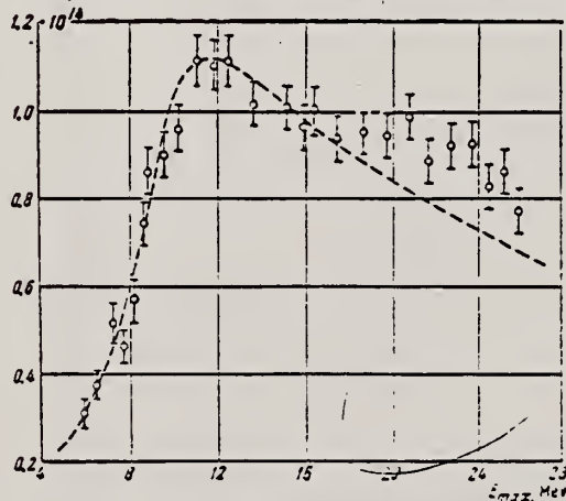
FIG. 1. Yield of the reaction Rh 103 (γ,γ 1 )Rh 103m at various maximum x-ray energies E max . Ordinates — saturated activity per second per mole per ampere of ionization current of the absolute chamber. The dashed curve is the yield curve calculated under the assumption that the reaction cross section is zero at energies above 12.5 Mev.
