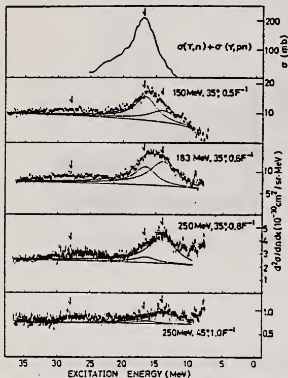
FIG 1. Spectra of photoreaction and electron scattering in ^{90}\text{Zr} . The arrows indicate the positions of the 14.0-, 16.65-, and 28-MeV peaks.
