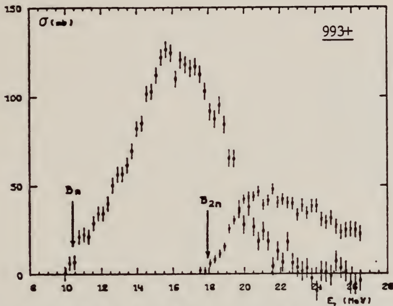
Fig. 9. Partial photoneutron cross sections [ \sigma(\gamma, n) + \sigma(\gamma, pn) ] and \sigma(\gamma, 2n) for ^{78}\text{Se} . Arrows B_n and B_{2n} indicate theoretical threshold values for (\gamma, n) and (\gamma, 2n) reactions respectively.
