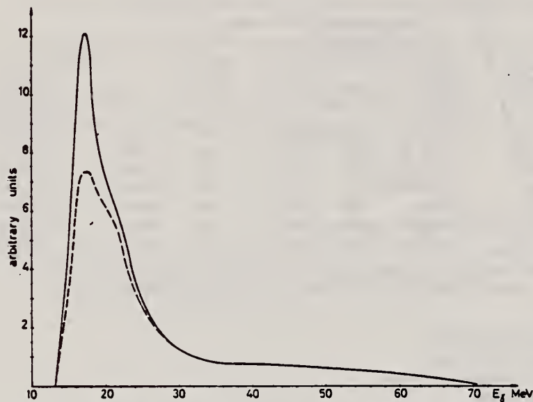
Fig. 3. ( \gamma, n ) reaction in ^{98}\text{Mo} , total (solid line) and \frac{1}{2}^- state (dashed line) cross sections.
