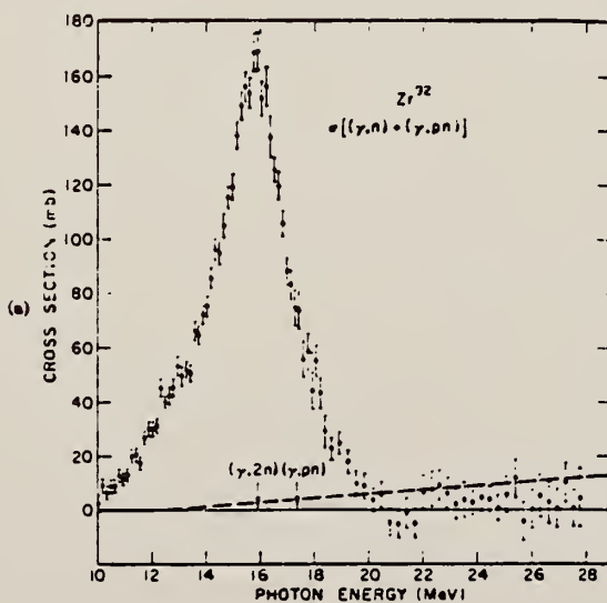
FIG. 11. (a) Total photoneutron cross section for Zr^{92} . (b) Single photoneutron cross section for Zr^{92} . (c) The (\gamma,2n) cross section for Zr^{92} .
