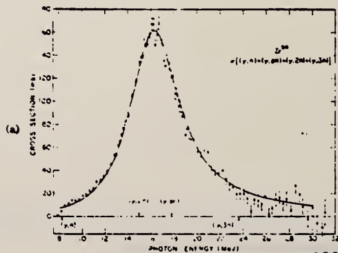
FIG. 12. (a) Total photoneutron cross section \sigma[(\gamma, n) + (\gamma, pn) + (\gamma, 2n) + (\gamma, 3n)] for Zr 94 . (b) Single photoneutron cross section for Zr 94 . (c) The (\gamma, 2n) cross section for Zr 94 . (d) The (\gamma, 3n) cross section for Zr 94 .
