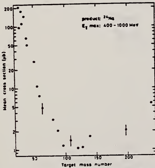
Fig. 2. The mean cross section in the energy range 400 to 1000 MeV calculated from the yields of Figure 1 in this work and of Figures 1 to 6 in [1]. This error is given by bars in some points
