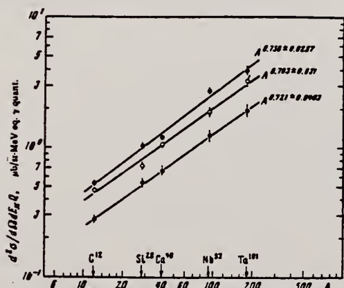
FIG. 4. Charged pion yield vs. the mass number of the nucleus: ●— E_\pi = 105 \pm 10 MeV, ○— E_\pi = 85 \pm 10 MeV, ●— E_\pi = 65 \pm 10 MeV.
