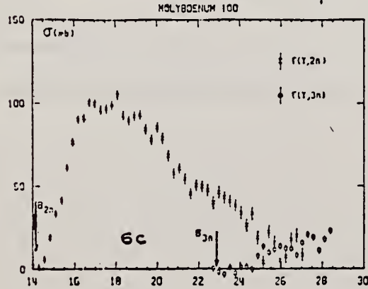
Fig. 6. Partial photonuclear cross sections \sigma(\gamma, 2n) and \sigma(\gamma, 3n) of ^{96}\text{Mo} , ^{98}\text{Mo} and ^{100}\text{Mo} . Arrows indicate theoretical threshold values given in table 2.
