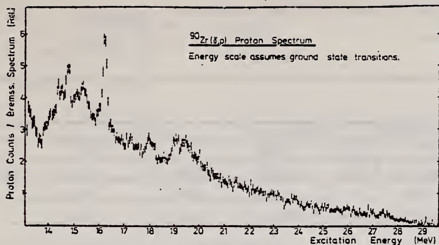
Fig. 2. The ^{90}\text{Zr}(\gamma, p) proton spectrum.
