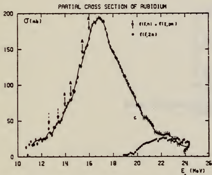
Fig. 1. Partial photoneutron cross sections \sigma(E, n) and \sigma(E, 2n) of Rb.
