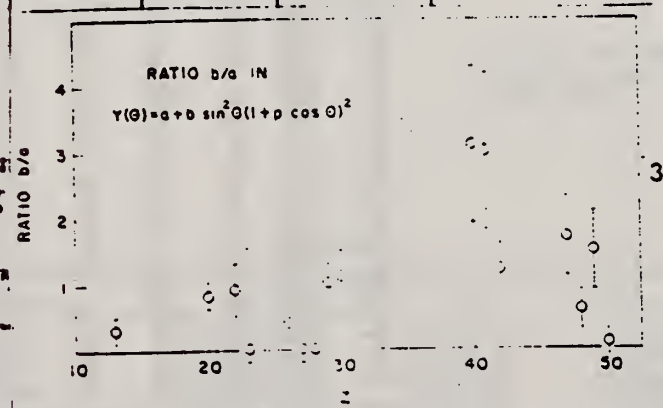
FIG. 2. The yields of fast photoprotons ( E_p > 8 MeV) obtained from targets of various elements when irradiated with 22 MeV bremsstrahlung. The target thicknesses range from 251 to 372 μg and about 8 MeV for protons. The errors noted are statistical. FIG. 3. The anisotropy coefficient b/a for fast photoprotons ( E_p > 8 MeV) from dielements. The errors noted are statistical.
