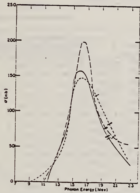
FIG. 2. Cross sections for the (γ, n) reactions in strontium isotopes. Full curve Sr 86 , short dashes Sr 87 , long dashes Sr 88 . The single and double slash marks on each curve represent the locations of the (γ, pπ) and (γ, 2n) thresholds, respectively. The units of the ordinate are 10 -27 cm 2 .
