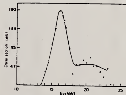
Fig. 5-2. Cross section curve for Mo 92 (γ, n)Mo 91 .
