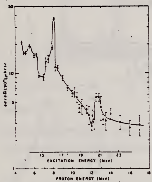
FIG. 1. Differential cross section of process ^{89}\text{Y}(p, \gamma_0)^{89}\text{Zr} at 90^\circ . The errors shown are statistical. Because of some uncertainty in the gamma-detector efficiency, absolute values are good probably to within 35%.
