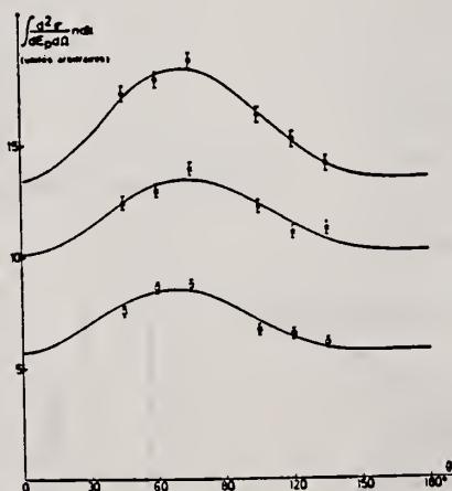
FIG. 3. — Distributions angulaires. E_0 = 40 MeV. \times E_p = 5.05 - 6.55 MeV; + 0.28 \sin^2 \theta (1 + 0.80 \cos \theta) . \circ E_p = 5.75 - 7.15 MeV; + 0.31 \sin^2 \theta (1 + 0.99 \cos \theta) . \square E_p = 7.05 - 9.45 MeV; + 0.37 \sin^2 \theta (1 + 1.29 \cos \theta) .
