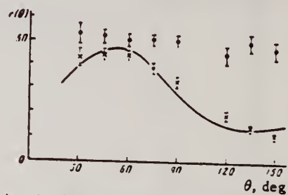
FIG. 6. Angular distributions of photoprotons from Rh for E γmax = 33.5 MeV. ● - E p = 3.25-9.25 MeV; × - E p > 9.25 MeV.
