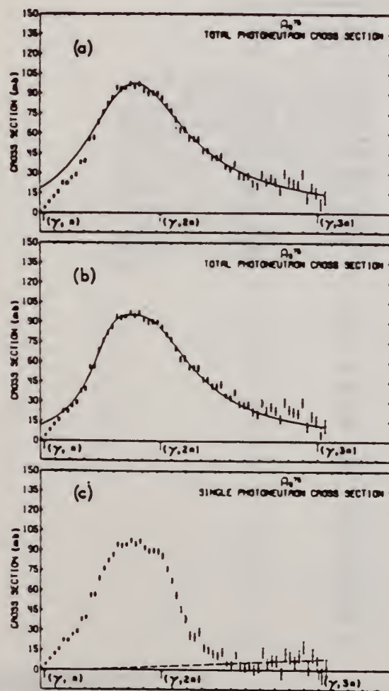
FIG. 5. Photoneutron cross sections for As 75 . (a) Total photoneutron cross section \sigma[(\gamma, n) + (\gamma, pn) + (\gamma, 2n)] . The solid line is a single-component Lorentz-curve fit to the giant-resonance data (13.6 to 21.3 MeV). (b) Total photoneutron cross section, repeated. The solid line is a two-component Lorentz-curve fit to the giant-resonance data. (c) Single photoneutron cross section \sigma[(\gamma, n) + (\gamma, pn)] . The dashed line represents the maximum systematic error owing to the uncertainty in the normalization of the positron bremsstrahlung subtraction. (d) Double photoneutron cross section \sigma(\gamma, 2n) .
