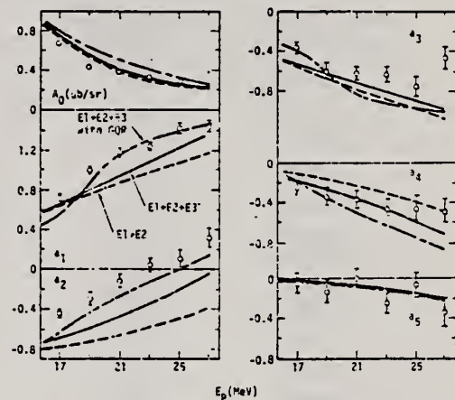
FIG. 2. Angular distribution coefficients extracted from LLL data. See text and Fig. 1 caption for significance of curves.
