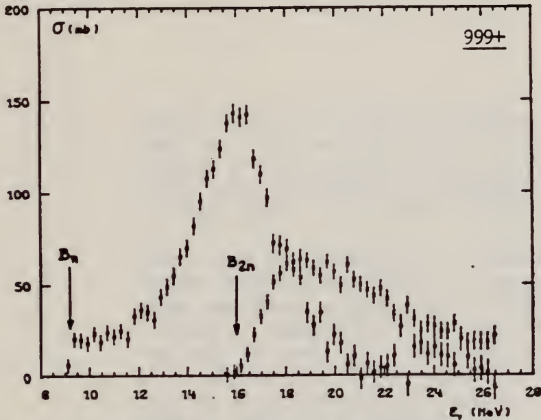
Fig. 11. Partial photoneutron cross sections [ \sigma(\gamma, n) + \sigma(\gamma, pn) ] and \sigma(\gamma, 2n) for ^{82}\text{Se} . Arrows B_n and B_{2n} indicate theoretical threshold values for (\gamma, n) and (\gamma, 2n) reactions respectively. Data were not corrected for impurities.
