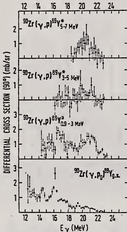
FIG. 3. Differential 90° cross section for the (\gamma, p_0) reaction and differential summed cross sections for reactions involving various regions of excitations in the residual nucleus ^{89}\text{Y} .
