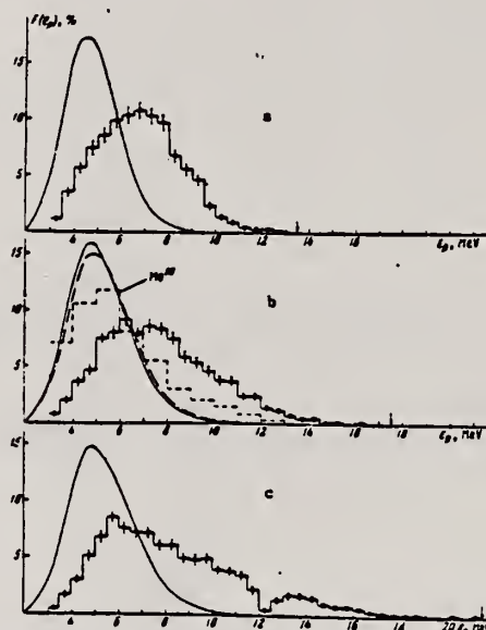
FIG. 2. Energy distributions of photoprotons from Nb^{93} for E_{\gamma,max} = 19.5 MeV (a), 23.5 MeV (b), and 27.5 MeV (c). The histograms are the experimental spectra. The dashed histogram in Fig. 2b is the photoproton spectrum of Mo^{93} . [1] The smooth curves are spectra computed from the evaporation model for level density \omega , taking account of pair correlations. The dashed curve in Fig. 2b is the same, neglecting pair correlations. Arrows indicate the maximum possible proton energy E_{p,max} = E_{\gamma,max} - B_p .
