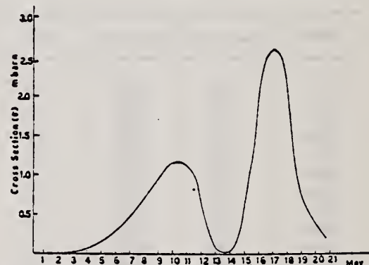
FIG. 2. Cross section as a function of energy for formation of the isomeric state of Y^{89} .
