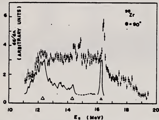
Fig. 1. Photoproton cross section for ^{90}\text{Zr} calculated from the energy distribution of the E_e = 20.0 MeV bombardment. The scale was constructed under the assumption that observed protons correspond to ground-state transitions. The triangles show the energy resolution. The solid curve is the (\gamma, p\eta) cross section calculated from the (p, \gamma) data.
