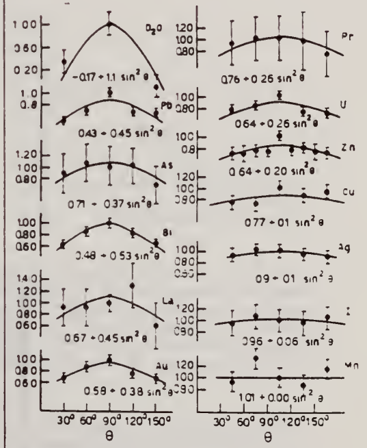
Figure 4: Angular distributions of fast photoneutron as observed with the Si 28 (n,p)Al 28 detector. Data normalized at 90° in each case.
