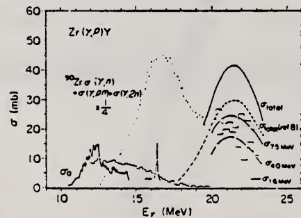
Fig. 11. Cross sections for strong photoproton transitions on Zr. Photoproton cross section obtained from the yield curve, 9) neutron emission cross section 10) and the results of the ^{90}\text{Y}(\gamma, p_0)^{90}\text{Zr} reaction 4, 5, 11, 12) are also shown.
