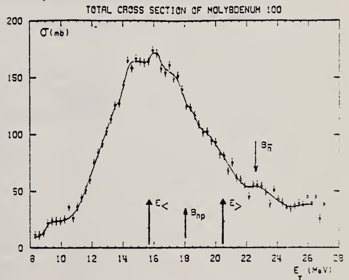
Fig. 11. Same as fig. 7, for ^{100}\text{Mo} .
