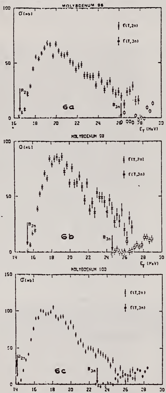
Fig. 6. Partial photoneutron cross sections \sigma(\gamma, 2n) and \sigma(\gamma, 3n) of 96 Mo, 98 Mo and 100 Mo. Arrows indicate theoretical threshold values given in table 2.
