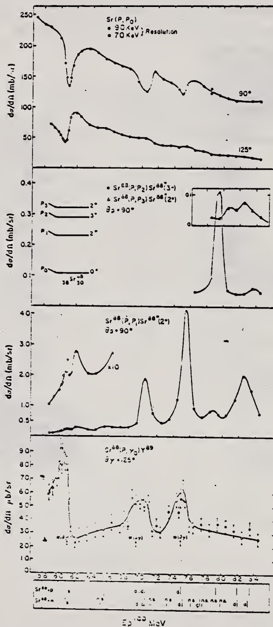
Fig. 3. Excitation curves for several exit channels taken simultaneously. Upper two curves elastic proton scattering from Sr at 90° and 125°. Inset at far right excitation curve for the reaction ^{86}\text{Sr}(p, p_2) at 90°. Curve labeled p_3 excitation curve for the ^{86}\text{Sr}(p, p_3) reaction at 90°. Note the striking resonance at 7.92 MeV. Curves labeled p_1 excitation curve for the ^{86}\text{Sr}(p, p_1) reaction at 90°. Bottom curve excitation curve for the ^{86}\text{Sr}(p, \gamma) reaction at 125°. Underlying box upper set of levels: resonance energies (lab) in ^{86}\text{Sr}+p reaction. The energy scale was set to agree with that of ref. 14). Lower set of levels from ref. 9) arbitrarily matched at 7.0 MeV and with energy intervals stretched by 39/88 to convert to "equivalent" lab energy. Levels shown with half the usual length are non-stripping levels.
