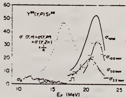
Fig. 10. Cross sections for strong photoproton transitions on ^{89}\text{Y} . The neutron emission cross section (9) and the result of the ^{88}\text{Sr}(p, \gamma)^{89}\text{Y} reaction (9) are also shown.
