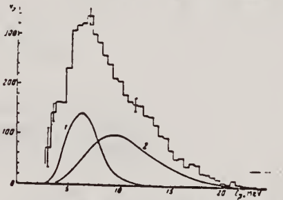
FIG. 2. Energy distribution of 5222 photoprotons from Rh for E γmax = 33.5 MeV. Same notation as in Fig. 1.
