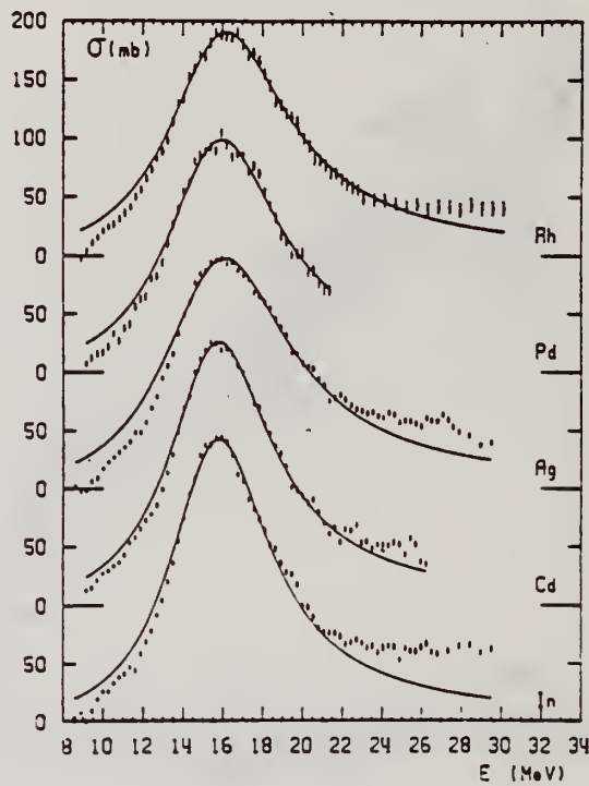
Fig. 8. Best single Lorentz line fit to \sigma_{tot}(\gamma) = \sigma(\gamma, n) + \sigma(\gamma, np) + \sigma(\gamma, 2n) for ^{49}\text{Rh} , ^{46}\text{Pd} , ^{47}\text{Ag} , ^{48}\text{Cd} and ^{49}\text{In} .
