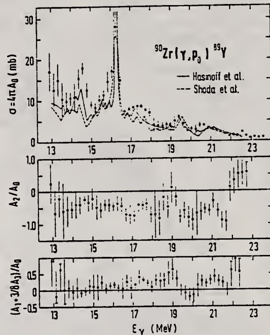
FIG. 4. Legendre polynomial coefficients for the angular distributions of protons in the reaction ^{90}\text{Zr}(\gamma, p_0)^{89}\text{Y} obtained from differential cross sections for the angles 30°, 90°, and 150° assuming an angular dependence of the form W(\theta) = \sum_{l=0}^3 A_l P_l(\cos\theta) . Cross sections for particular angles were determined from measured spectra by means of a least-squares-fit analysis (Ref. 13). On the top diagram present results for \sigma = 4\pi A_0 (data points) are compared to the data of Refs. 11 and 8.
