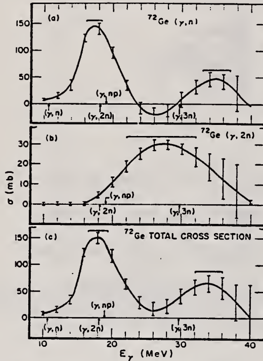
FIG. 5. The \sigma(\gamma, n) cross section for ^{72}\text{Ge} . (b) The \sigma(\gamma, 2n) cross section for ^{72}\text{Ge} . (c) The total cross section \sigma(\gamma, n) + \sigma(\gamma, 2n) + \sigma(\gamma, np) + \sigma(\gamma, p) for ^{72}\text{Ge} .
