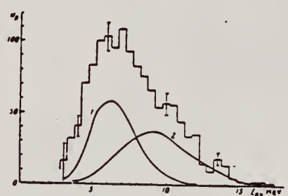
FIG. 1. Energy distribution of 1287 photoprotons from Rh for E γmax = 22.5 MeV. Calculated spectra: curve 1 for evaporation; curve 2 for protons from the direct photoeffect.
