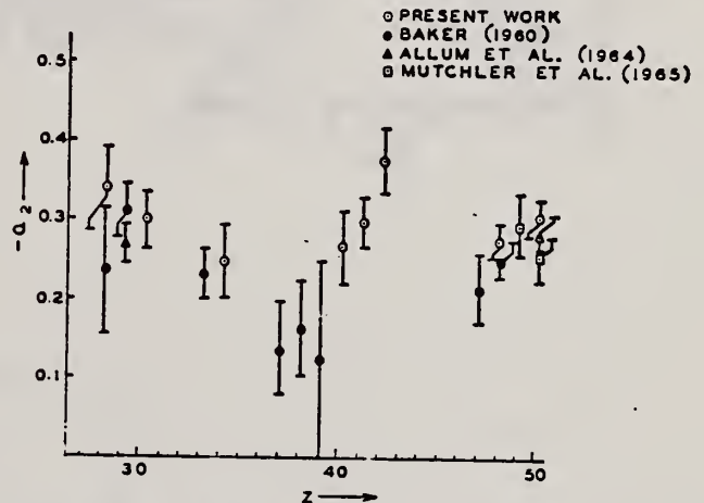
FIG. 2. The anisotropy coefficients a_2 , in the formula W(\theta) = a_0(1 + a_1P_1 + a_2P_2) , obtained in the present work, and those obtained by other workers in the same part of the Periodic Table.
