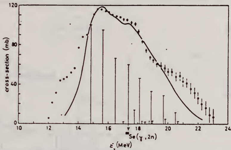
Fig. 1. - Corrected (\gamma, 2n) cross-section for ^{76}\text{Se} . The dipole strengths, calculated for ^{76}\text{Se} , are indicated by the vertical bars.
