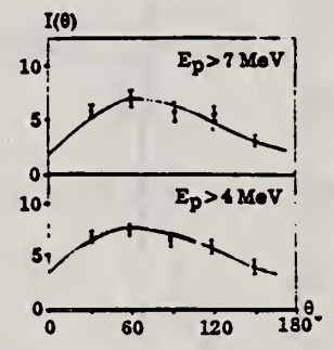
Fig. 4. Angular distributions of photoprotons at E_{\gamma\max} = 25 MeV.
