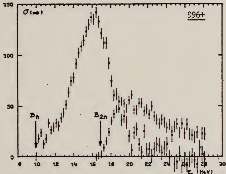
Fig. 10. Partial photoneutron cross section [\sigma(\gamma, n) + \sigma(\gamma, pn)] and \sigma(\gamma, 2n) for ^{80}\text{Se} . Arrows B_n and B_{2n} indicate theoretical threshold values for (\gamma, n) and (\gamma, 2n) reactions respectively.
