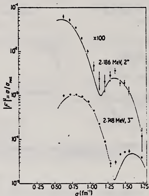
Figure 3. A comparison of the high momentum transfer data of Phan-Xuan-Ho et al (1973) with the extrapolation of the fits obtained in the present experiment to 209 MeV. The parameters of the fit are presented in table 3.
