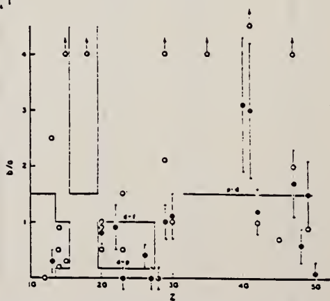
Fig. 4. The values of the fast photoproton anisotropy coefficient b/a found by the present authors (●) and other workers (○) in the region of the periodic table 10 < Z < 50 . Arrows indicate outside points. The references to the results of other workers are given in Table II. The denunciations are explained in the text.
