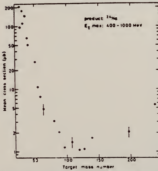
Fig. 2. The mean cross section in the energy range 400 to 1000 MeV calculated from the yields of Figure 1 in this work and of Figures 1 and 2 in [1]. The errors given in [1] are in some points
