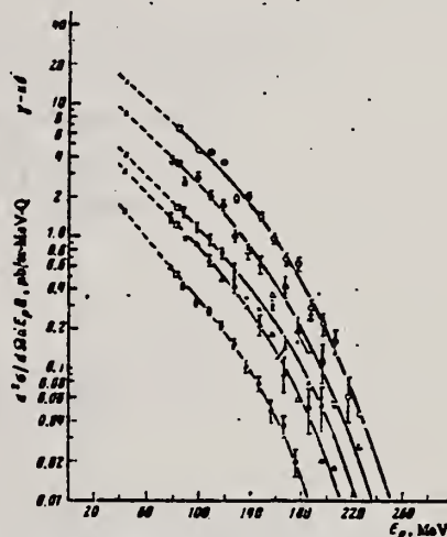
FIG. 3. Energy spectra of protons, E_{\text{max}} = 300 MeV, \theta_{\text{lab}} = 90 \pm 7^\circ . Points: \circ - ^{12}\text{C} , \Delta - ^{28}\text{Si} , \times - ^{40}\text{Ca} , \Delta - ^{93}\text{Nb} , \circ - ^{181}\text{Ta} . \square -data from ref. 5, \bullet -data from ref. 6.
