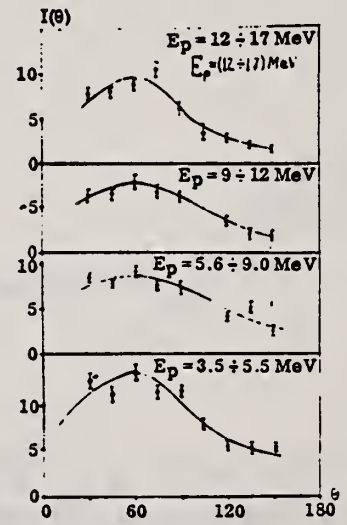
Fig. 5. Angular distributions of photoproton at E_{\gamma\max} = 34 MeV.
