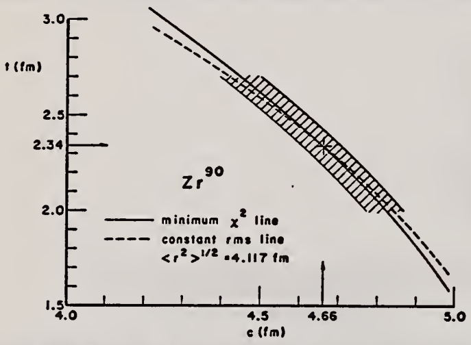
Fig. 2. Values of half-density radius c and skin thickness t consistent with the experimental results lie within the cross-hatched area. The solid line locates the best fit (minimum \chi^2 ), and the dashed line corresponds to a fixed rms radius of 4.12 fm.
