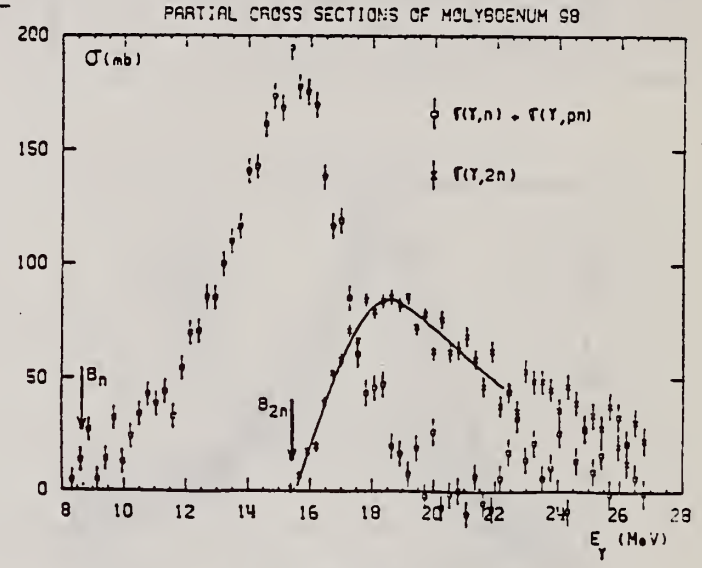
Fig. 4. Same as fig. 1, for 98 Mo.
