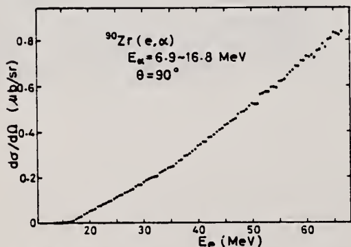
FIG. 5. Differential cross section of the (e, α) reaction at θ=90°.
