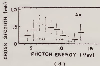
Fig. 2. The elastic scattering cross sections for Mg, Fe, Zn, As, Cd, Sb and Bi. The indicated spread in energy is the width of the sum-up channels, and the vertical lines are the statistical errors including background counts. The arrows represent the positions of the threshold energies of ( \gamma, p ) or ( \gamma, n ) reaction taken from Ref. 16. The open squares at 7 Mev are Reibel and Mann's data 9 . In Fig. 2(c), the cross section values, which are analyzed by displacing the sum-up channels by five channels to lower energy side than the positions generally used, are indicated by the closed triangles.
