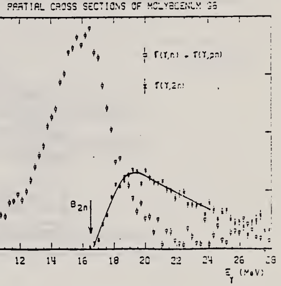
Fig. 3. Same as fig. 1, for ^{96}\text{Mo} .
