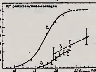
FIG. 4. Dependence of photoproton yield Y_p and photo-neutron yield Y_n from Nb^{93} on E_{\gamma,max} . For Y_p : x—present work, o—[6], □—[7]; the yields have been multiplied by the factor 5. For Y_n : x and o—measured in [11] and [12], respectively; the smooth curve was obtained in [10].
