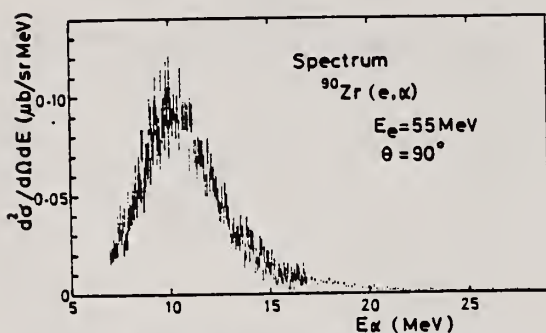
FIG. 4. (e, α) energy spectrum of 90 Zr at θ=90°, for E e =55 MeV. Alpha-particle energy was corrected for energy loss in half target thickness.
