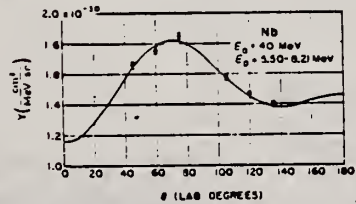
Fig. 9. Angular distribution of protons from Nb. The curve is a plot of the expression (1.31 - 0.15 \cos \theta + 0.41 \sin^2 \theta + 0.65 \cos \theta \sin^2 \theta) \times 10^{-20} , which is a four-parameter least-squares fit to the data.
