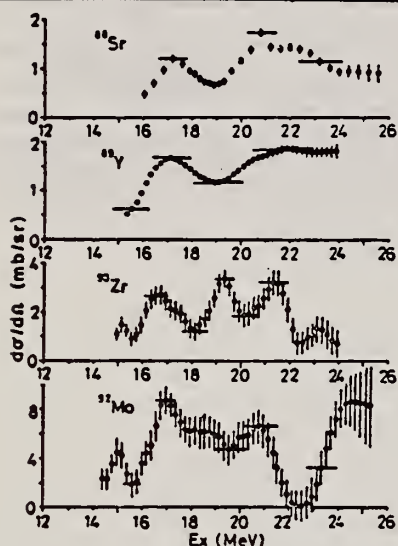
Fig. 3. Differential (γ, p) cross sections at θ = 90° analysed from (e, e'p) cross sections by the least structure method.
