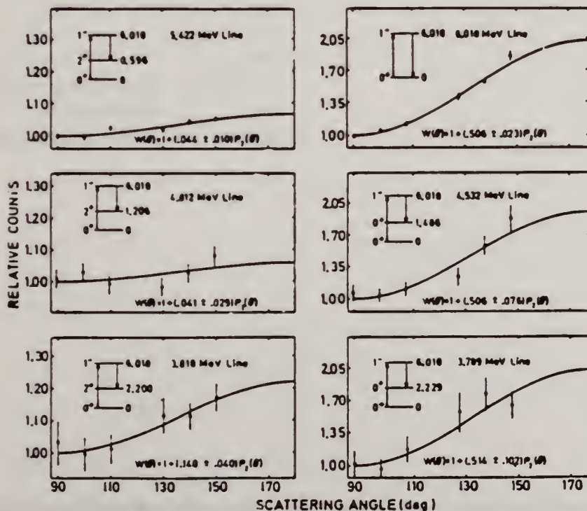
FIG. 4. Angular distribution of the elastic and some intense inelastic lines in 14 Ge as measured using a 20- \infty Ge(Li) detector. The solid lines have the form W(\theta) = 1 + AP_2(\cos\theta) and are least-square fits to the experimental distribution. In each case the corresponding \gamma - \gamma cascade is indicated.
