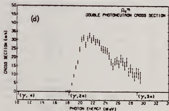
FIG. 5. Photoneutron cross sections for As 75 . (a) Total photoneutron cross section \sigma[(\gamma, n) + (\gamma, pn) + (\gamma, 2n)] . The solid line is a single-component Lorentz-curve fit to the giant-resonance data (13.6 to 21.3 MeV). (b) Total photoneutron cross section, repeated. The solid line is a two-component Lorentz-curve fit to the giant-resonance data. (c) Single photoneutron cross section \sigma[(\gamma, n) + (\gamma, pn)] . The dashed line represents the maximum systematic error owing to the uncertainty in the normalization of the positron bremsstrahlung subtraction. (d) Double photoneutron cross section \sigma(\gamma, 2n) .
