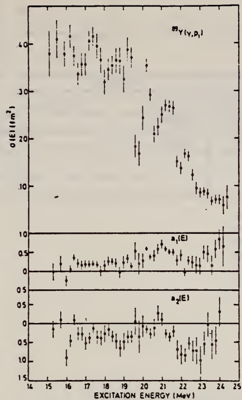
FIG. 8. The upper half of the figure shows the total \sigma(E) cross section, while in the lower half the angular distribution coefficients a_1(E) and a_2(E) are represented.
