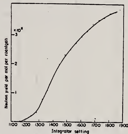
Fig. 4-2. Activation curve for Mo 92 (γ, n)Mo 91 .
