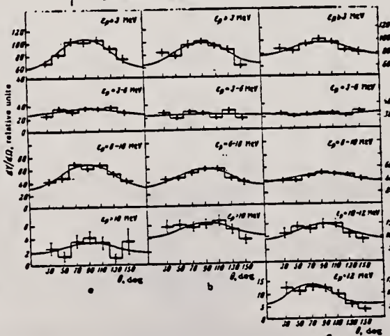
FIG. 3. Angular distributions of photoprotons from Nb^{93} for E_{\gamma,max} = 19.5 MeV (a), 23.5 MeV (b), and 27.5 MeV (c). The histograms are the experimental results. The smooth curves represent distributions of the forms I(\theta) = a + b \sin^2 \theta and I(\theta) = a + b \sin^2 \theta + c \sin^2 \theta \cos \theta . The parameters a, b, and c obtained by least squares are given in Table II.
