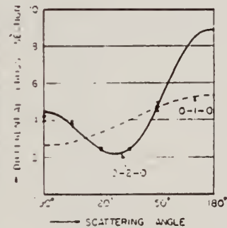
FIG. 4. Angular distribution of the resonance radiation from the 596-kev level in Ge 74 . The solid line represents the theoretical angular distribution for an excited state with spin 2 and a ground state with spin 0, corrected for the finite angular resolution. The differential cross section is given in arbitrary units.
