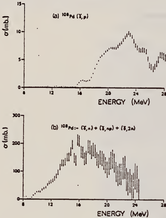
Fig. 2. (a) The (\gamma, p) cross section in ^{108}\text{Pd} , obtained using an analysis bin width of 1.5 MeV. (b) The (\gamma, n) + (\gamma, np) + (\gamma, 2n) cross section in ^{108}\text{Pd} , obtained using an analysis bin width of 0.5 MeV.
