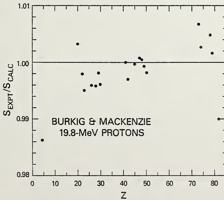
Fig. 4.5. Ratio of experimental to calculated proton stopping powers at 19.8 MeV. Experimental data are from Burkig and MacKenzie (1957).
