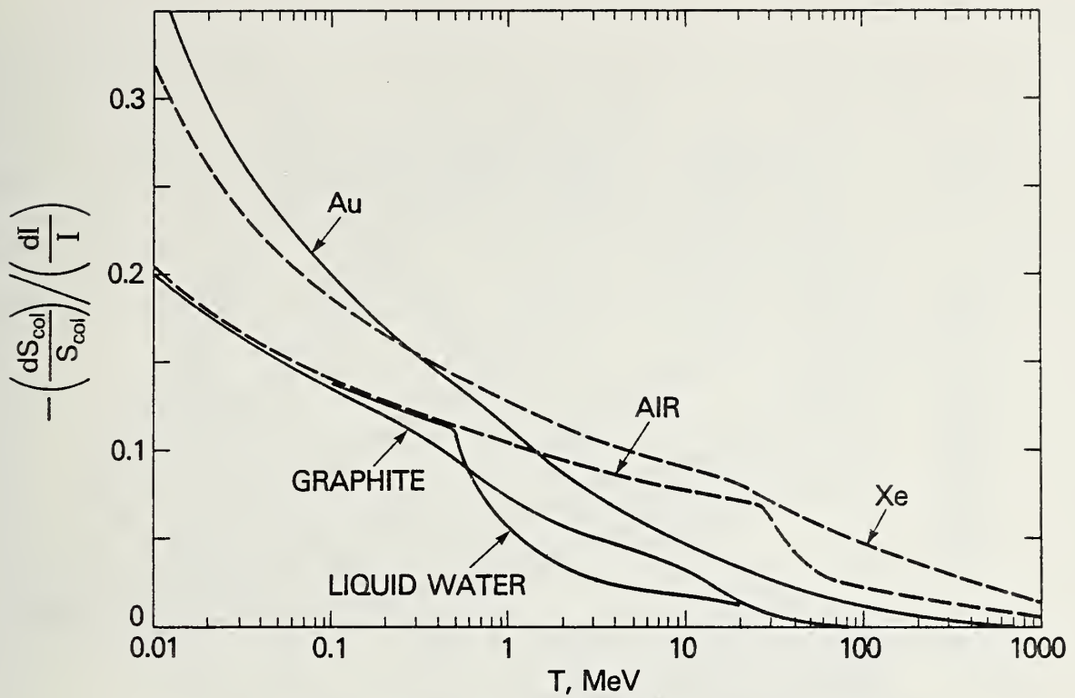
Fig. 3.1. Percent increase (decrease) of the collision stopping power for electrons resulting from a 1-percent decrease (increase) of the mean excitation energy.
