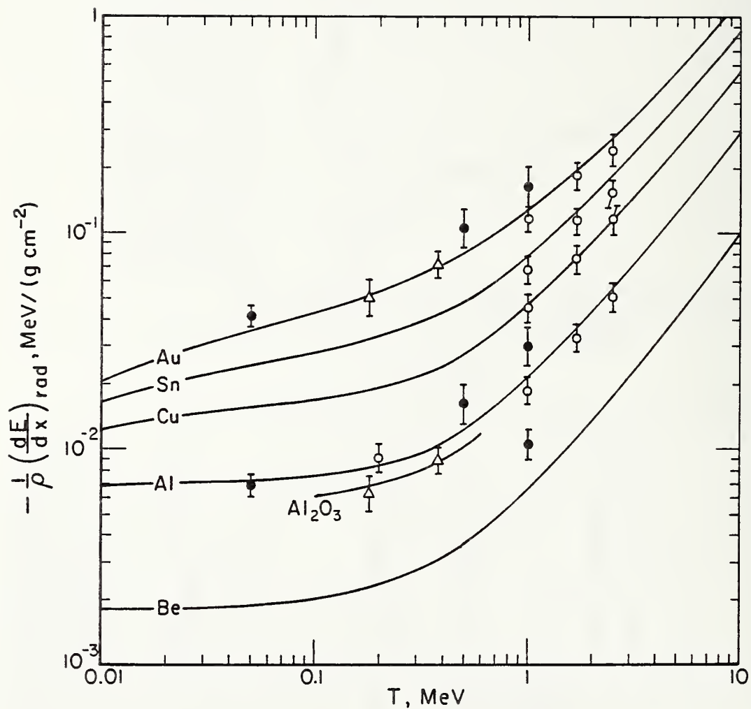
Fig. 9.3. Comparison of theoretical radiative stopping power, calculated according to Eq (9.1), with experimental results.
