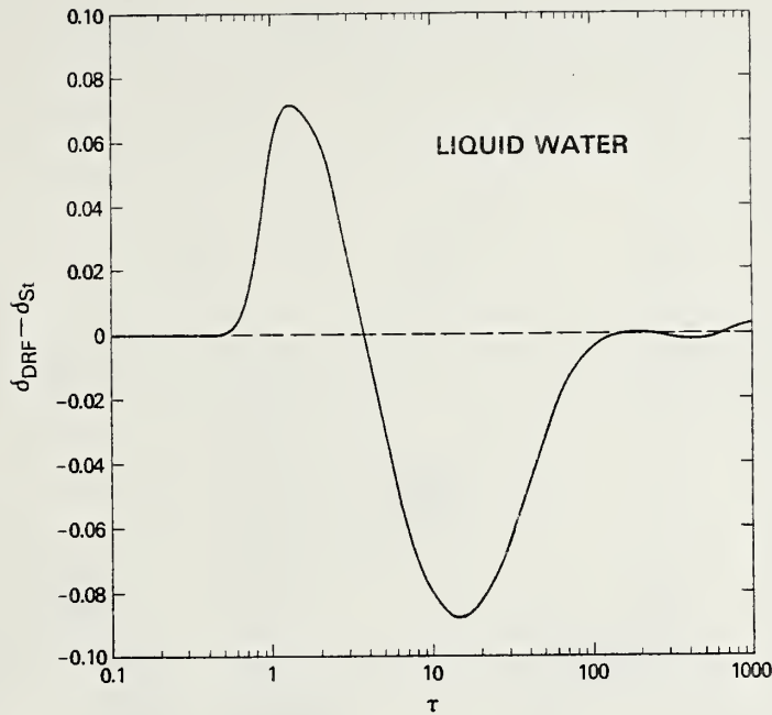
Fig. 6.3. Difference between the density-effect correction \delta_{DRF} calculated by Ashley (1982b) using a semi-empirical dielectric function for water, and the corresponding value \delta_{St} obtained by Sternheimer's method. The latter was calculated with I = 75.4 eV, to match the I -value for water found by Ashley.
