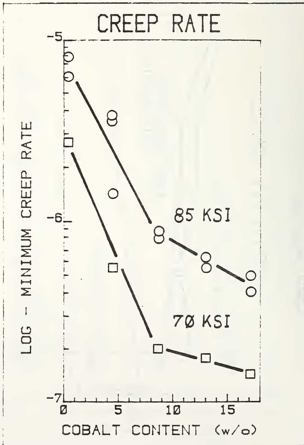
FIGURE 3 - Creep of Cobalt Modified Astroloy
