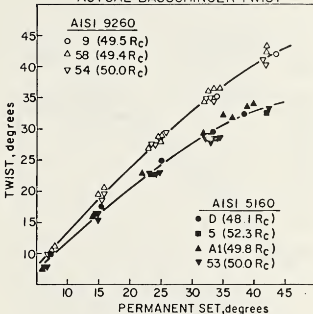
Fig. 3 - Comparison of the Bauschinger effect of AISI 5160 and 9260 spring steels
