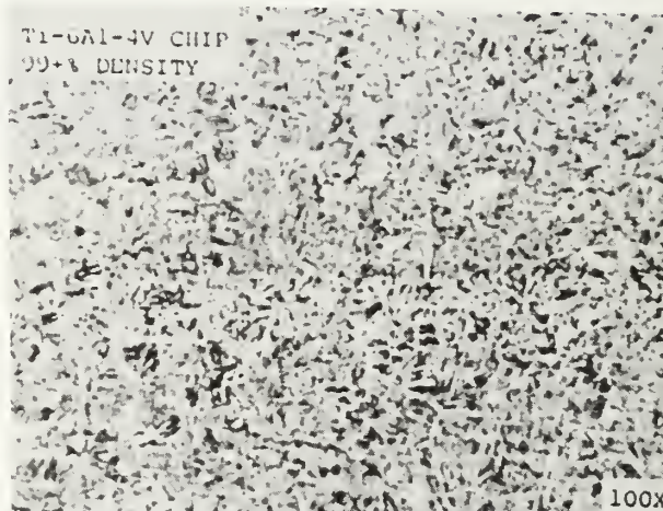
FIG. 7B MICROSTRUCTURE Ti-6Al-4V COLD ISOSTATIC PRESSED AND SINTERED FOLLOWED BY HIP
