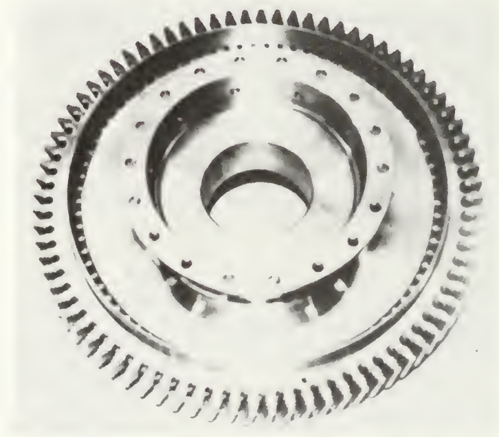
Figure 2 Typical High Pressure Turbine Disk Used to Evaluate Inconel 718 Substitution
