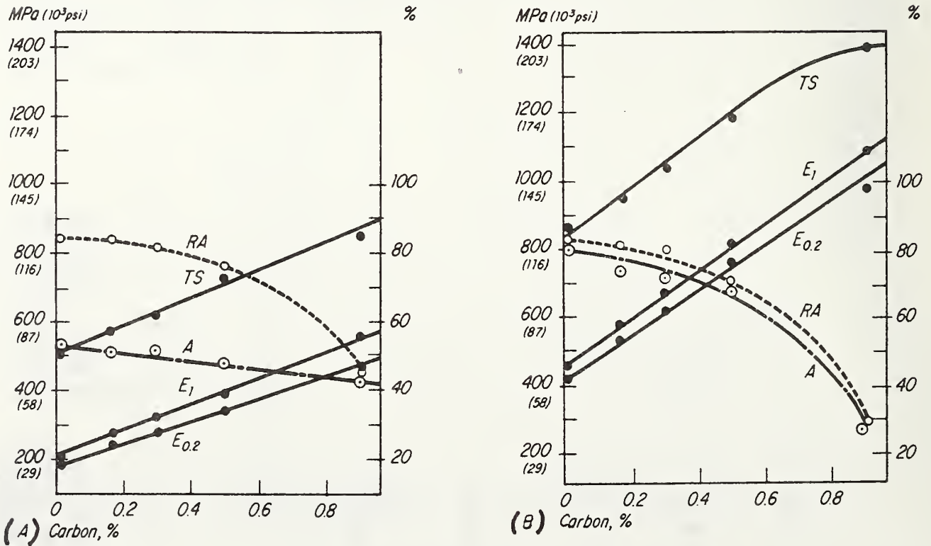
Fig. 9. The effect of carbon on the mechanical properties of Fe-30Mn-5Al alloys. Note that the properties at room temperature(A) are lower than those at liquid nitrogen temperature(B). TS=tensile strength; E_1 and E_{0.2} =yield strength (1 and 0.2% offsets); RA=reduction in area; A=elongation. -ref.(15)
