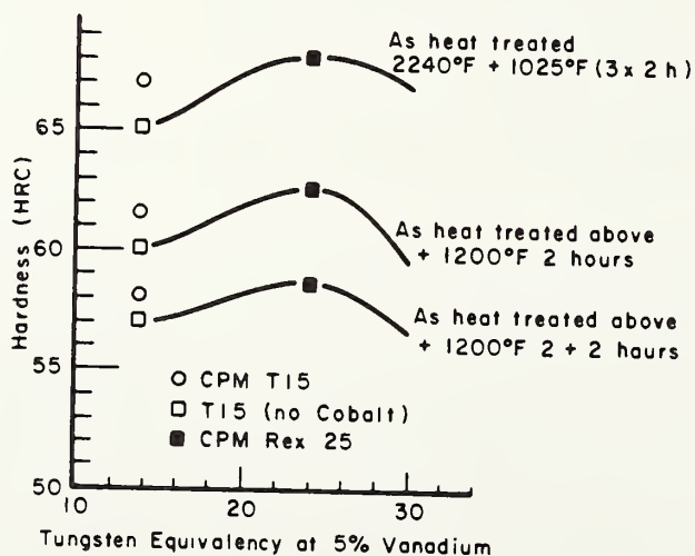
Figure 3 - Effect of Weq on Attainable Hardness and 1200F Temper Resistance of CPM Rex 25.
