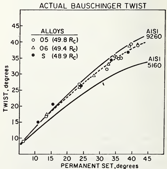
Fig. 7 - Comparison of the 5160 and 9260 ABT curves with ABT data for three alloys with almost the same potential load-loss resistance as 9260
