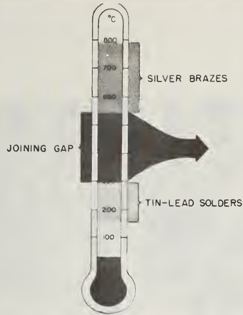
SOLDER/BRAZE JOINING GAP
