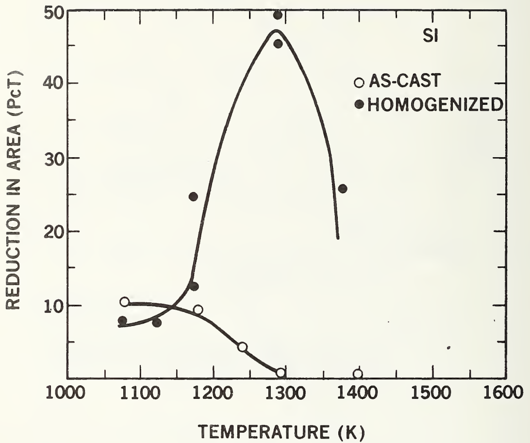
FIG. 13(A). HOT DUCTILITY TEST RESULTS FOR ALLOY S-1 - REF. (21)
