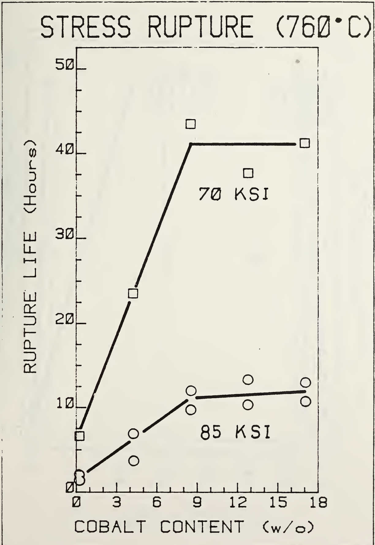
FIGURE 4 - Stress Rupture of Cobalt Modified Astroloy
