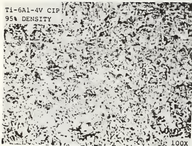
FIG. 7A MICROSTRUCTURE Ti-6Al-4V AS PRESSED AND SINTERED
