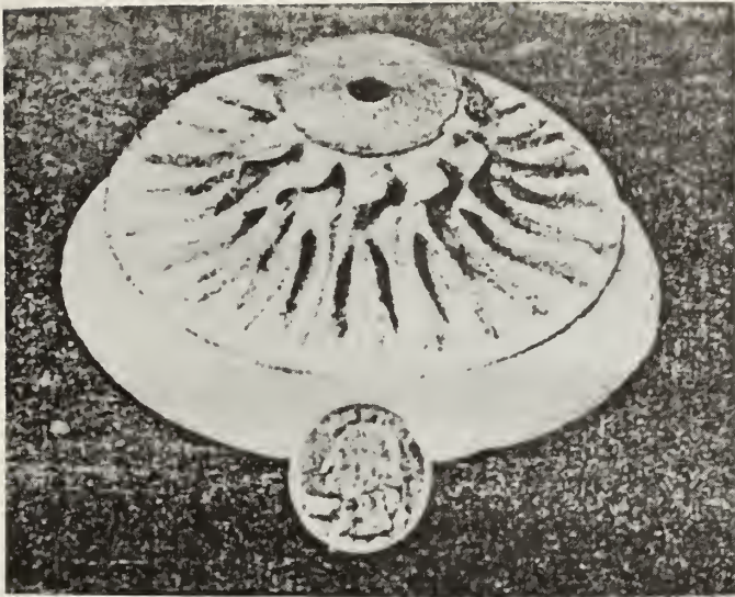
FIG. 8 Ti-6Al-4V RADIAL ROTOR
