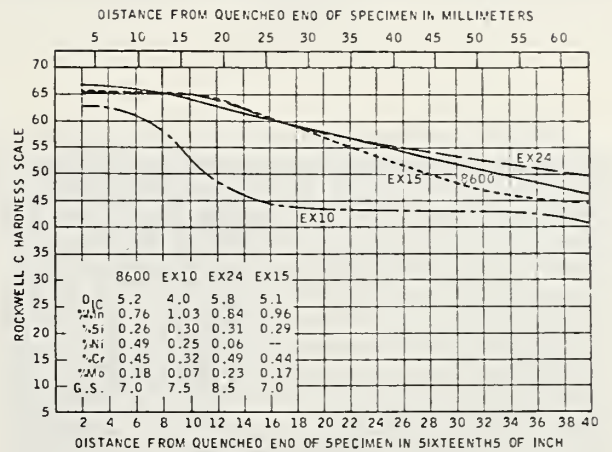
0.90% C case hardenability comparison (low-side chemistry).
