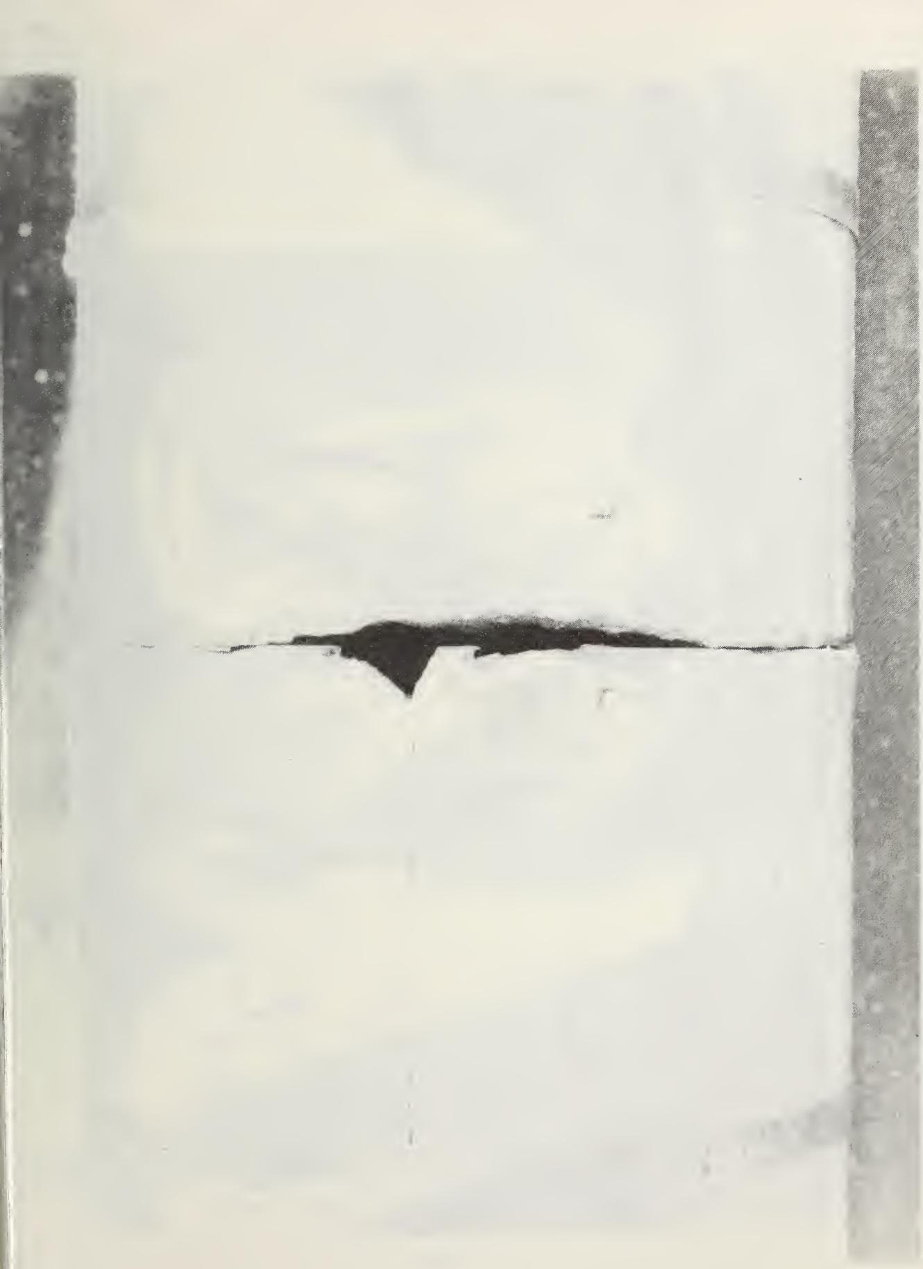
Figure 35. The joint of KAYLO-10 insulation jacket was eroded out by the boiling action of water outside the carrier pipe.
