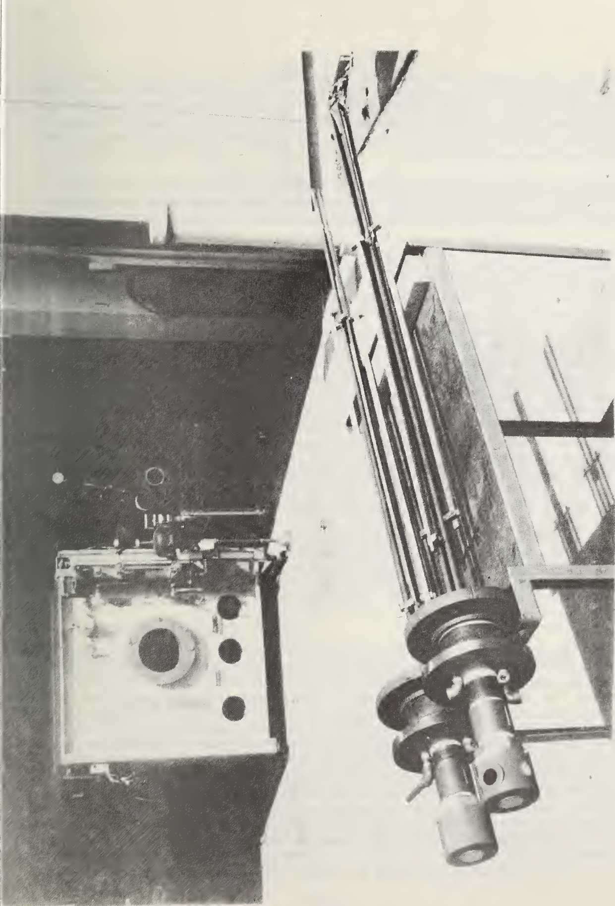
Figure 31. Immersion electric heaters for the heat loss test.
