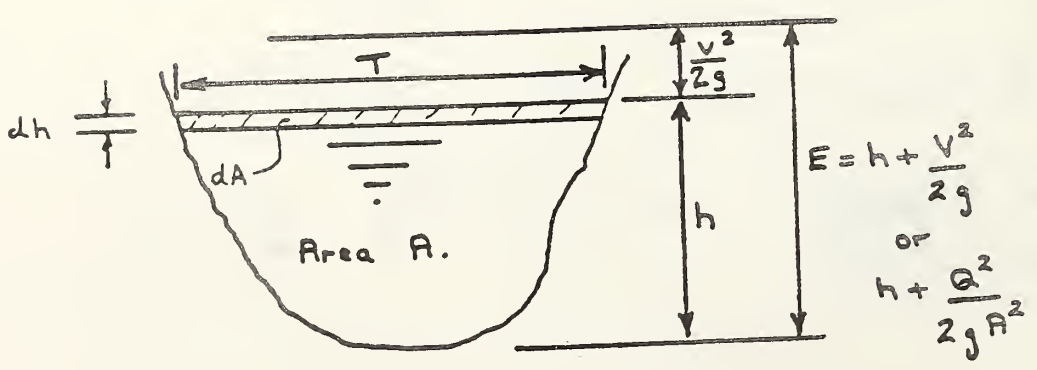
Figure 2. Relationship between flow specific energy and flow depth
