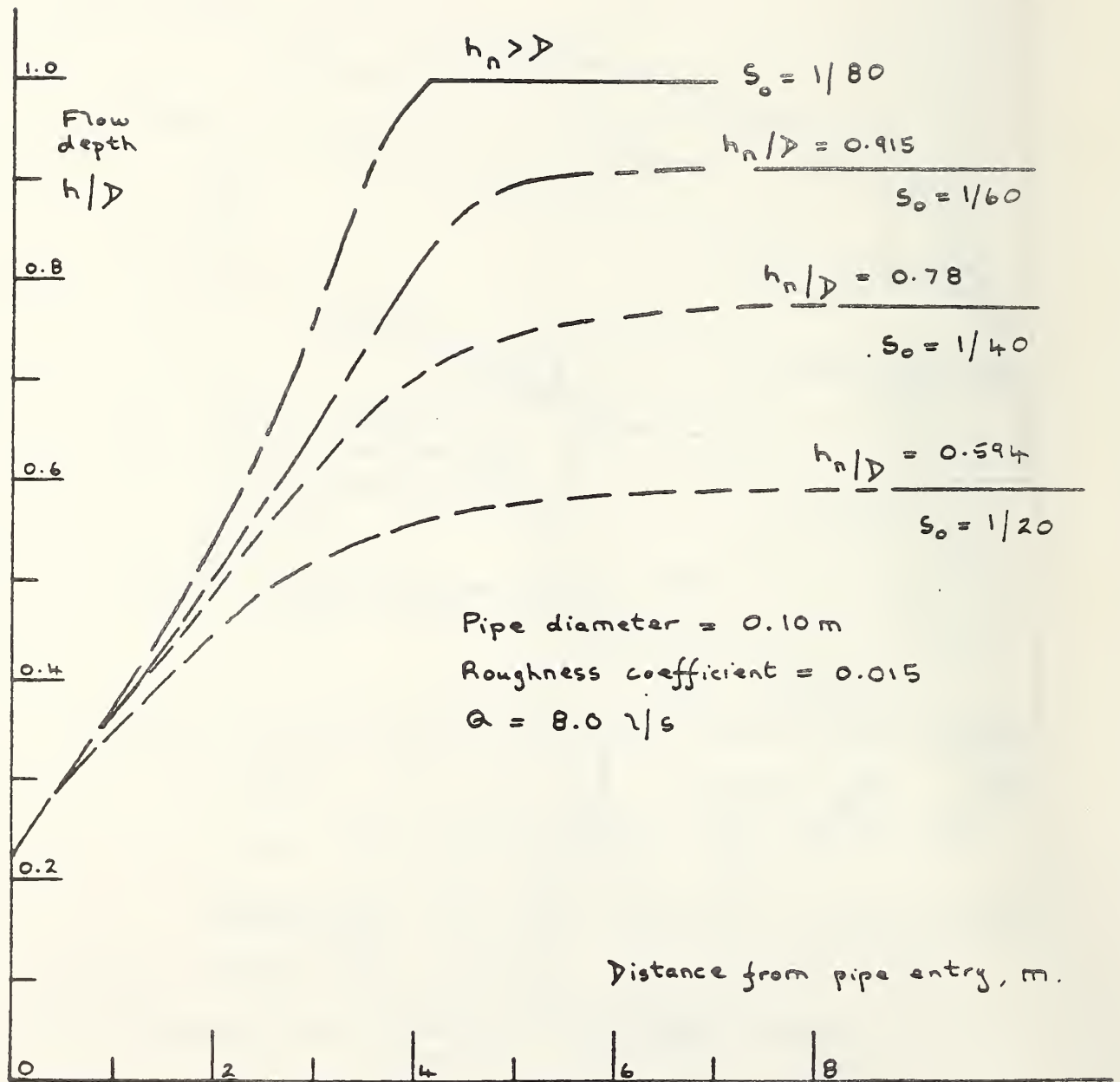
Figure 6. Water surface profiles for a range of pipe gradients, illustrating increase in transition length as pipe slope is increased
