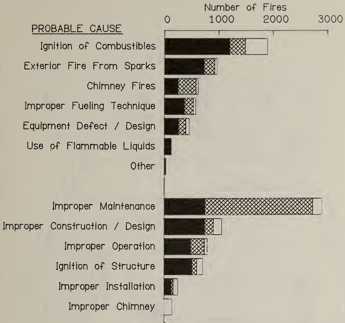
Figure 1: Breakdown of fire incidents by probable cause and equipment type as recorded in NFIRS fire incident data
