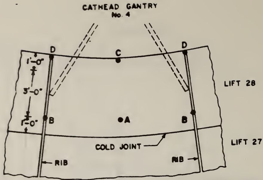
Figure 4.2 Location of maximum hoop and meridional stress resultants in lift 28 (points C,D and A,B, respectively)
