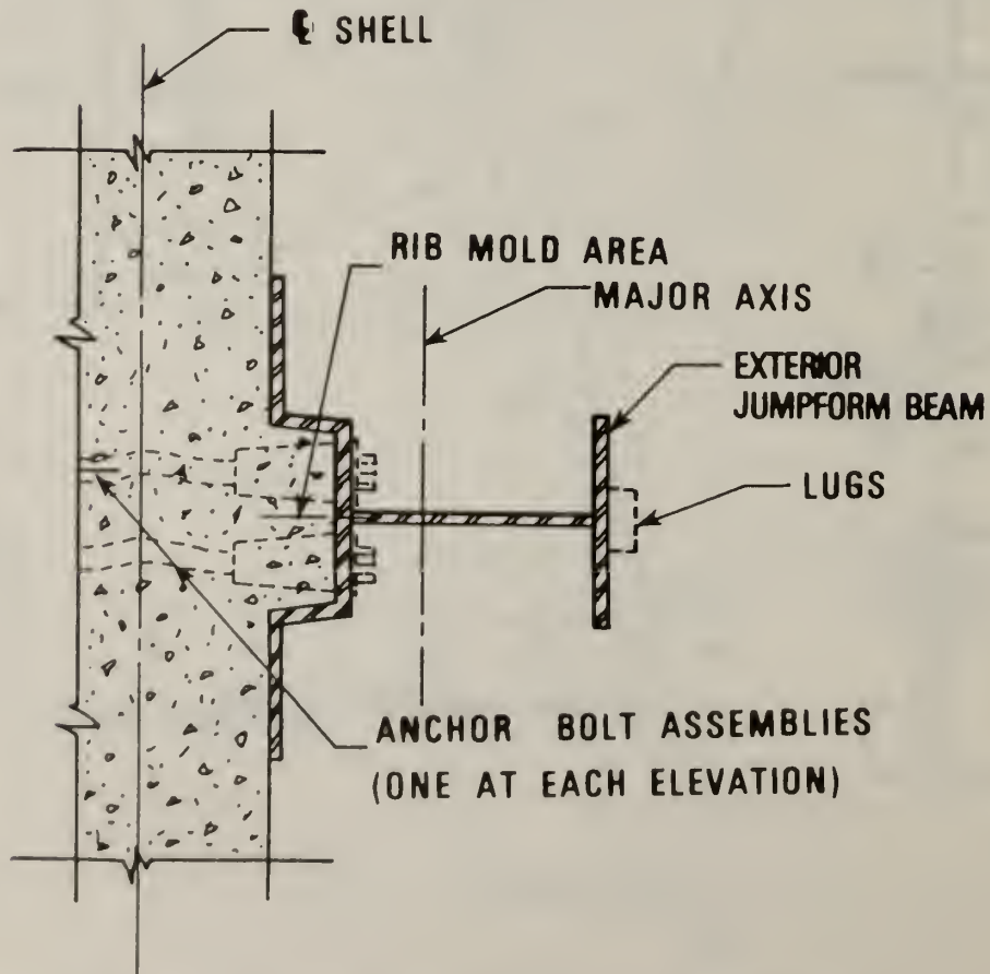
Figure 4.3 Sectional configuration at the interface of exterior jumpform beam and concrete shell
