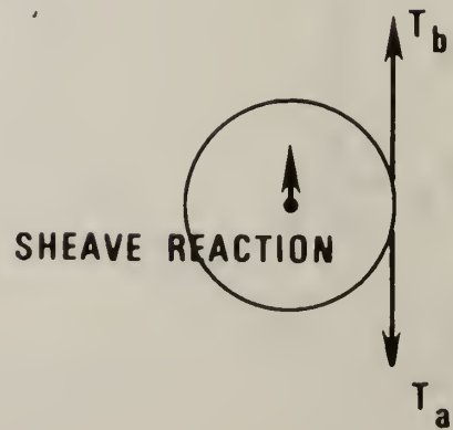
Figure 2.5 Idealization of hoisting cable as a one-dimensional system
