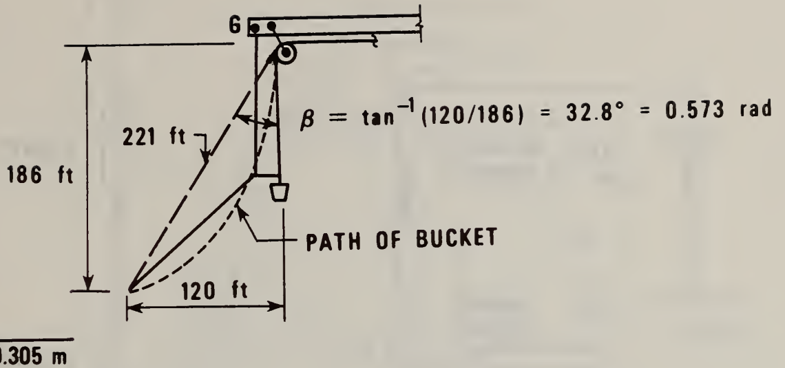
Figure 2.2 Path of the bucket
