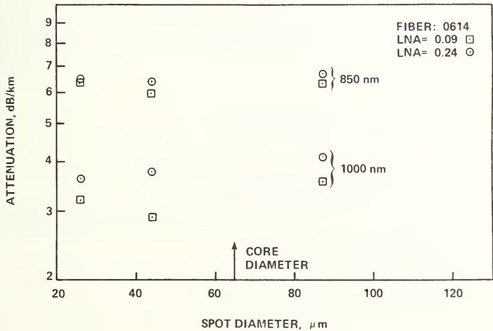
Figure 3.2 NBS data on fiber 0614 prior to comparison.
