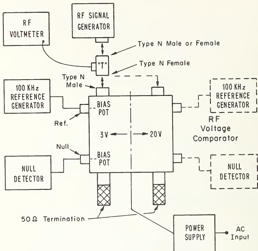
Figure 9. Block Diagram for Calibration of RF Voltmeters (0.01-20V)
