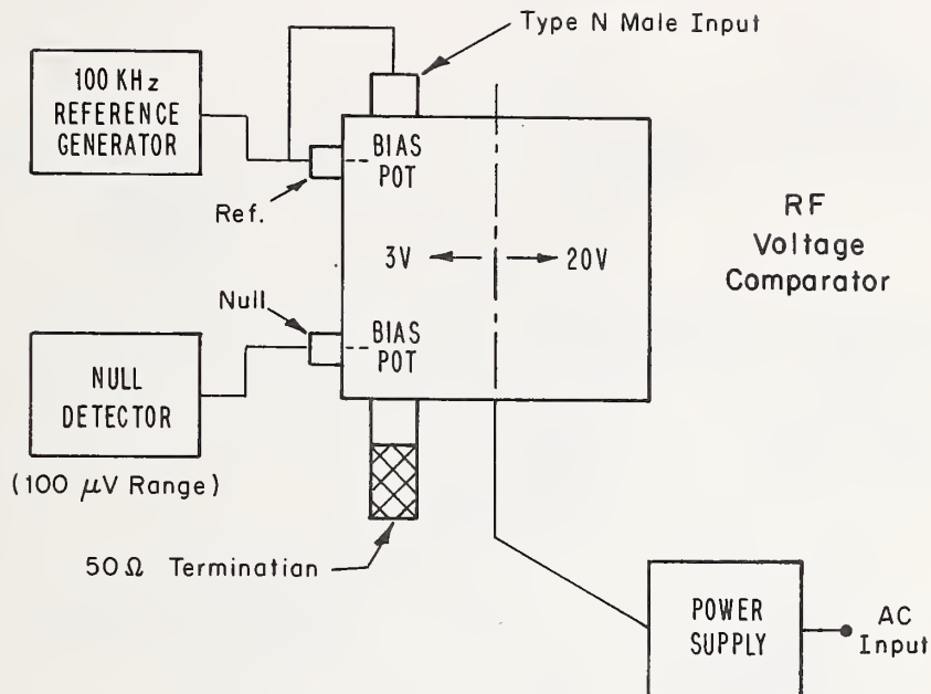
Figure 6. Offset Voltage Measurement Diagram
