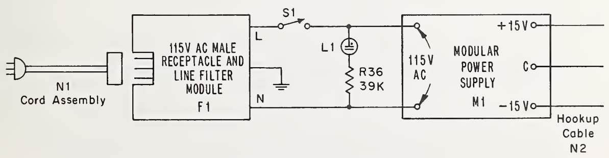
Figure 5. Block Diagram of Modular Power Supply (±15Volts)
