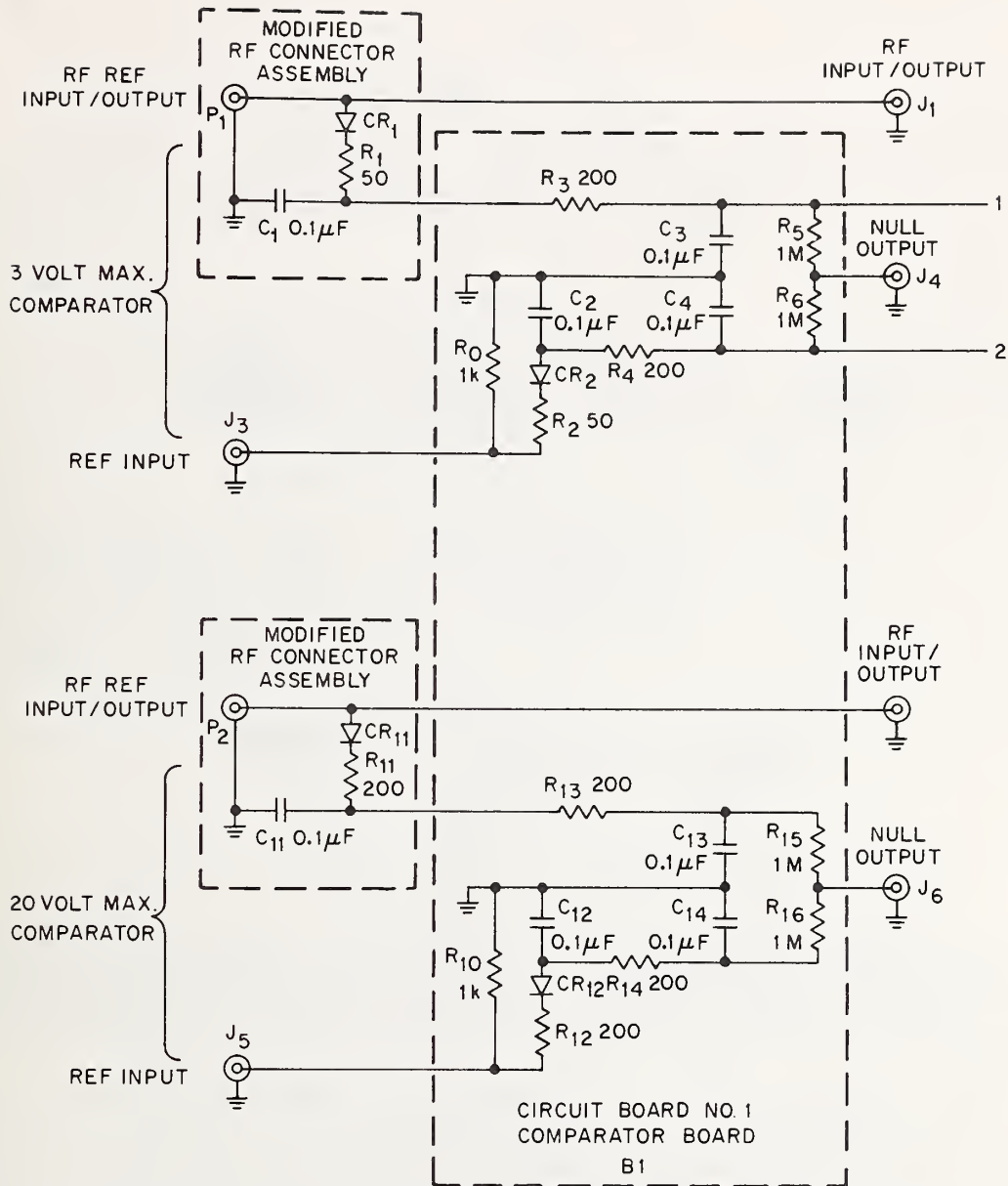
Figure 2. Circuit Diagram of Detector and Summing Networks of RF Voltage Comparator
