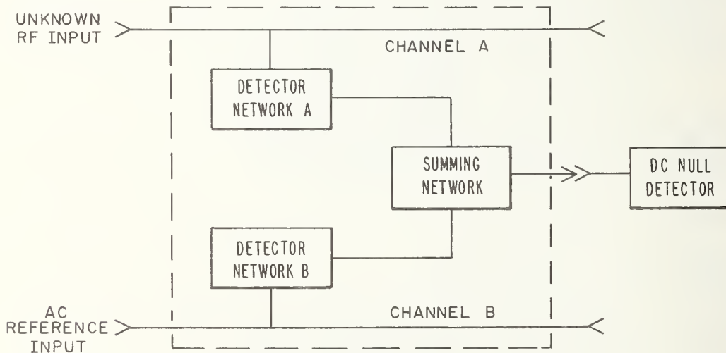
Figure 1. Basic Block Diagram of RF Voltage Comparator
