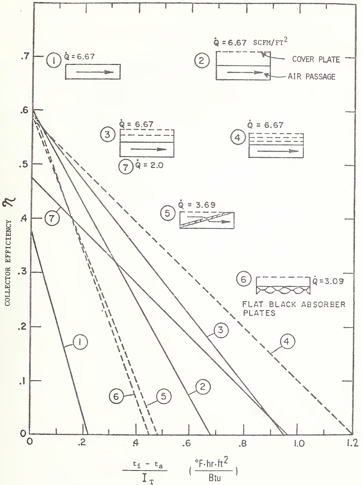
Figure 1A-3 Typical Thermal Efficiency Curves for Flat Plate Collectors Using Air as the Working Liquid, Based on Collector Gross Frontal Area [5] (Q indicates flow rate in standard cubic feet per minute (scfm) per unit collector area)
