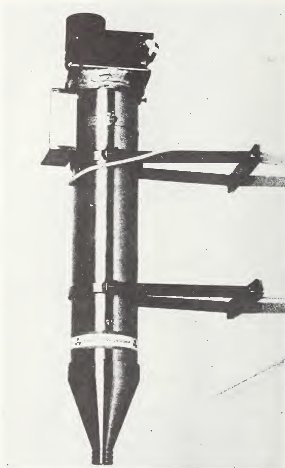
Figure 13. Hosemann reference ionization chamber
