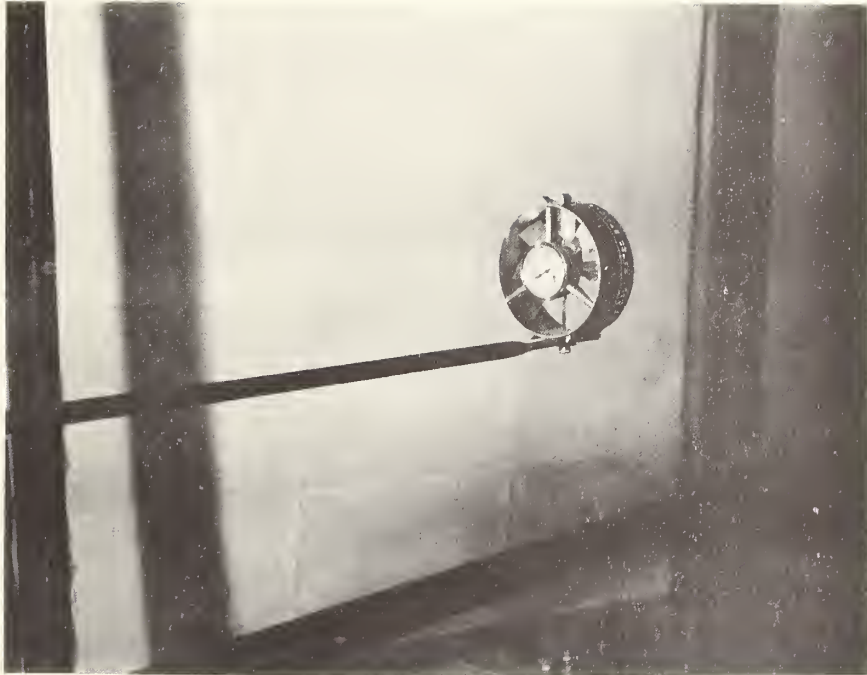
FIGURE 1. THE ANEMOMETER MOUNTED IN THE TUNNEL, SHOWING METHOD OF SUPPORT.
