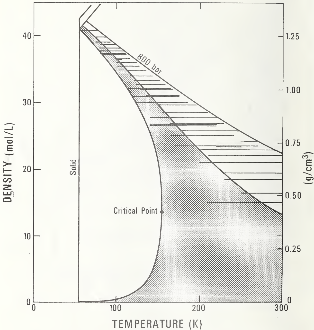
Figure 2. New experimental isochores (horizontal lines); shaded area shows the region of earlier NBS data.
