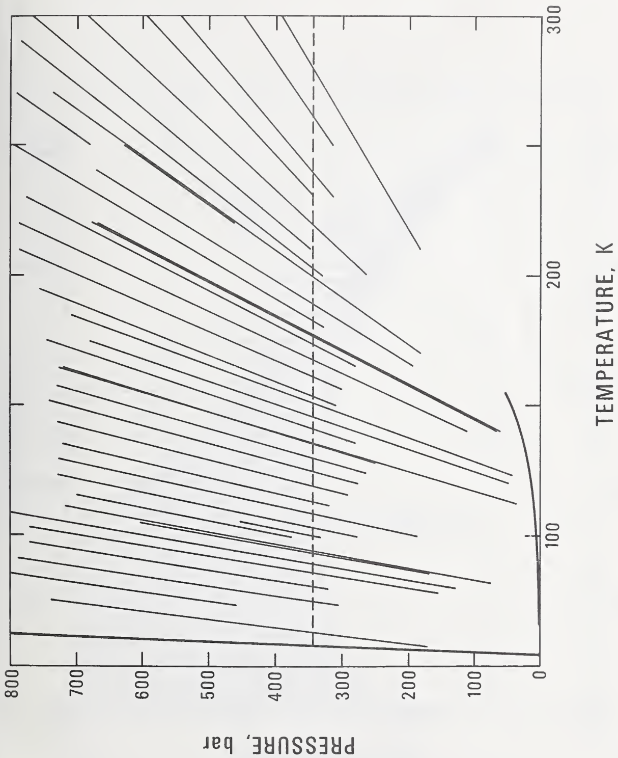
Figure 1. Experimental isochores. Dashed line indicates limit of earlier NBS data.
