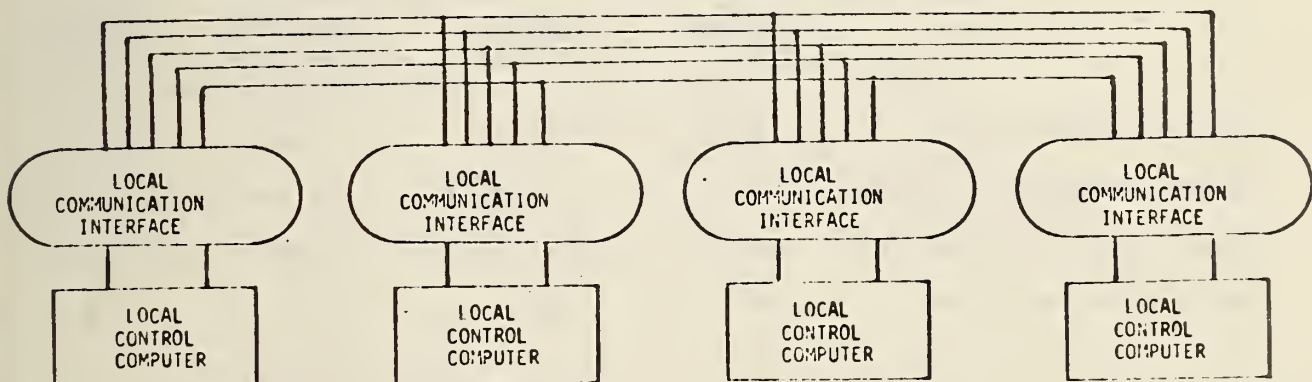
NETWORK CONTROL FUNCTION IS DISTRIBUTED OVER LOCAL COMMUNICATION INTERFACES
