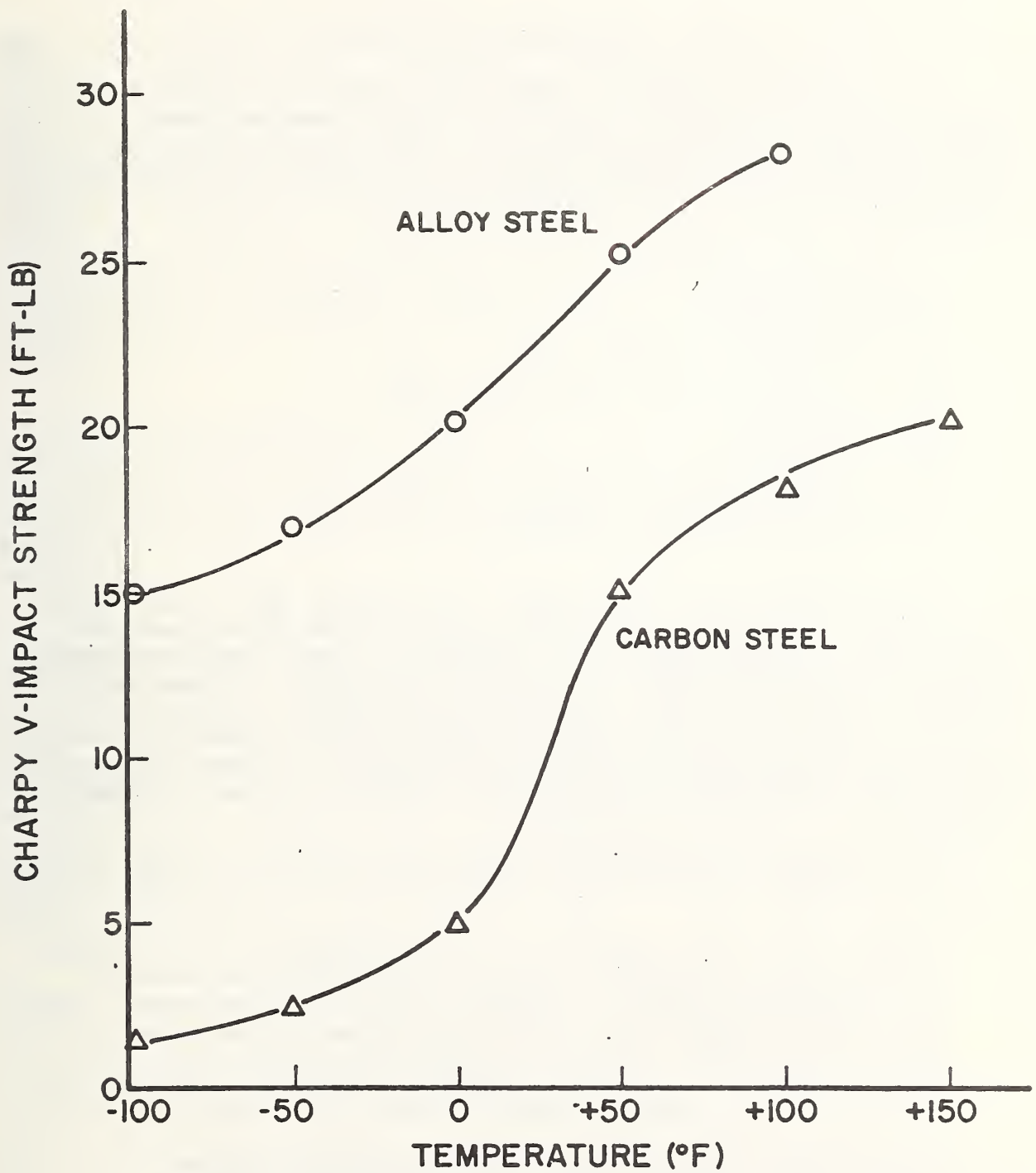
Figure 9. Impact Strength vs. Temperature Curves for Carbon and an Alloy Steel
