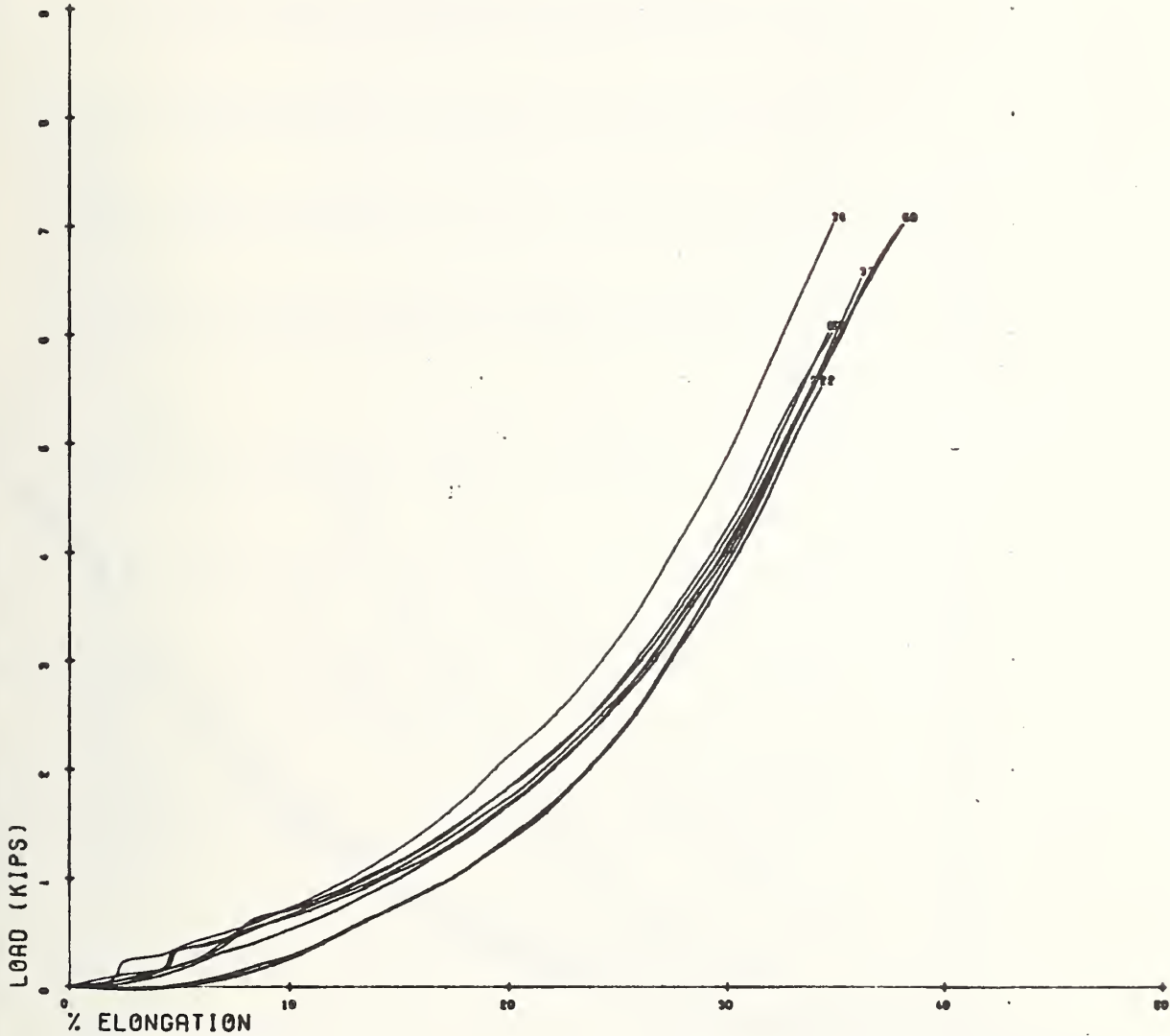
Figure A-13. Load/Relative Extension Curves Obtained for 1/2 inch Filament Nylon Lanyards.
