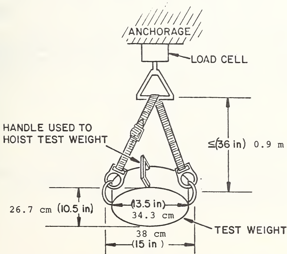
Figure 15. A Possible Setup for Dynamic Testing of Linemen's Body Straps.
