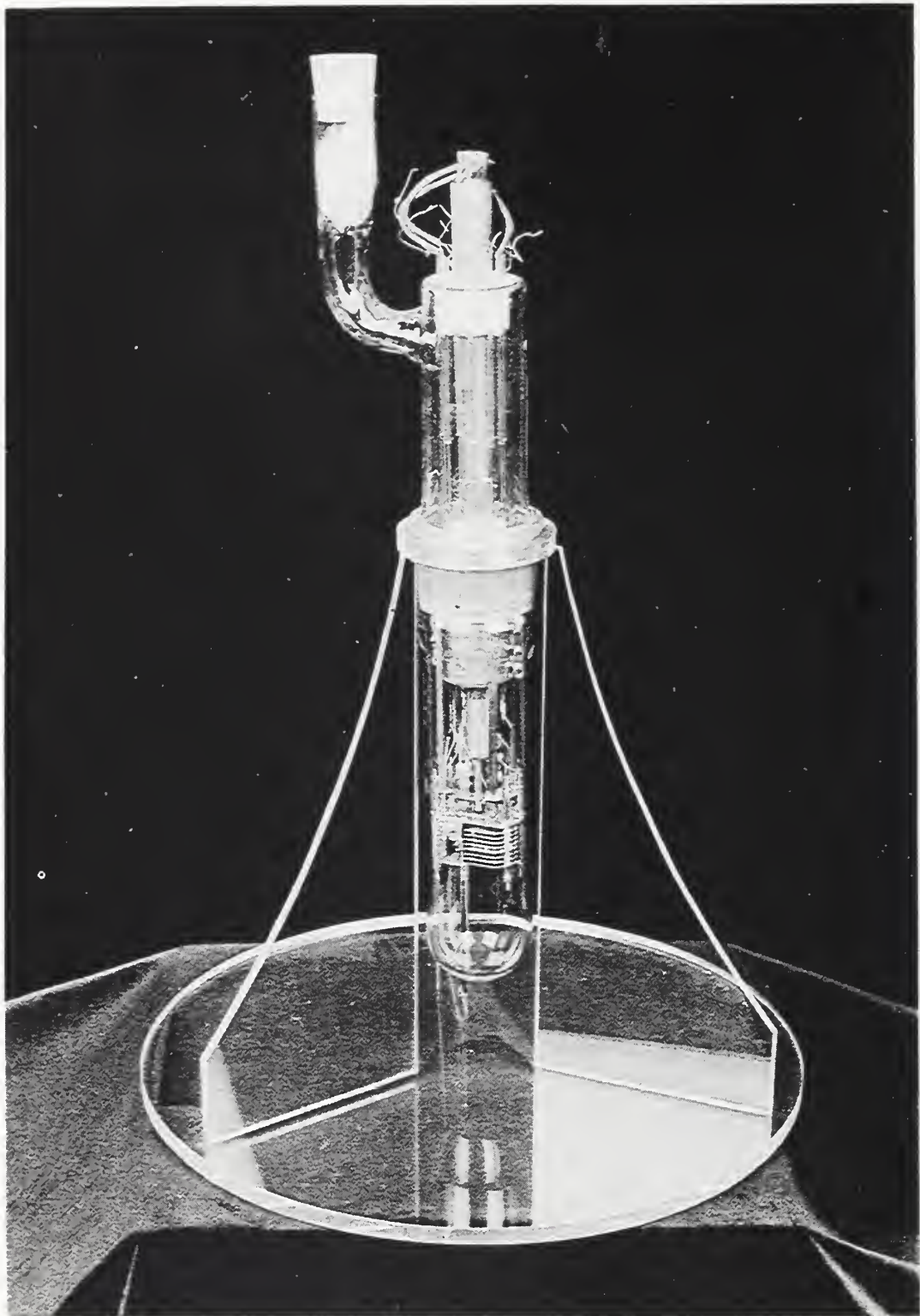
Omegatron (1951) M7
