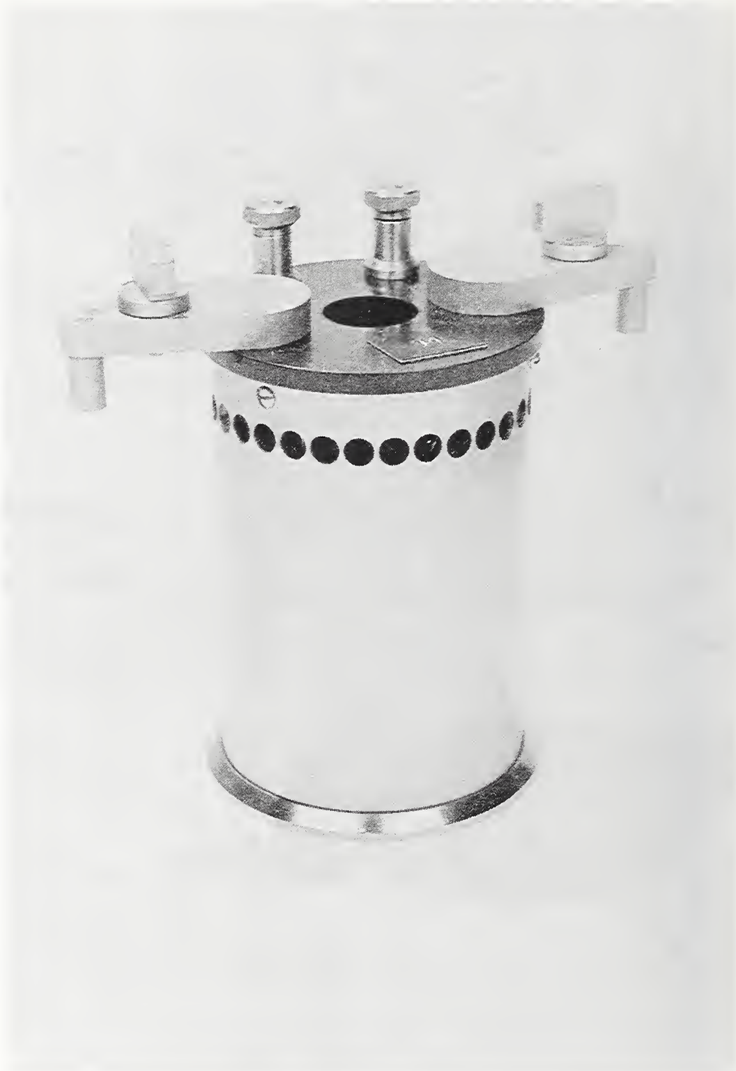
One-Ohm Resistor, Double-Walled (1930) R7
