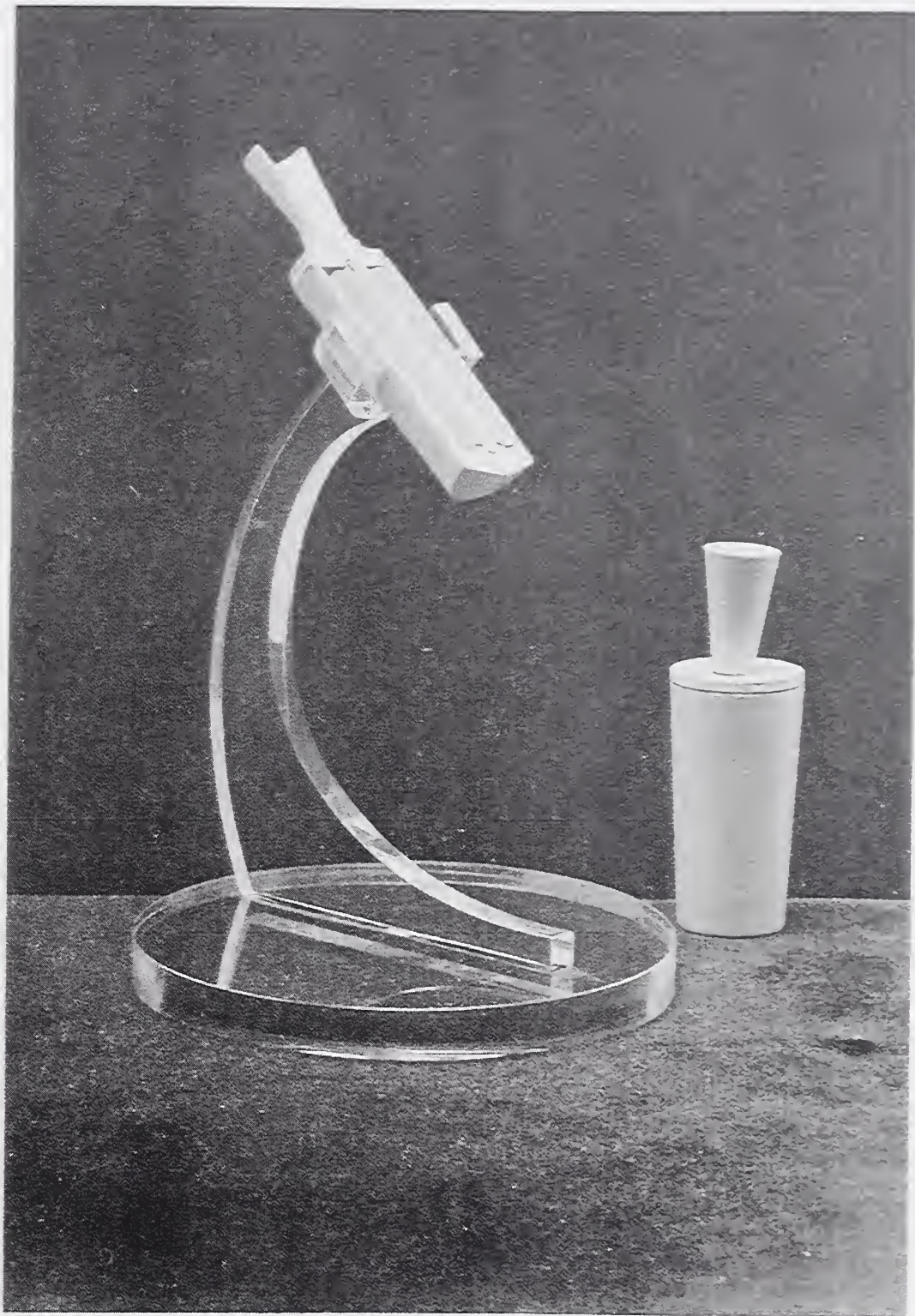
Platinum Blackbody (1930) M197
