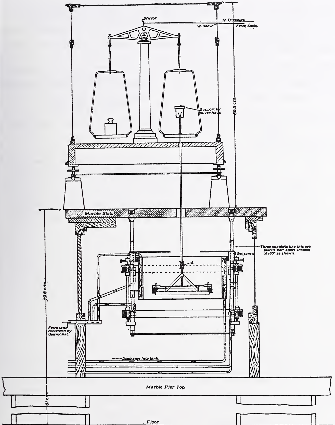
Rueprecht Balance (1901) M291 Schematic drawing of section of the assembled balance
