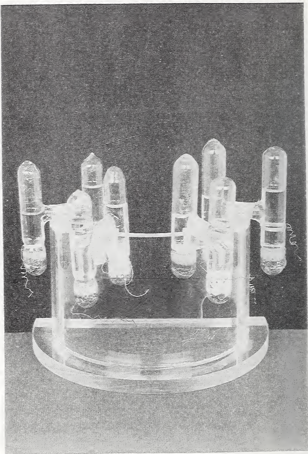
Weston Standard Cell (1905) M281
