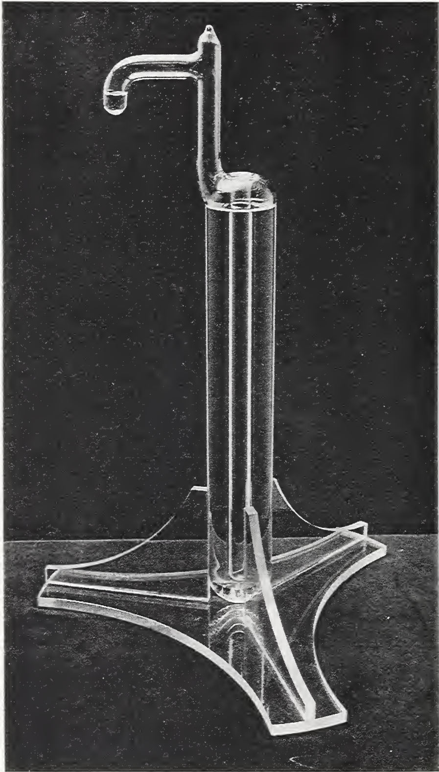
International Standard of Temperature Triple-Point Cell (1944) M524
