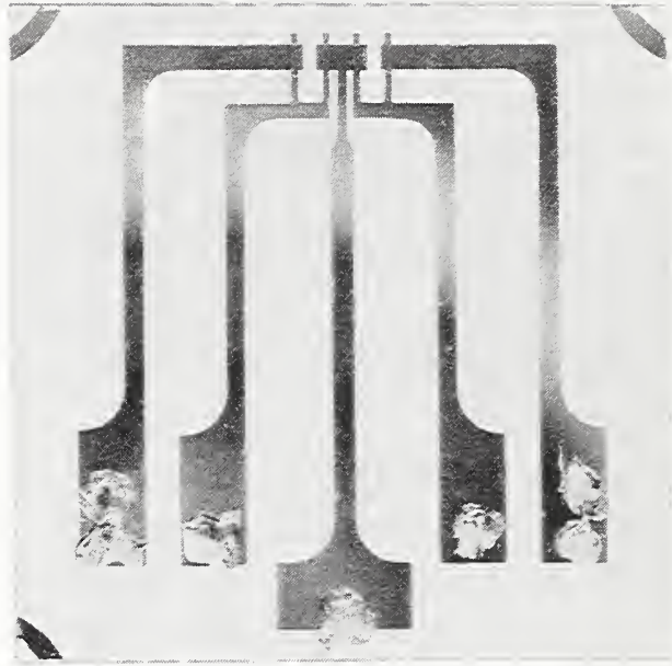
Josephson Junction (1971) M550
