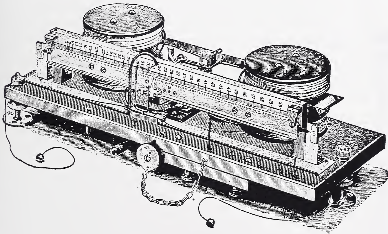
Current Balance, Kelvin (1902) M89
