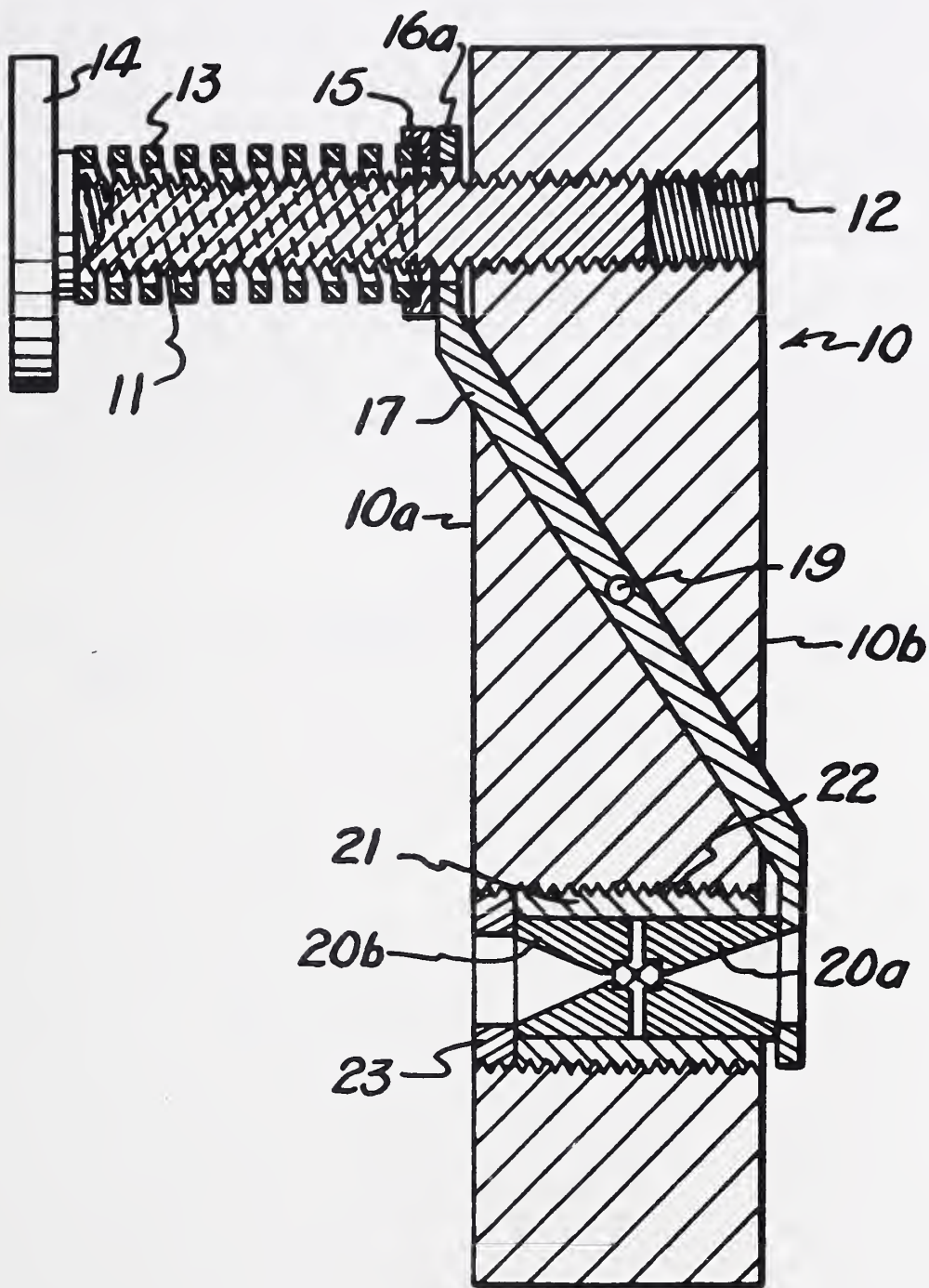
Diamond Anvil Optical Cell (1958) M325 Patent drawing of high-pressure optical cell
