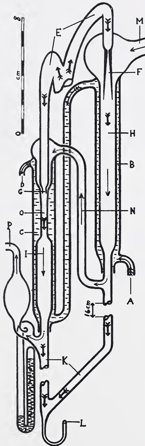
Vacuum Pump, Two-Stage (1917) M414 Schematic drawing
