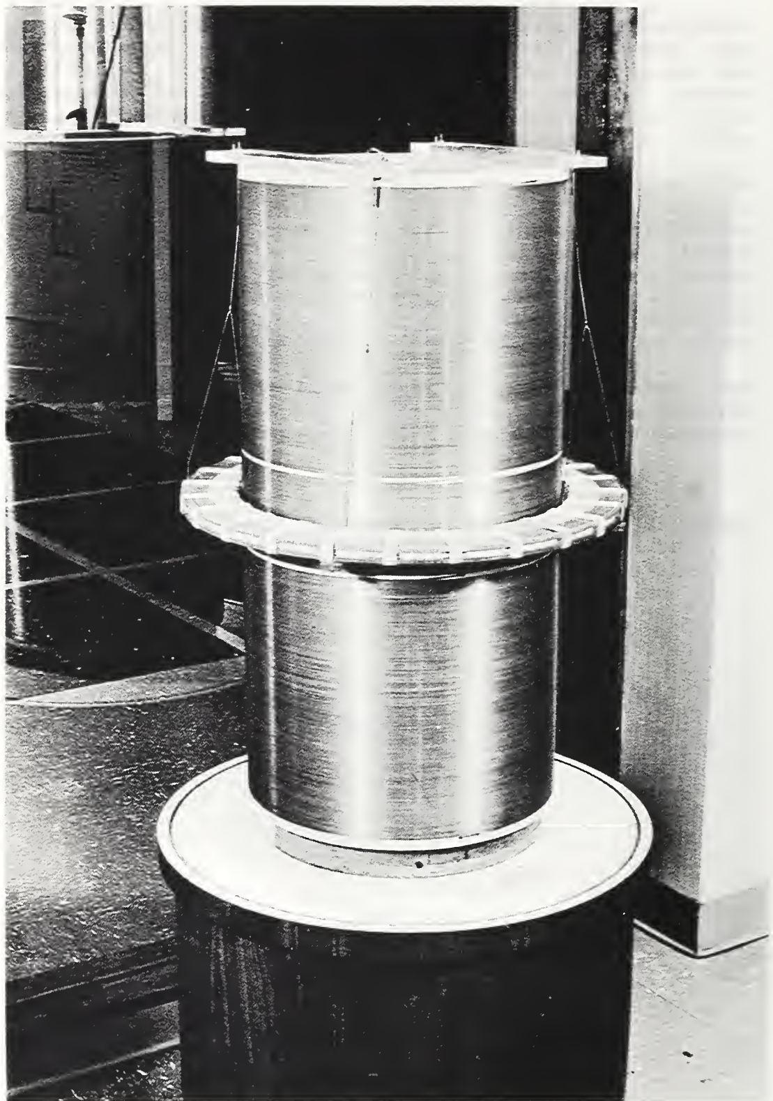
Mutual Inductor, Wenner (1938) M41
