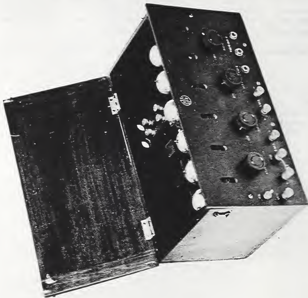
First AC Radio Receiver (1922) M166
