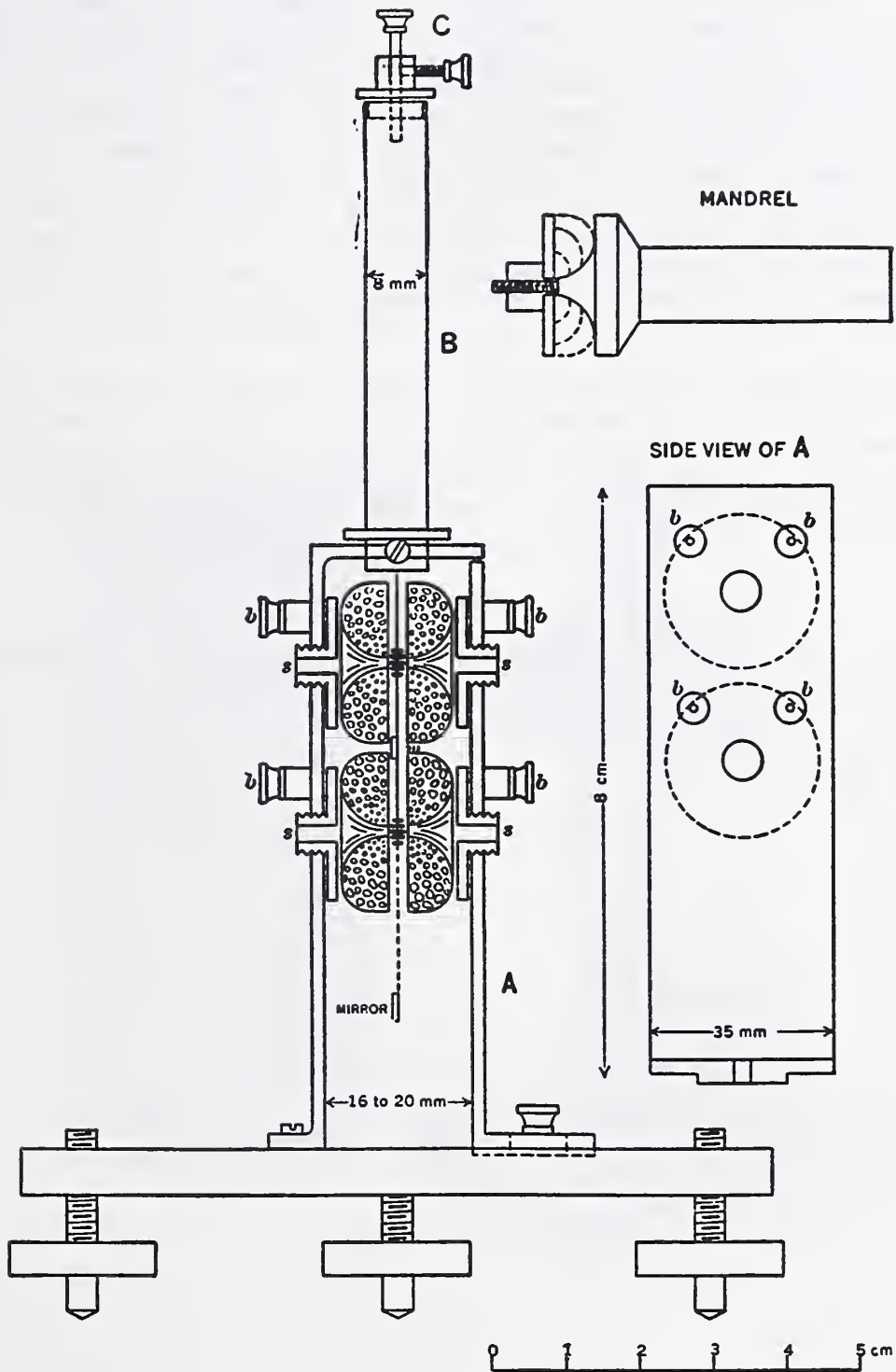
Schematic drawing of Galvanometer, Moving Magnet (1907) M219
