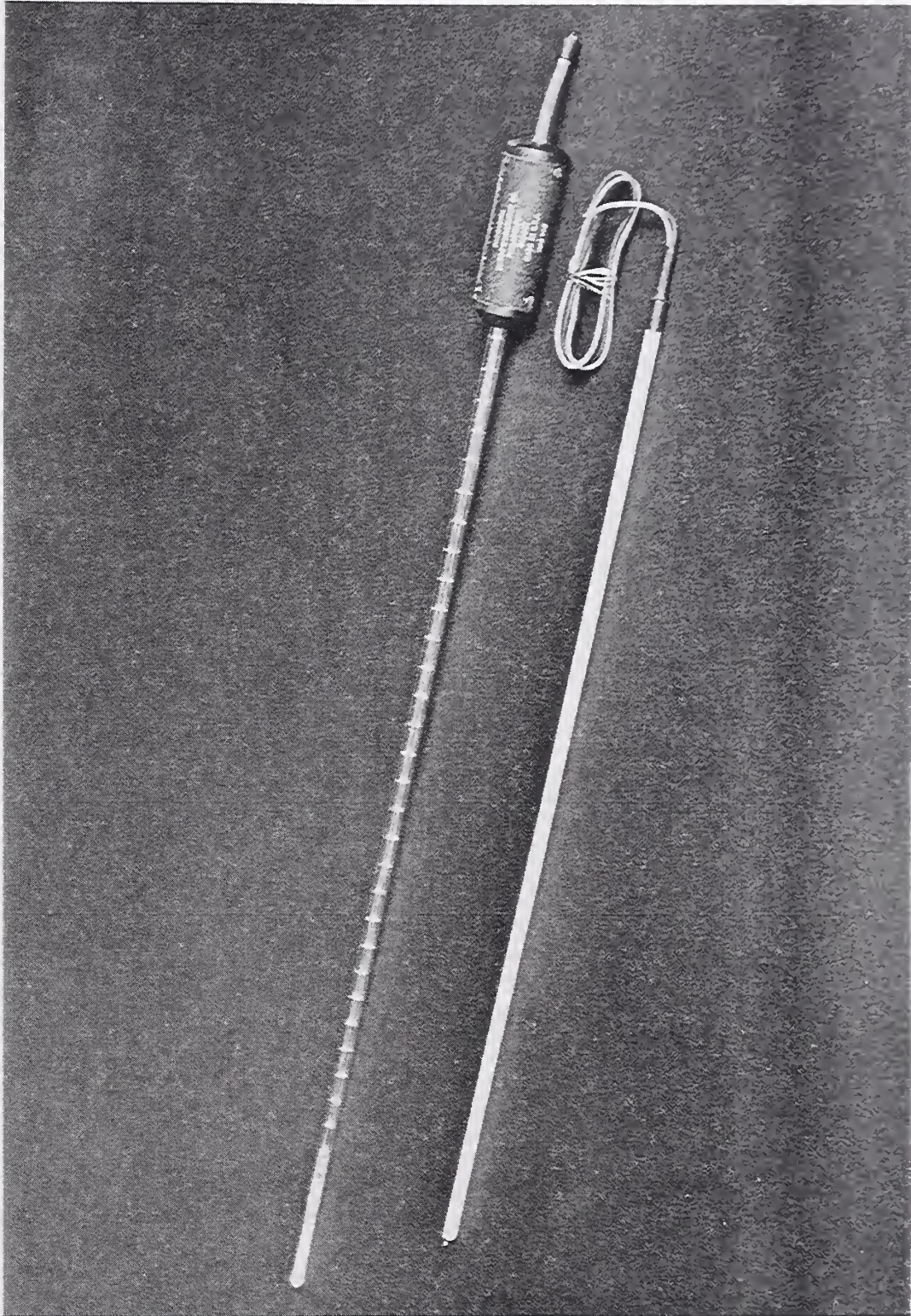
Thermocouple, Platinum vs. Platinum-10 Percent Rhodium M522
