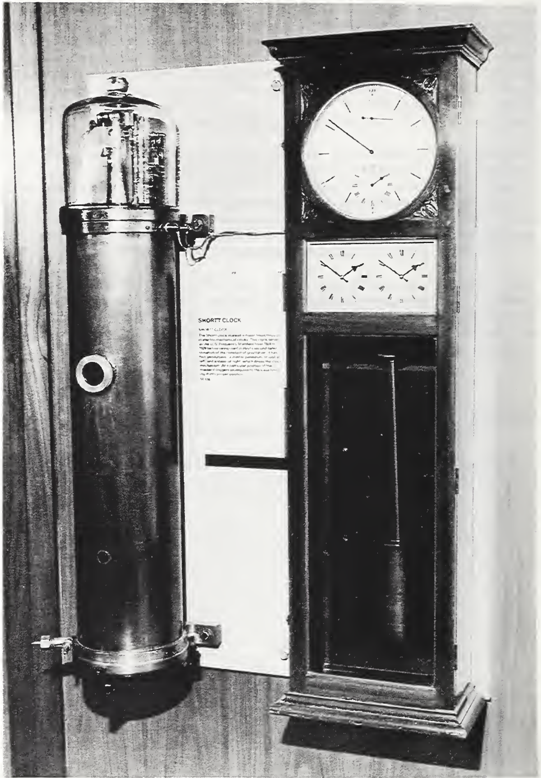
Shortt Clock (1921) M516
