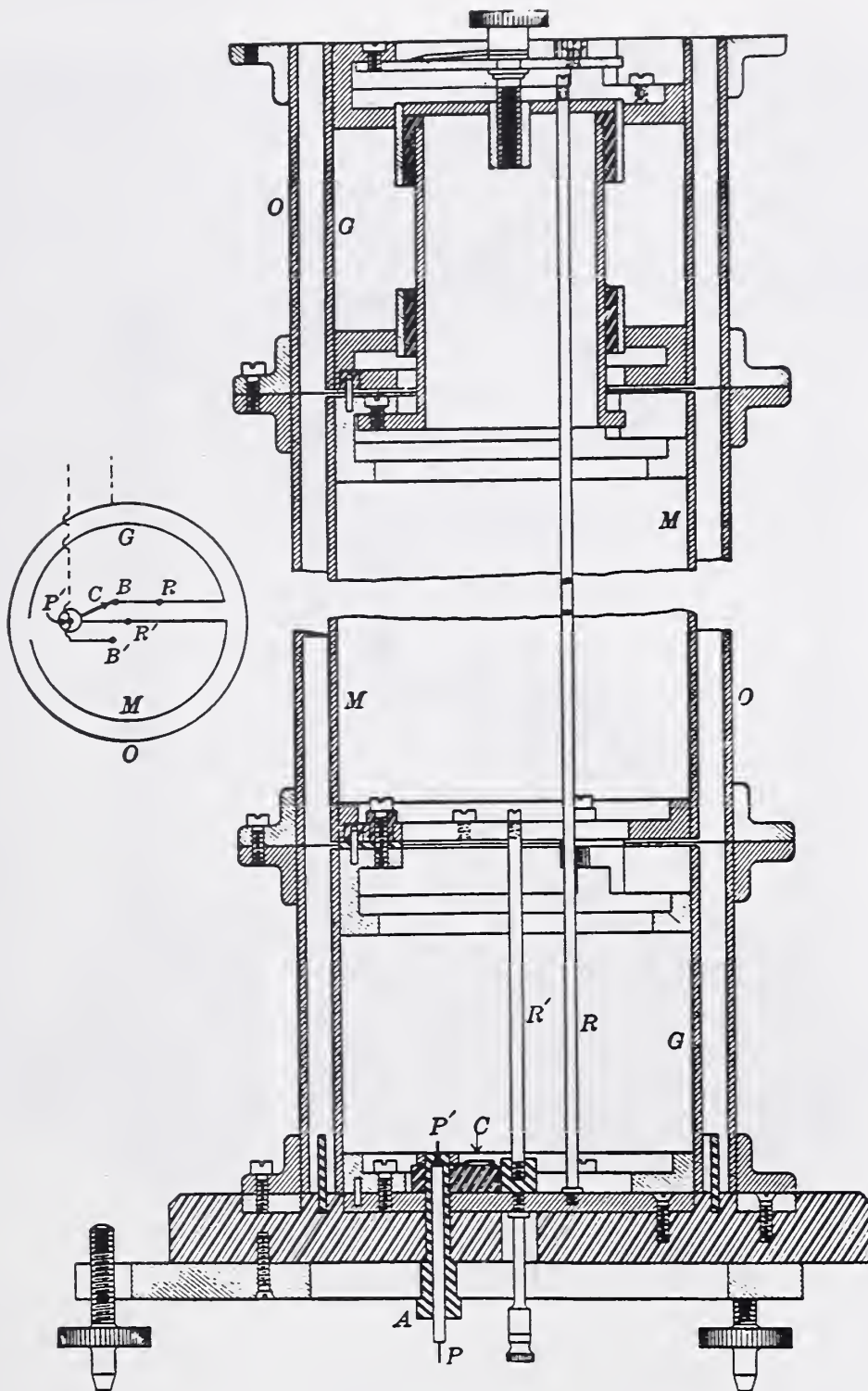
Cylindrical Capacitor (1904) M30 Schematic drawing of section
