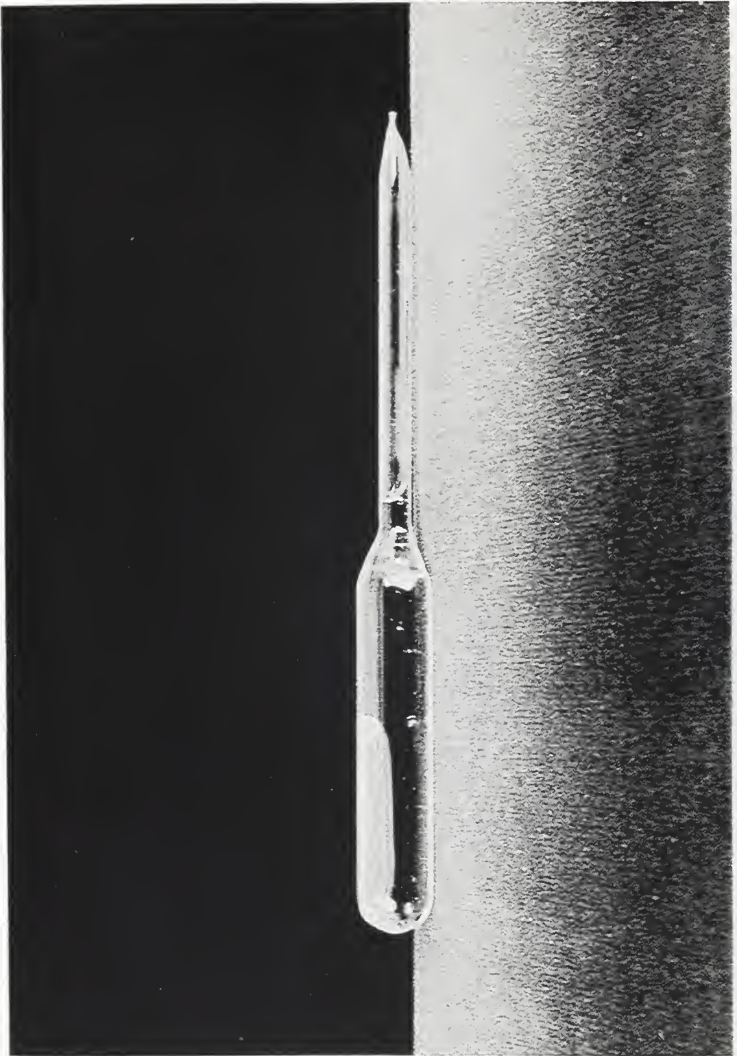
Heavy Water (1931) MII
