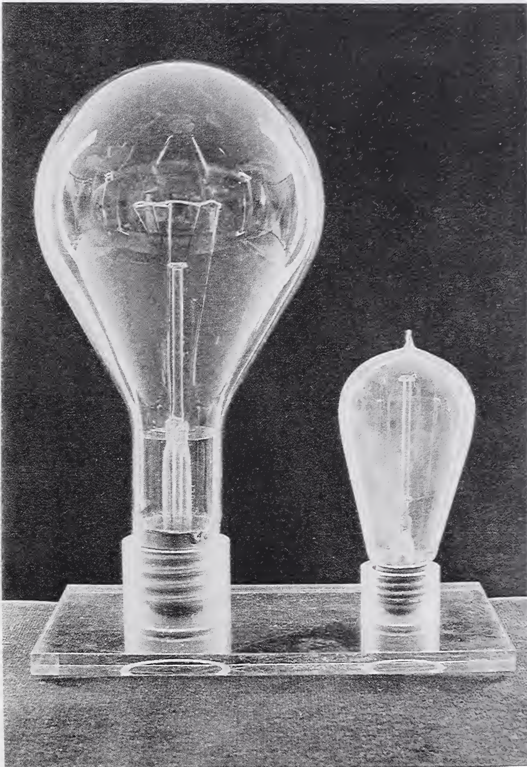
Luminous Flux Standard Lamps (1917 to Present) M229A, 229B
