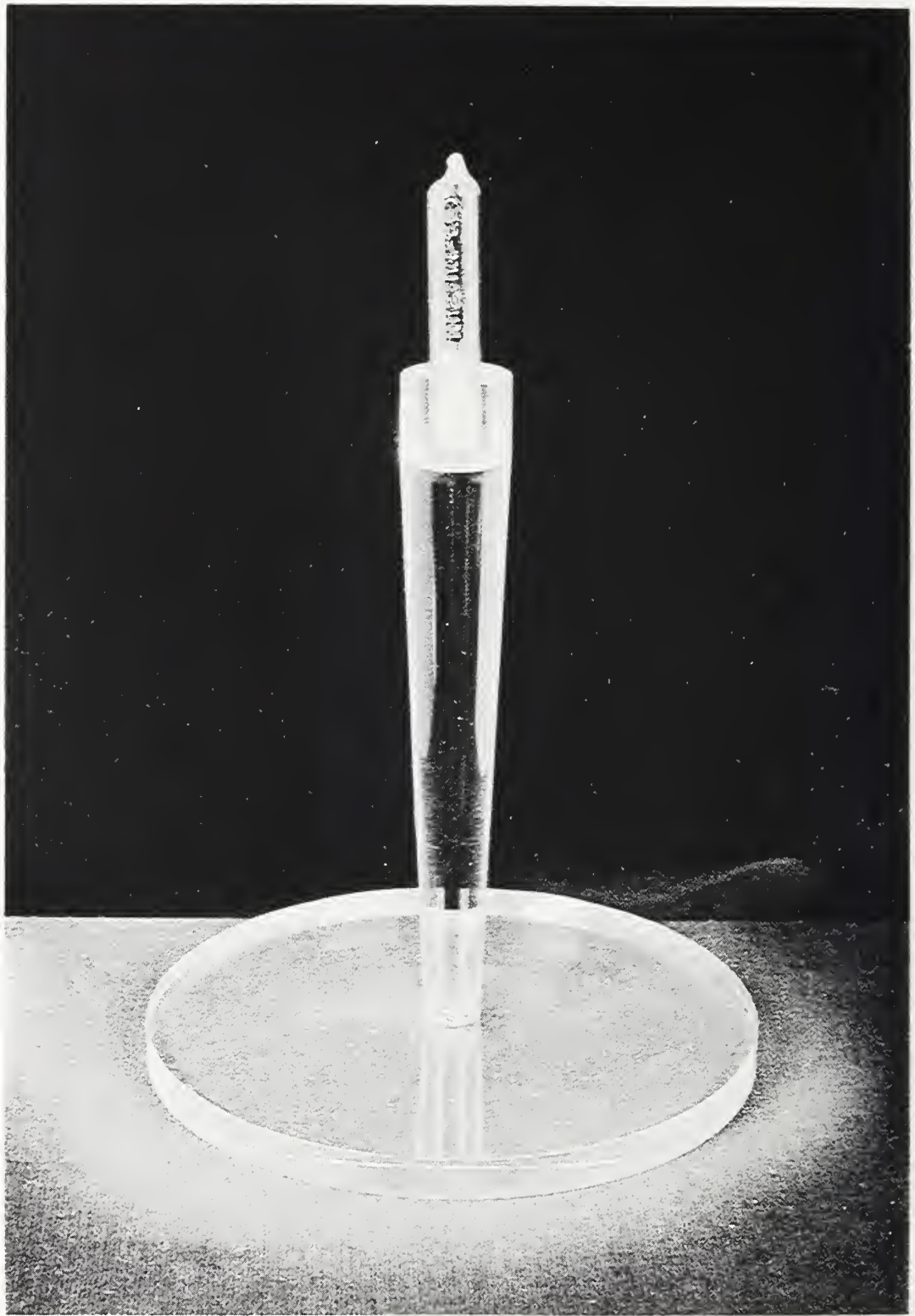
Uranyl Nitrite Crystals (1941) M82
