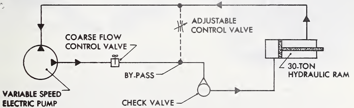
Figure 2.10 - Schematic of hydraulic loading system.
