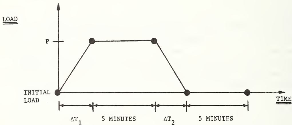
Figure 6.2 - Load-time schematic diagram.
