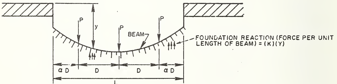
Figure 6.A.1 - Beam on elastic foundation.
