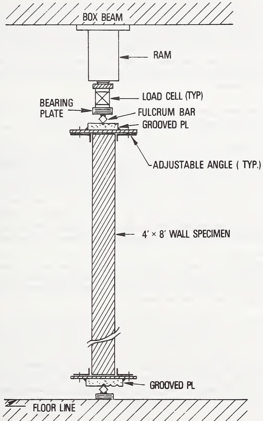
Figure 6.1 - Recommended pin-pin loading setup.
