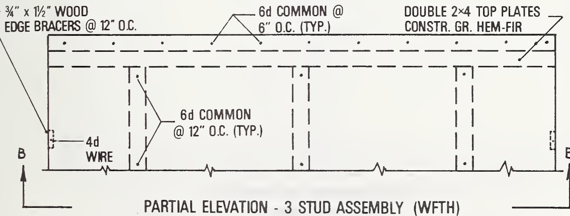
Figure 2.1 - Wood-frame construction test panels (WFFR, WFTH).
