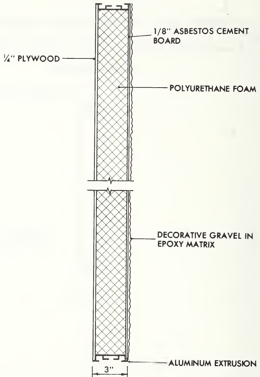
Figure 2.4 - Foamed plastic core sandwich test panel (ACUP).
