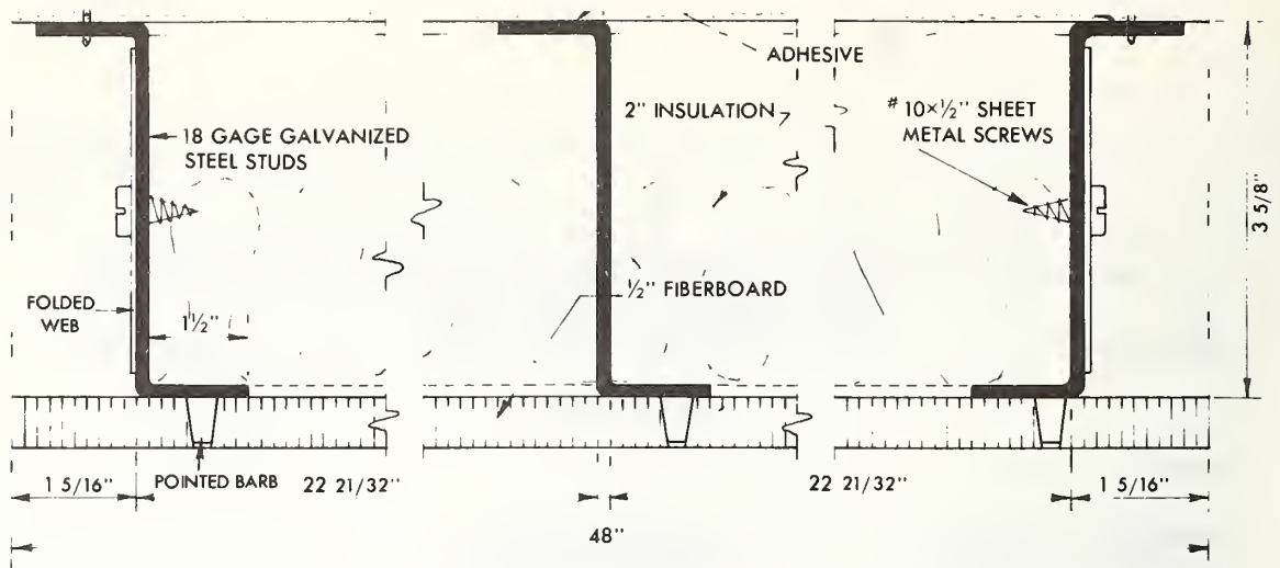
HORIZONTAL SECTION THRU PANEL
