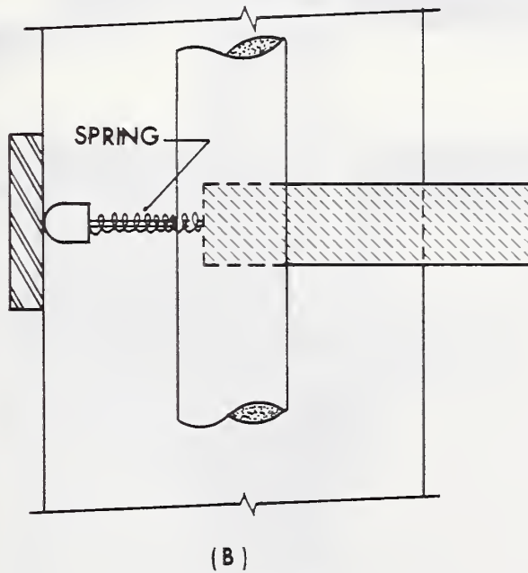
Figure 4.2 - Details of LVDT-core contacting wall-mounted reference plate.
