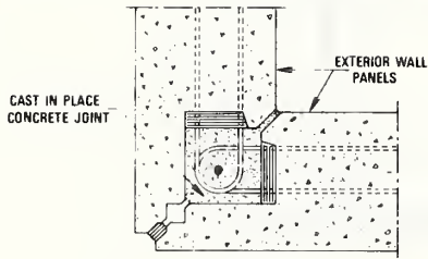
TYPICAL VERTICAL JOINT AT EXTERIOR CORNER
