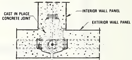
TYPICAL VERTICAL JOINT OF THE INTERSECTION OF EXTERIOR AND INTERIOR PANELS
