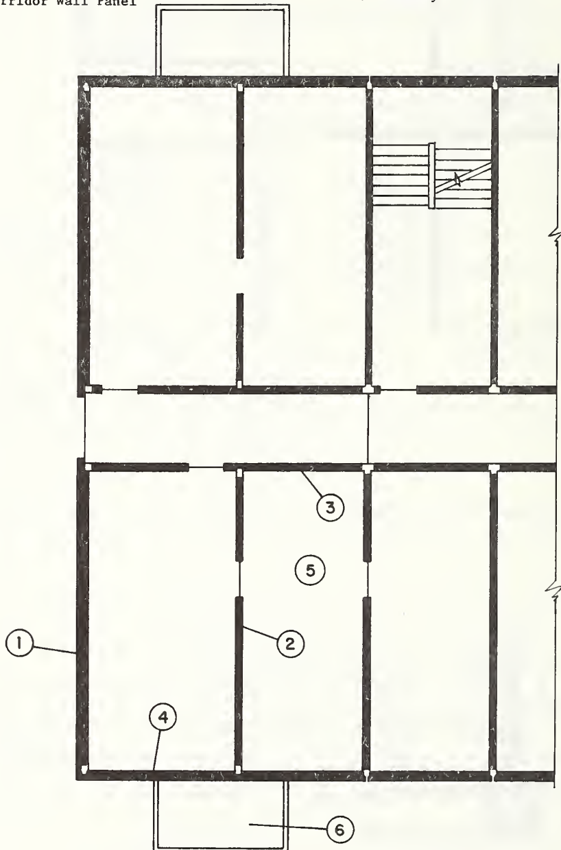
Figure 10 Portion of Typical Floor Plan of Camei System
