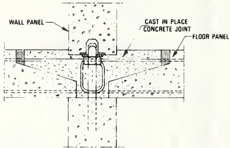
TYPICAL INTERIOR WALL TO FLOOR JOINT
