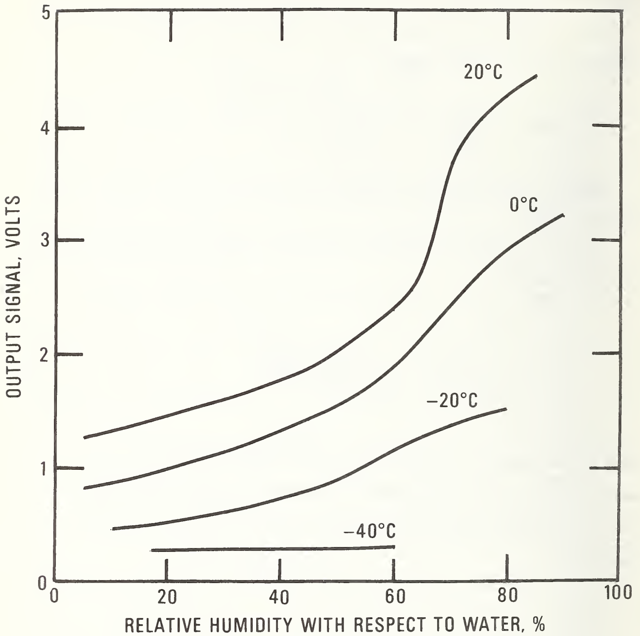
Figure 1. Output Voltage vs Relative Humidity for Sensor #2.
