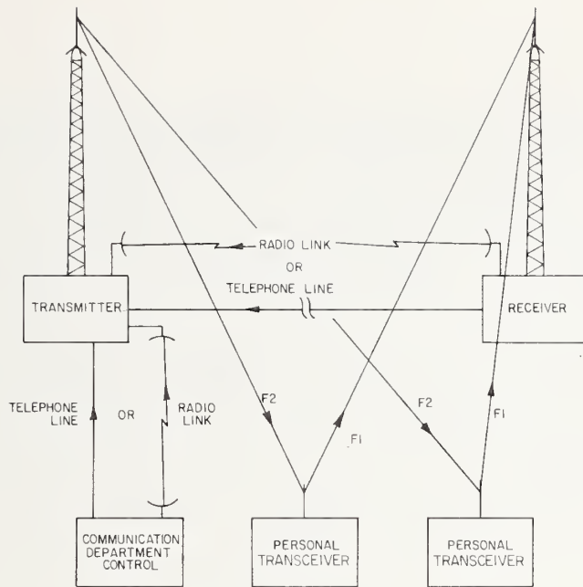
Figure 4. Block diagram of a repeater using two antenna sites.
