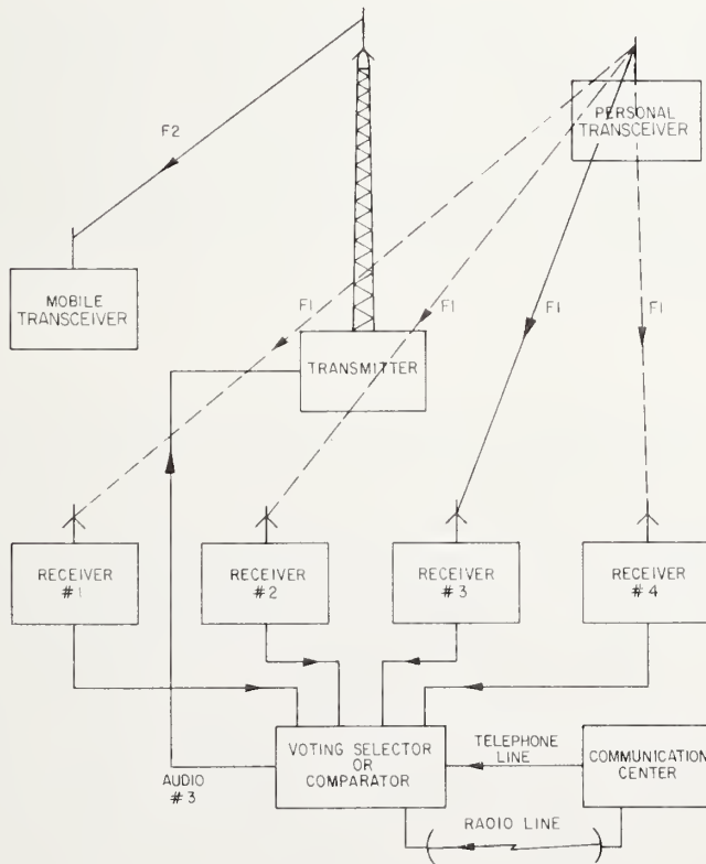
Figure 5. Block diagram of a repeater using voting receivers.
