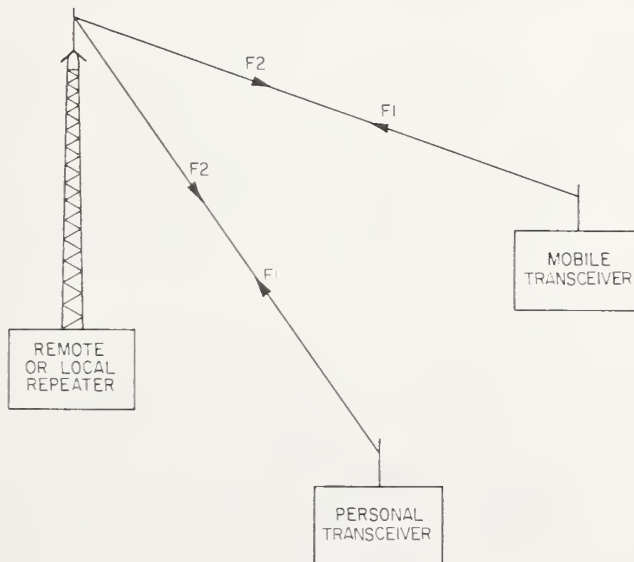
Figure 3. Block diagram of a repeater using single antenna and duplexer.
