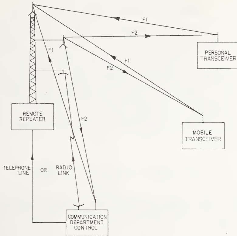
Figure 2. Block diagram of a repeater under remote control.
