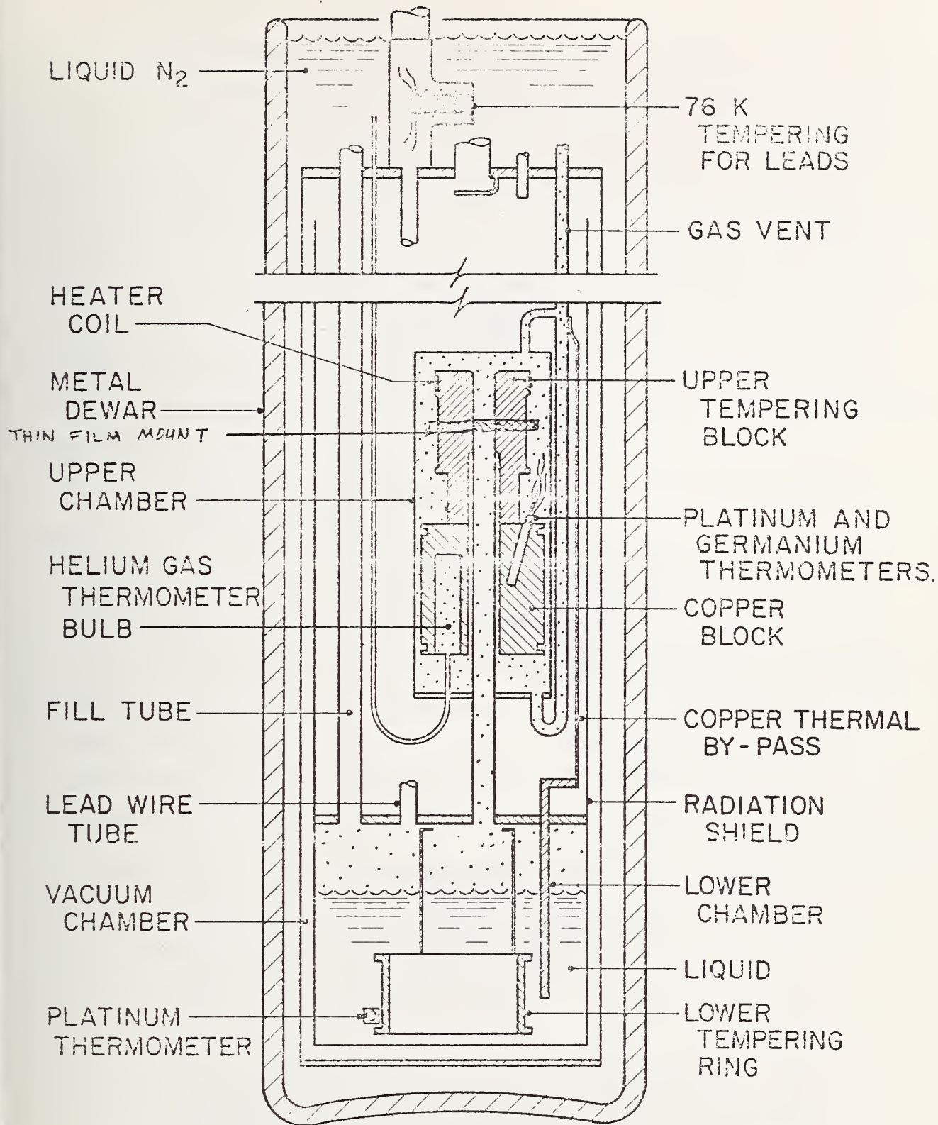
Figure 5. Calibrated cryostat.
