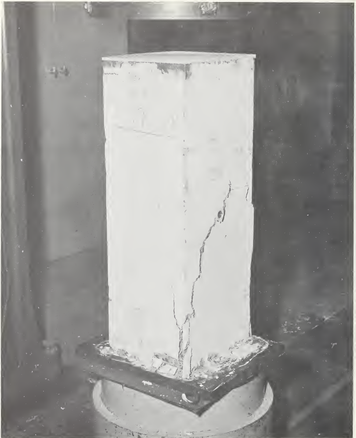
FIGURE 4.8 FAILURE OF COLUMN STUB BEARING ON A STEEL PLATE AND BEDDED IN HIGH STRENGTH GYPSUM
