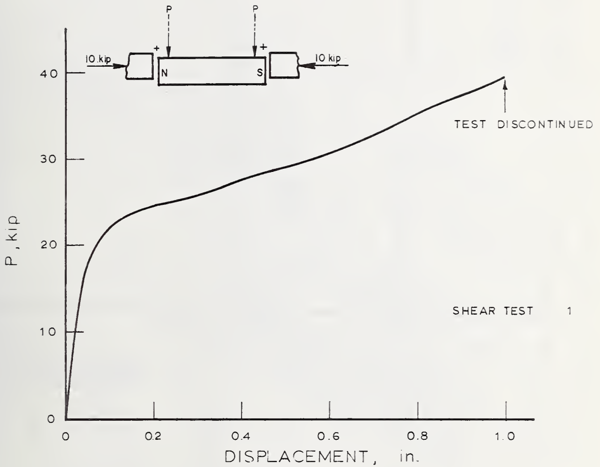
FIGURE 4.25 VERTICAL DISPLACEMENTS OF SOUTH END OF CENTER SEGMENT IN SHEAR TEST 1
