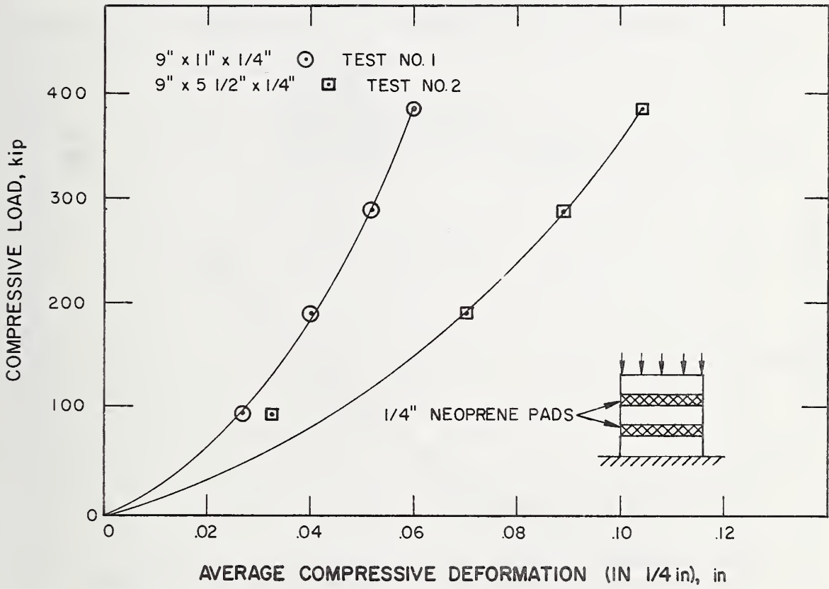
FIGURE 4.11 RELATIONSHIP BETWEEN COMPRESSIVE LOAD AND AVERAGE COMPRESSIVE DEFORMATION OF NEOPRENE PADS
