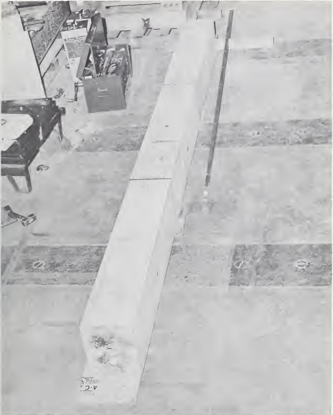
FIGURE 4.21 SPECIMEN ARRANGED FOR PRE-LOADING AND GROUTING OF THE DOWEL
