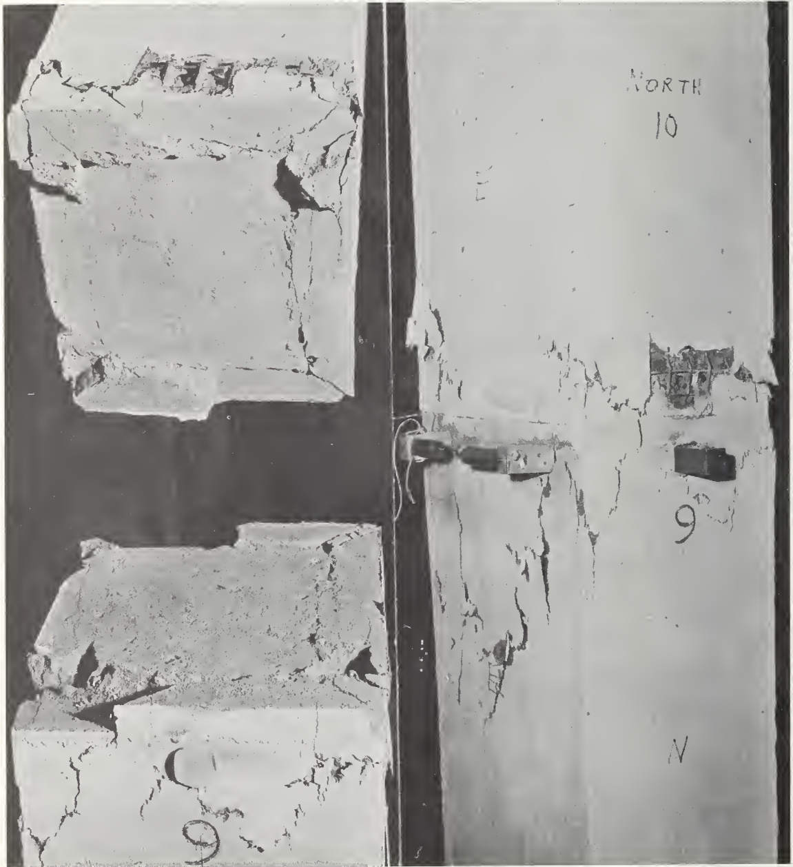
FIGURE 4.6 TYPICAL FAILURE OF A GROUTED CONNECTION
