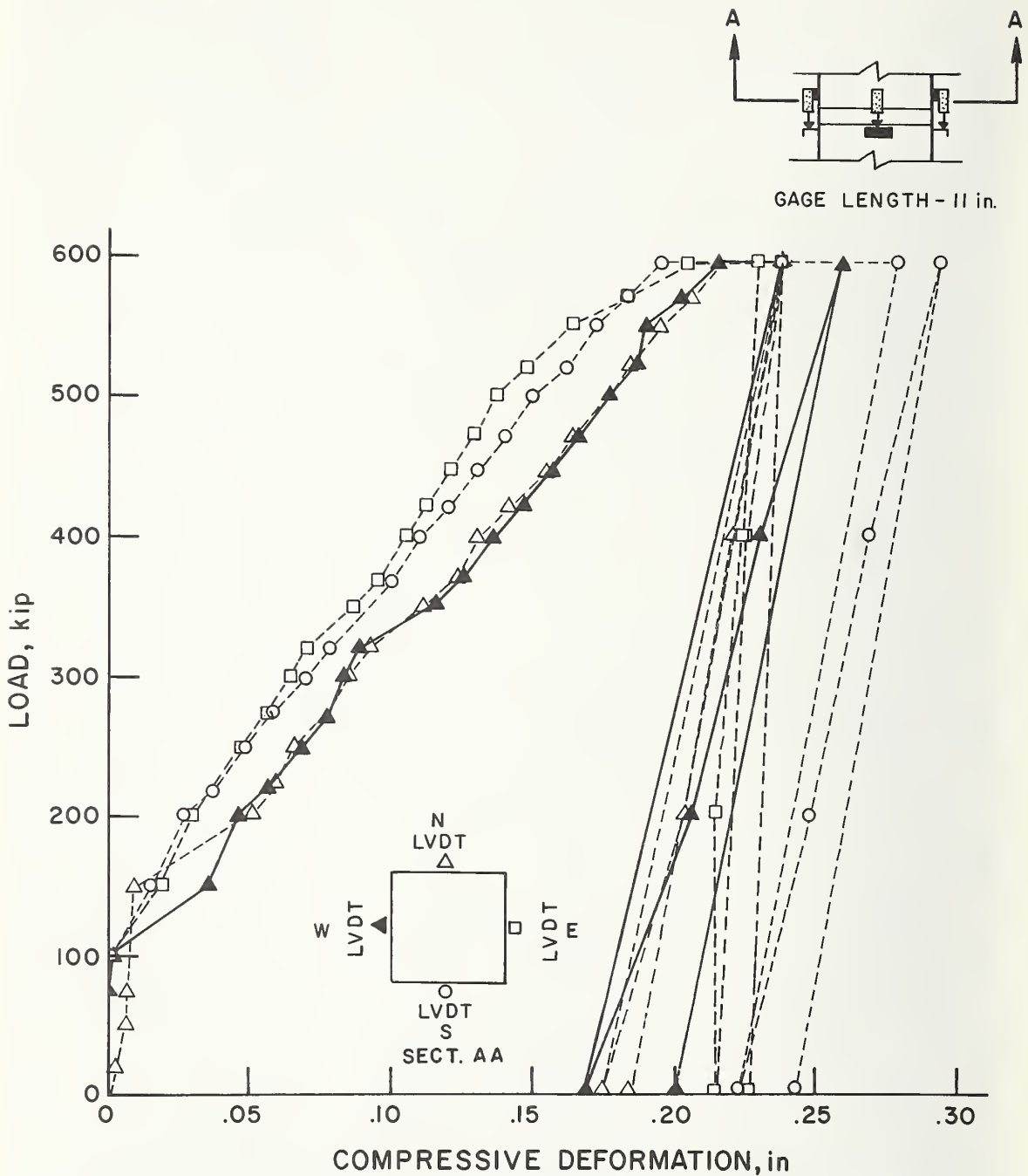
4.16 SPECIMEN WITH GROUTED DOWEL VERTICAL DEFORMATIONS OF AN 11-IN SEGMENT INCLUDING THE JOINT
