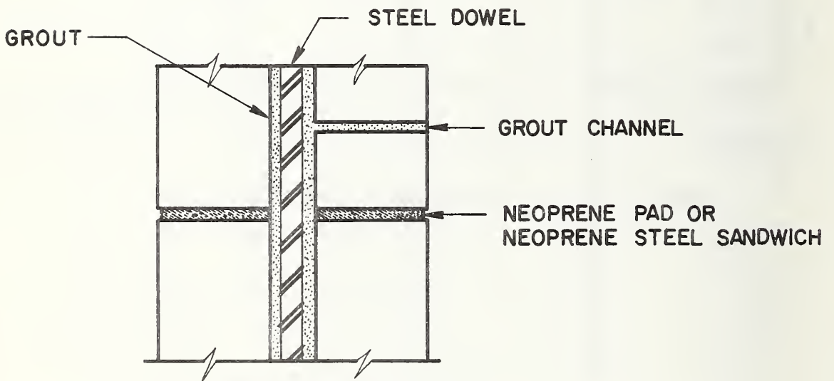
(b) CONNECTION DETAIL
