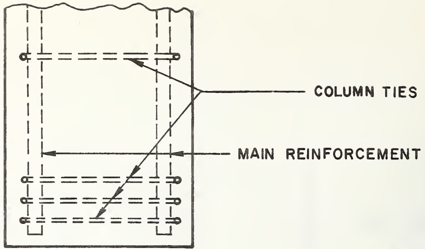
(a) COLUMN REINFORCEMENT AT CONNECTION
