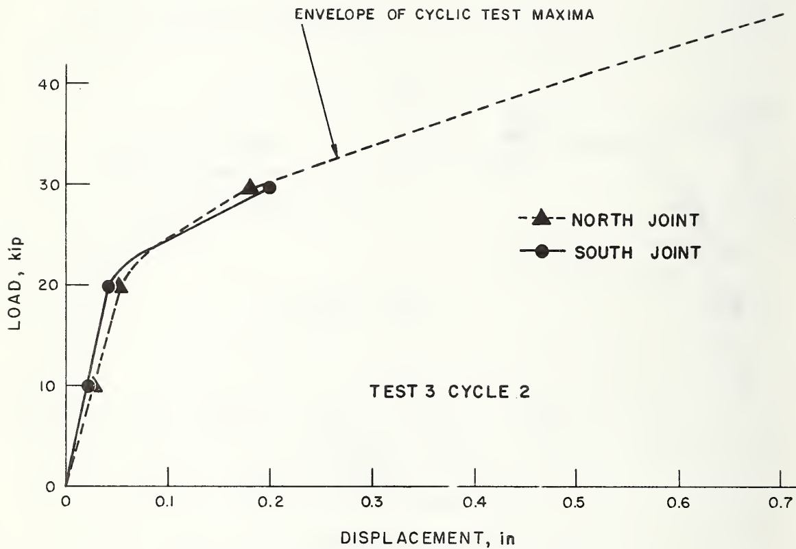
FIGURE 4.32 NET JOINT DISPLACEMENTS IN SHEAR TEST 3
