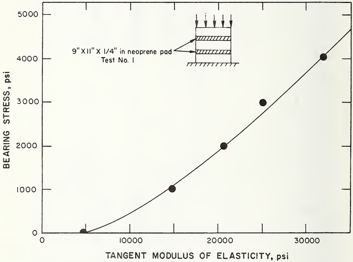
FIGURE 4.12 RELATIONSHIP BETWEEN COMPRESSIVE STRESS AND TANGENT MODULUS OF ELASTICITY FOR THE FULL-SIZED NEOPRENE PADS
