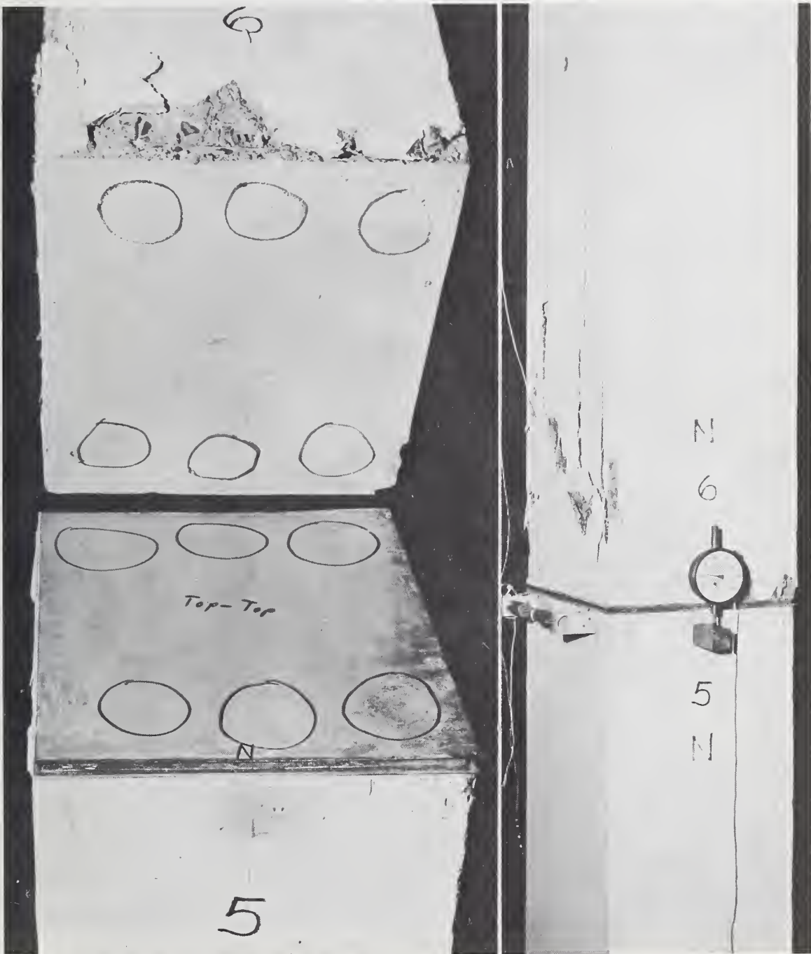
FIGURE 4.7 TYPICAL FAILURE OF CONNECTION USING A STEEL-NEOPRENE-STEEL SANDWICH
