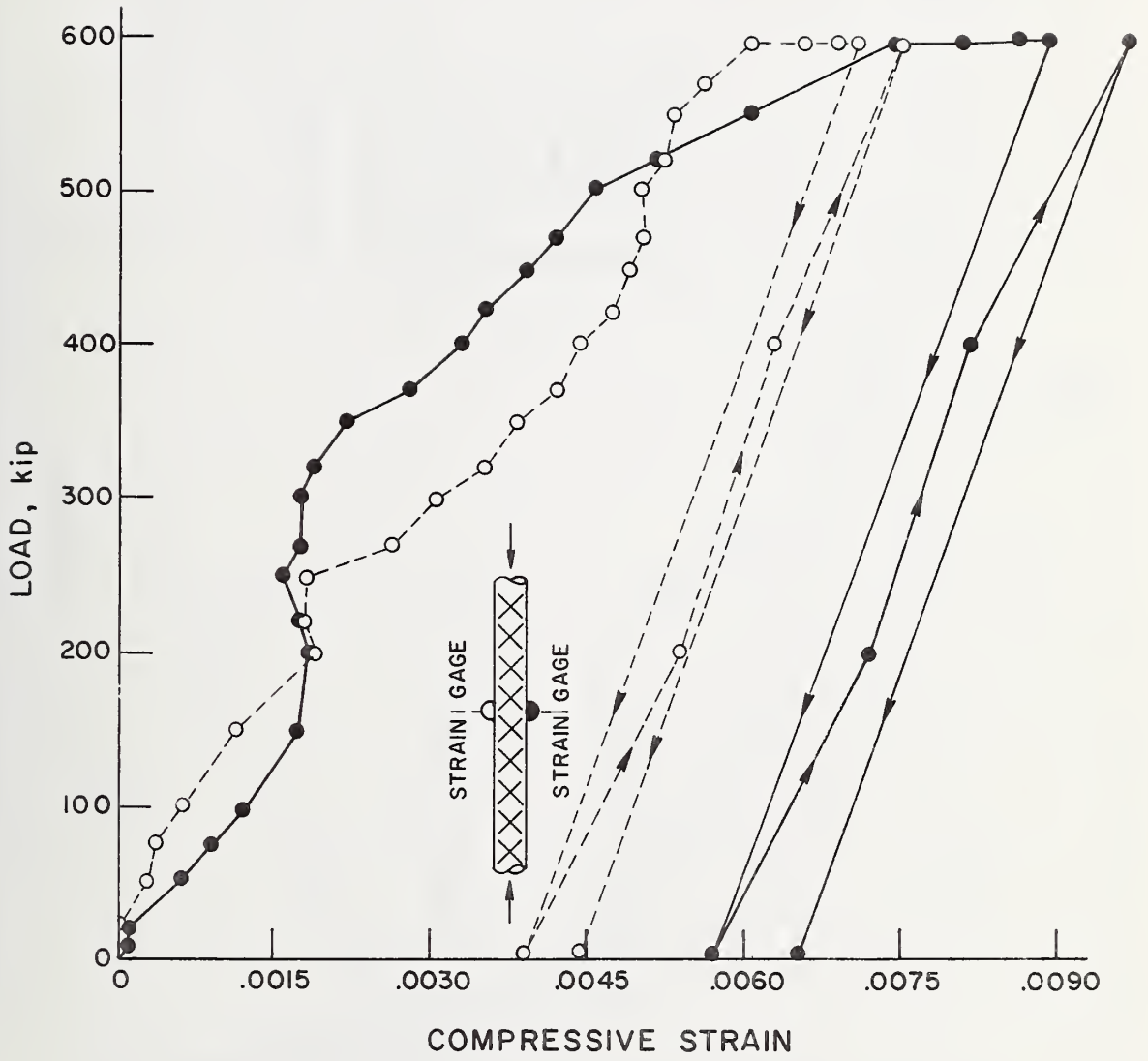
4.17 SPECIMEN WITH GROUTED DOWEL, LONGITUDINAL DOWEL STRAIN IN THE JOINT
