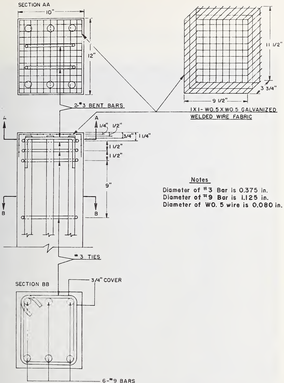
FIGURE 4.3 TYPICAL DETAILS OF TEST SPECIMENS
