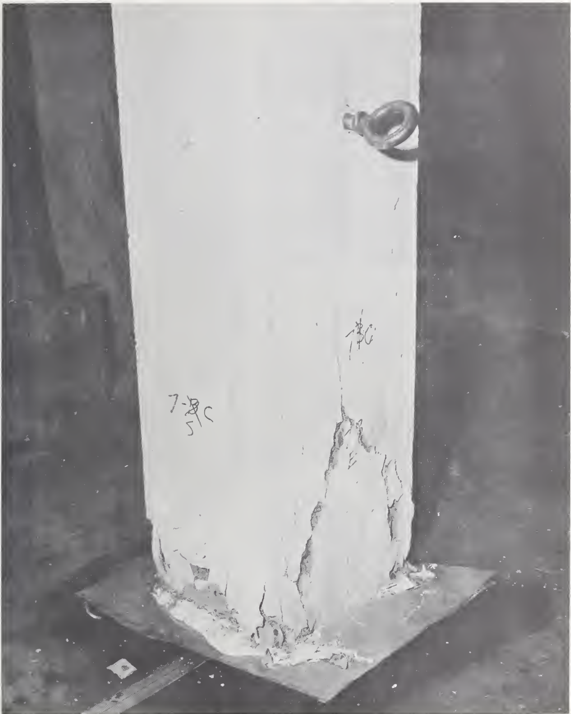
FIGURE 4.9 FAILURE OF COLUMN STUB BEARING ON A STEEL PLATE COVERED BY A LOW FRICTION MEMBRANE.
