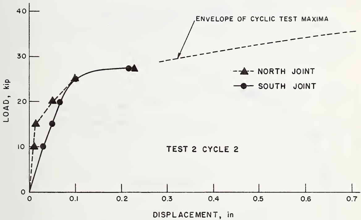
FIGURE 4.31 NET JOINT DISPLACEMENTS IN SHEAR TEST 2
