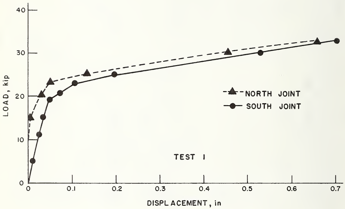
FIGURE 4.30 NET JOINT DISPLACEMENT IN SHEAR TEST 1
