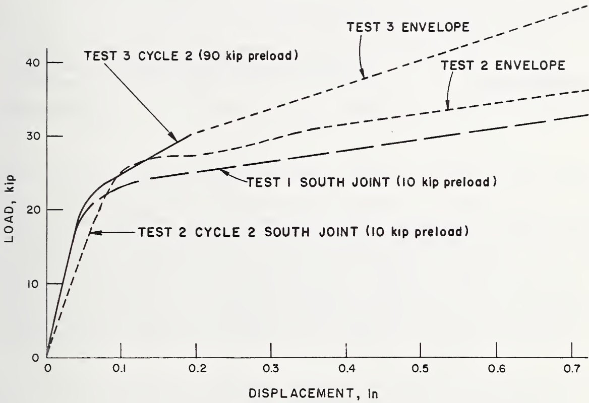
FIGURE 4.33 COMPARISON OF NET JOINT DISPLACEMENTS IN SHEAR TESTS 1, 2, AND 3.
