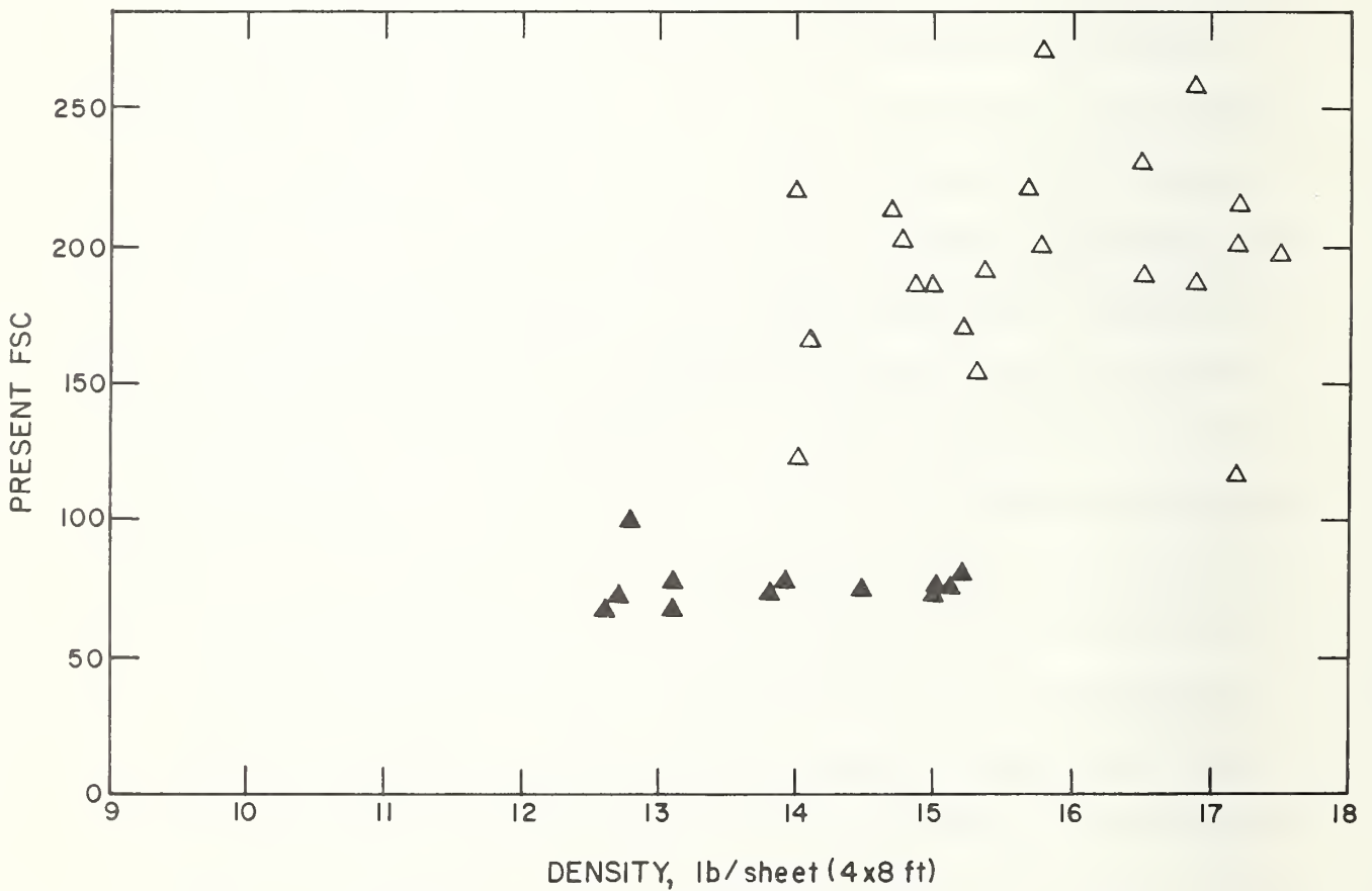
FIGURE 8. FSC AS FUNCTION OF DENSITY OF SPECIMEN #3 BASED ON THE PRESENT (BOTTOM) AND "RATE" (TOP) FORMULAS. ▲ DATA AFFECTED BY CHANGE OF FORMULA.
