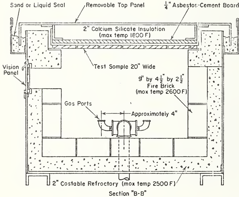
FIG. 1—Test Furnace Showing Critical Dimensions.
