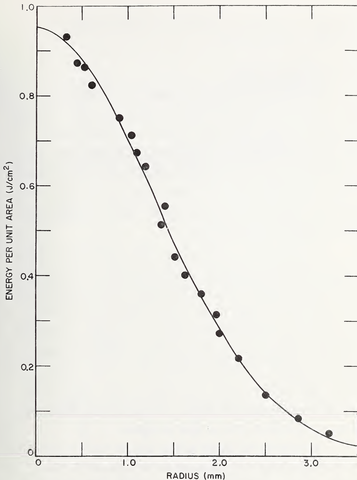
Fig. 2. Beam Profile. Energy per unit area as a function of distance from laser beam axis as measured at the focusing lens. The solid line is a Gaussian fit to the data.
