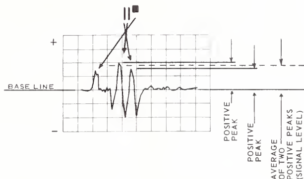
Fig. 24 Wave Form as It Appears on Face of Oscilloscope
