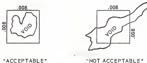
Fig. 22 Example of Single Voids
