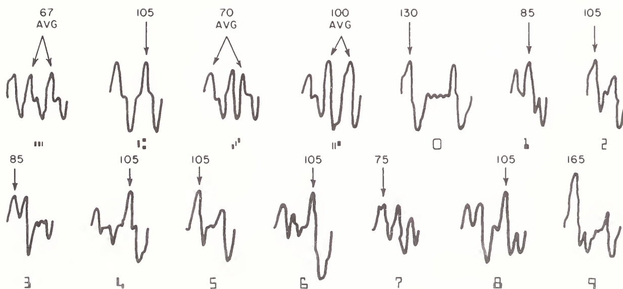
Fig. A4 Waveform Peaks for Signal Level Measurement
