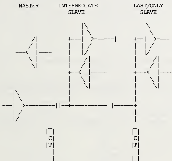
FIGURE 11 CONFIGURATION FOR BIDIRECTIONAL BUS SIGNALS
