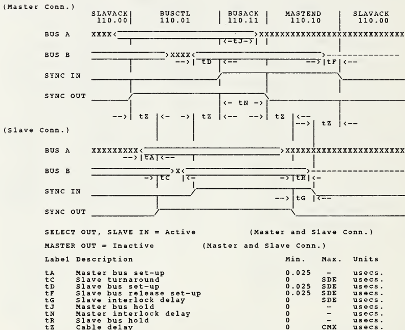
FIGURE 51 BUS CONTROL SEQUENCE (Preceding Transfers In)
