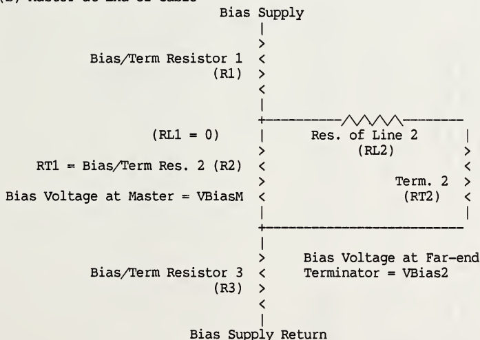
FIGURE F1 THE TWO SUBSYSTEM ARRANGEMENTS WITH PARAMETER LABELS
