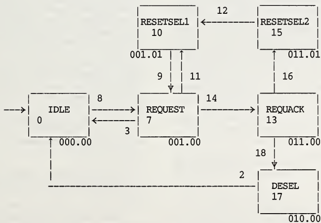
FIGURE 21 SELECTIVE RESET SEQUENCE
