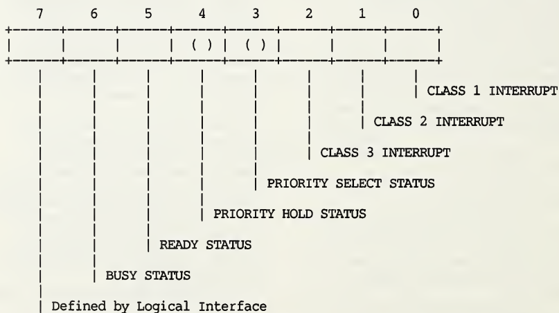
FIGURE 41 SLAVE INTERRUPTS OCTET
