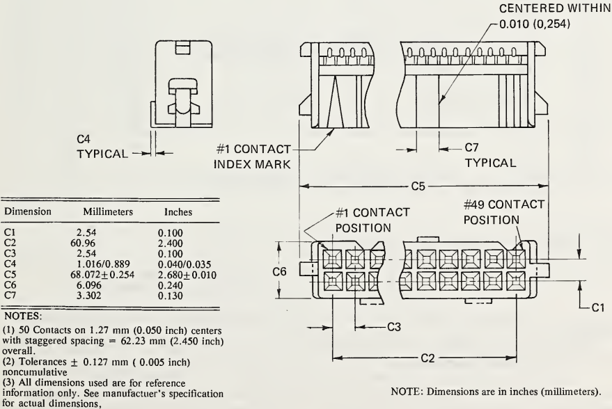
FIGURE 3 2 x 25 PIN HEADER - PLUG
