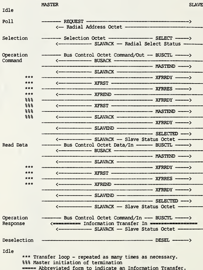
FIGURE A1 State Sequences for Information Transfer
