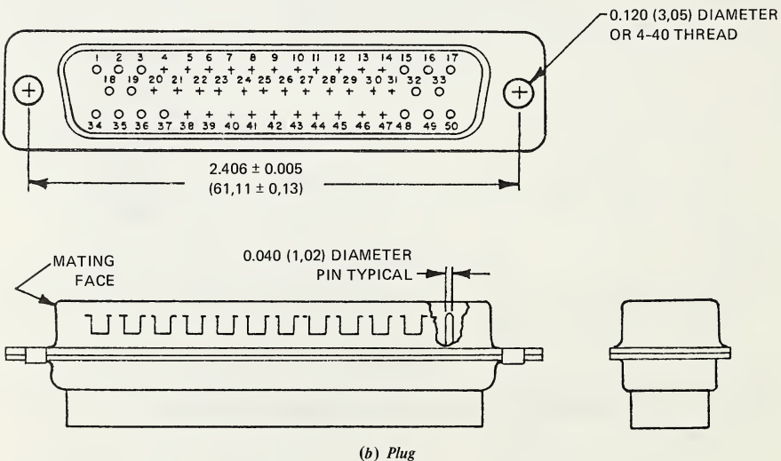
FIGURE 6 50-POSITION SUBMINIATURE "D" RECEPTACLE/PLUG
