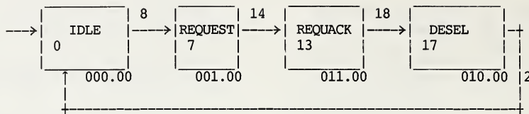
FIGURE 17 REQUEST TRANSFER SETTINGS SEQUENCE
