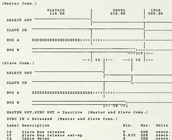
FIGURE 47 NORMAL DESELCTION SEQUENCE
