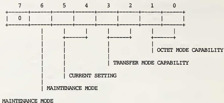
FIGURE 40 TRANSFER SETTINGS OCTET
