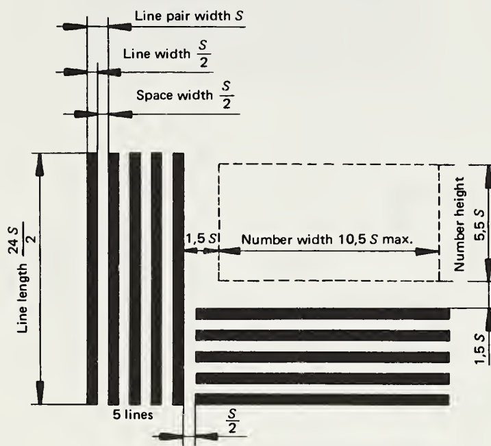
Figure 3A. Resolution test pattern
