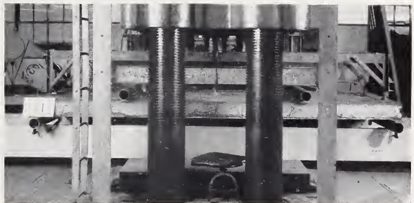
FIGURE 3.—Floor specimen AG-T1 under transverse load.
