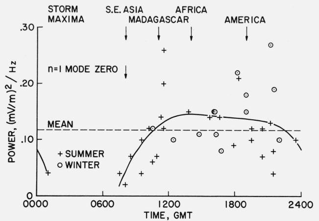
FIGURE 10. Diurnal variation of the power in the fundamental ( n=1 ) mode.
