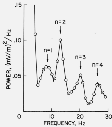
FIGURE 5. Spectrum of the natural vertical electric field observed at 16.18 GMT on January 12, 1963.
