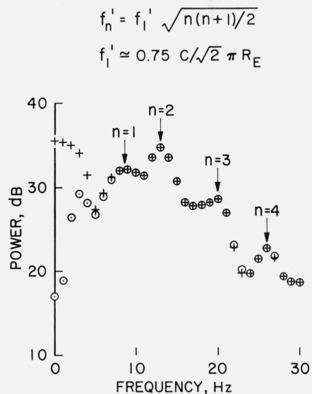
FIGURE 4. Spectrum of the digitized signal waveform observed at 16.18 GMT on January 12, 1963.
