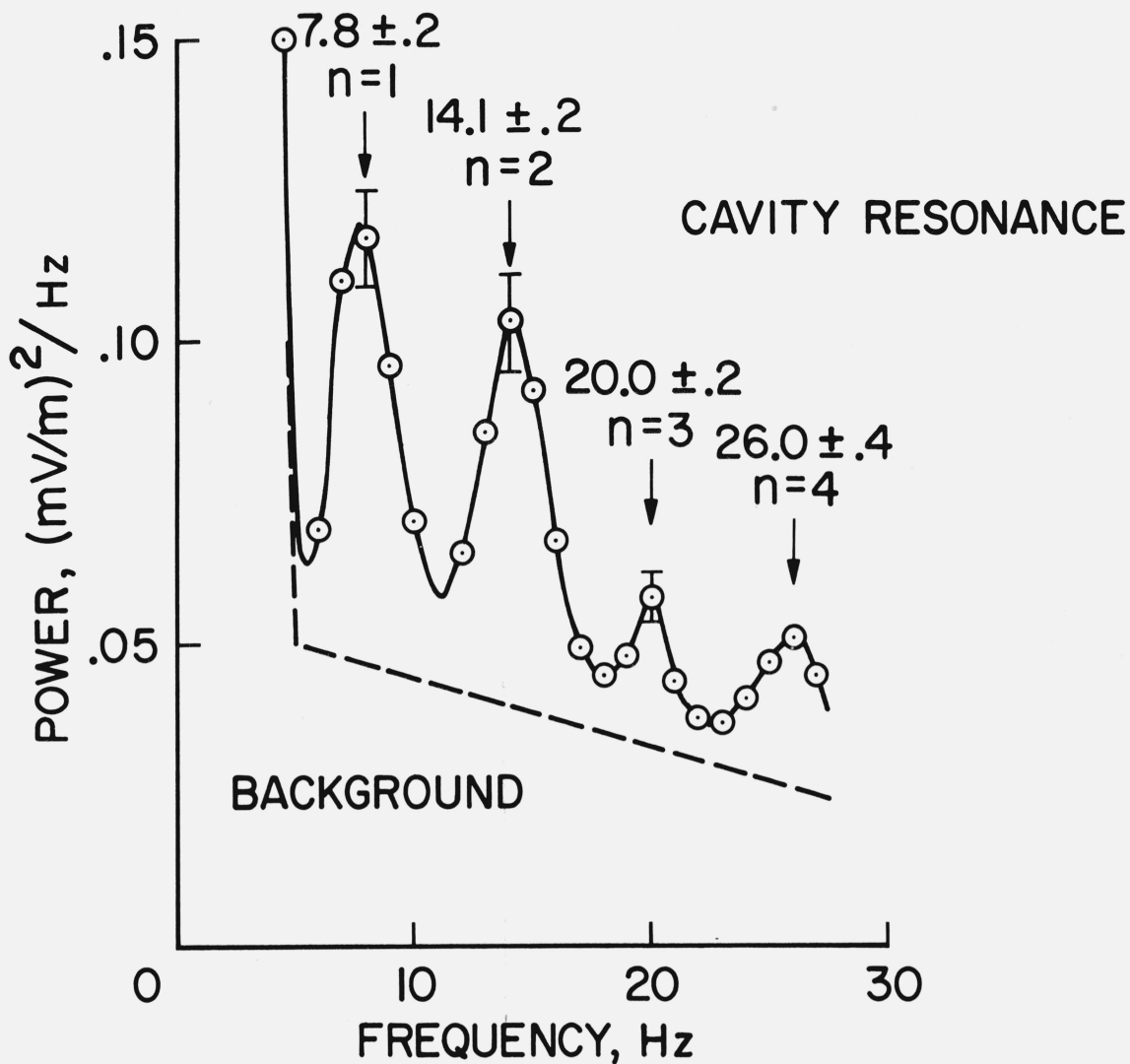
FIGURE 6. Mean ELF spectrum of the natural vertical electric field observed in 1962 and 1963.
