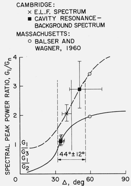
FIGURE 8. Ratio of the power, G_1 , in the fundamental ( n=1 ) mode to that in the higher harmonic ( n=2 and 3) modes as a function of \Delta , the half width of the equatorial thunderstorm belt.
