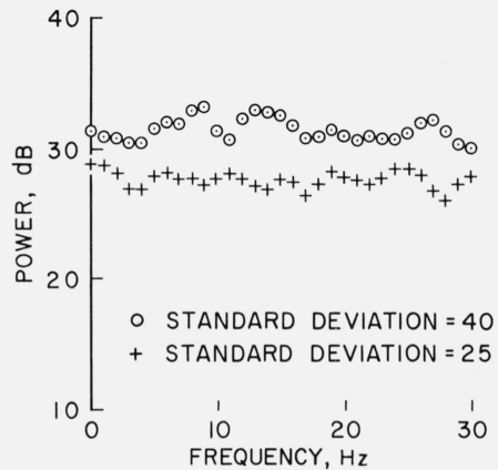
FIGURE 3. Spectra of two series of 600 random numbers, 0 with a standard deviation of 40 about a mean of 130, and + with a standard deviation of 25.
