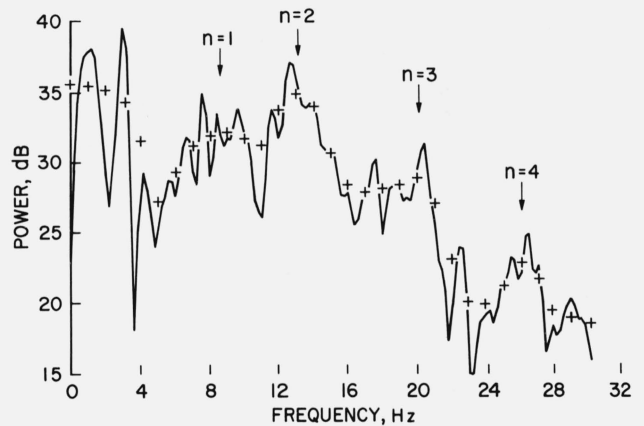
FIGURE 11. Spectrum of the digitized signal waveform observed at 16.18 GMT on January 12, 1963, computed at 0.2-Hz intervals (solid line).
