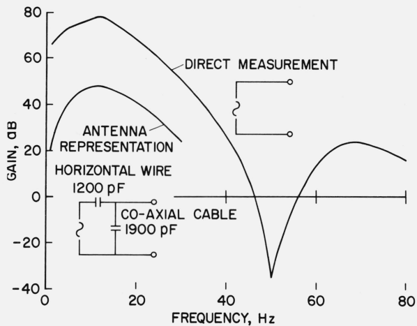
FIGURE 1. Frequency response of the amplifying system.
