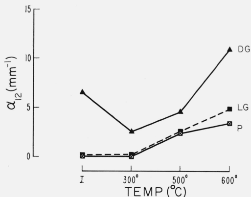
FIGURE 11. Change in \alpha_{12} with heat treatment (No. 2 thermal schedule), for spectral types.
