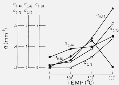
FIGURE 7. Visible spectrum change due to heating for a dark green as described by absorption coefficients (No. 2 schedule).
