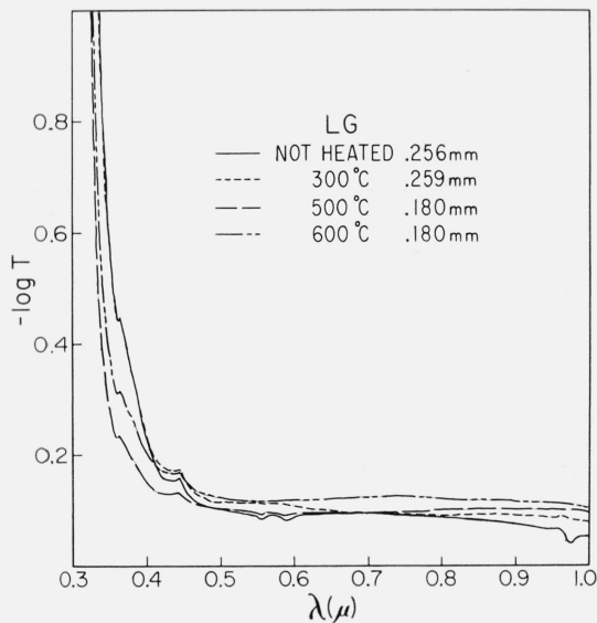
FIGURE 3. Change in the 0.3 to 1 \mu absorption spectrum of a light green with heating for 24 hr at various temperatures (No. 2 schedule).
