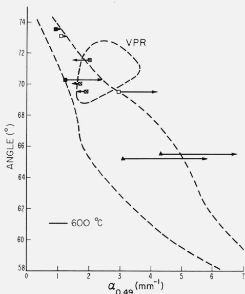
FIGURE 9. The magnitude and direction of change of \alpha_{0.49} due to heating at 600 ^{\circ}\text{C} for 24 hr as a function of initial coordinates.
