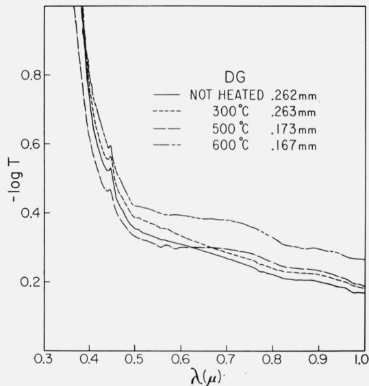
FIGURE 4. Change in the 0.3 to 1 \mu absorption spectrum for a dark green with heating for 24 hr at various temperatures (No. 2 schedule).
