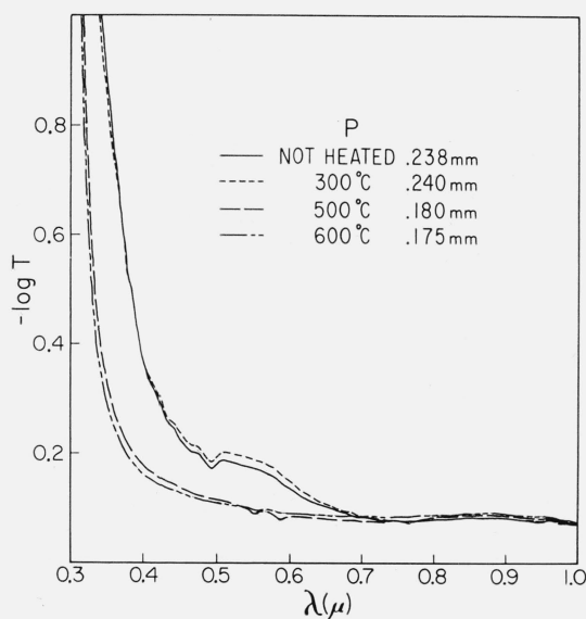
FIGURE 2. Change in the 0.3 to 1 μ absorption spectrum of a pink ruby with heating for 24 hr at various temperatures (No. 2 schedule).
