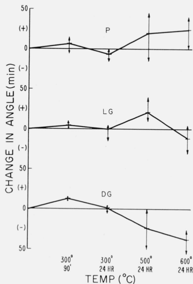
FIGURE 13. Behavior of apparent optic angle with heat schedule for the three spectral types: pink ruby, light green, and dark green.
