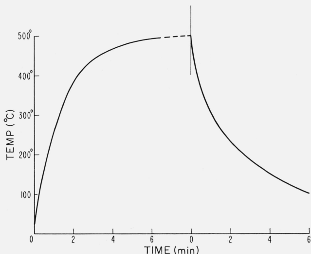
FIGURE 1. Heating and cooling curves for a representative sample subjected to a heating procedure at 500 °C.
