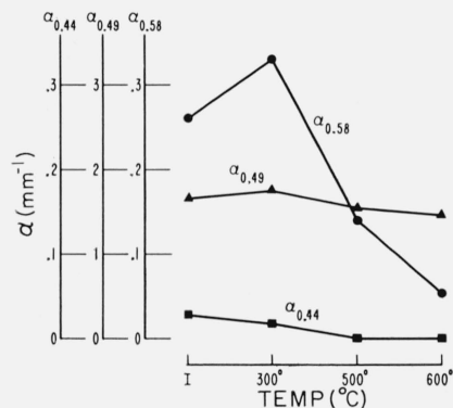
FIGURE 5. Change in visible spectrum of a pink ruby due to heating (No. 2 schedule) as described by absorption coefficients.
