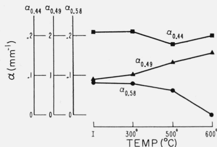
FIGURE 6. Visible spectrum change due to heating for a light green as described by absorption coefficients (No. 2 schedule).
