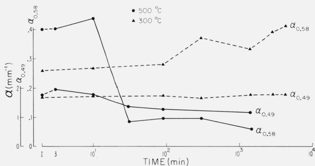
FIGURE 8. Effect of heating on the visible pink associated absorption region of 0.47 to 0.6 \mu and on the height of the absorption edge of a very pink ruby.
