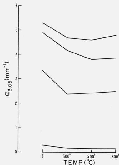
FIGURE 10. Effect of heat treatment on the infrared pink correlated structure as represented by \alpha_{3.05} for various initial values.
