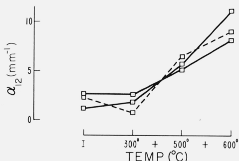
FIGURE 12. Effect of heat treatment on the 12 \mu band of several ruby specimens (No. 4 procedure).
