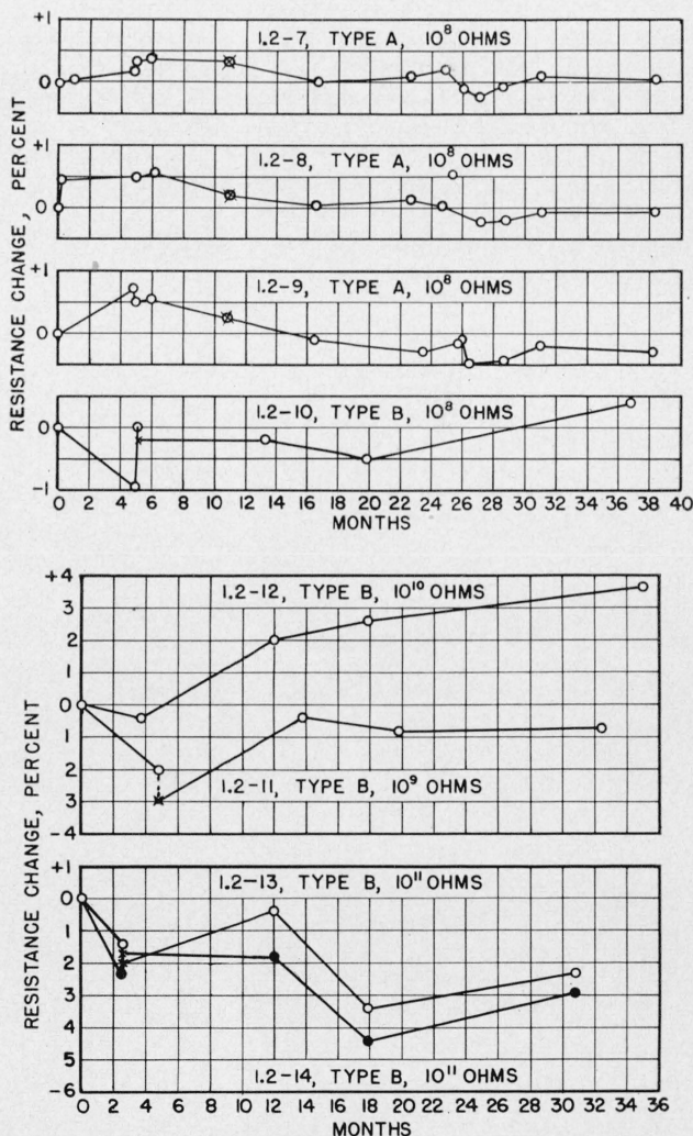
FIGURE 4. Change of resistance of multimegohm resistors with time. The crosses are values obtained after the resistors had been subject to a voltage of 180 volts.
