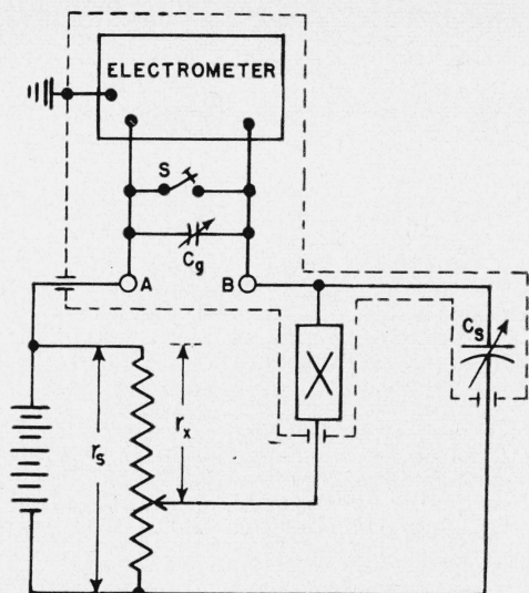
FIGURE 1. Circuit used to measure multimegohm resistors.
