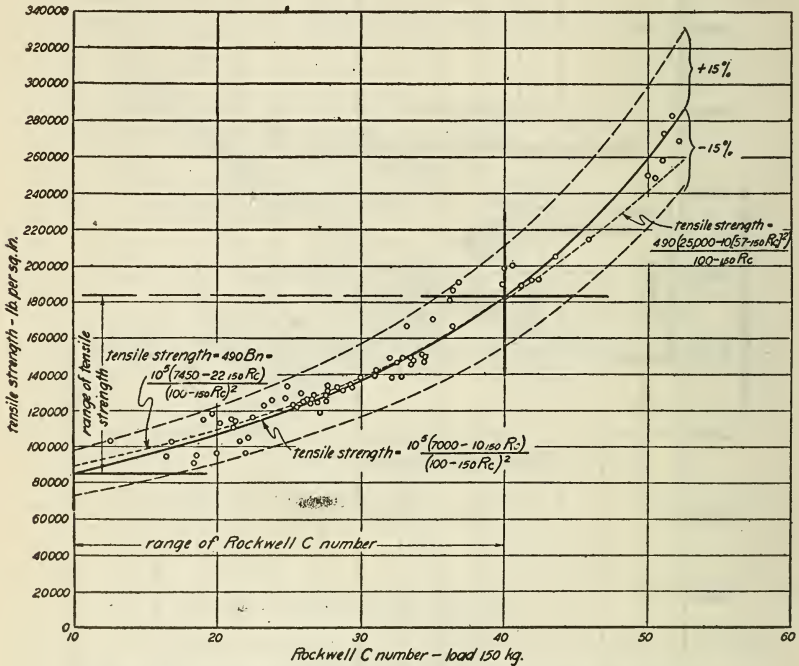
FIGURE 11.—Experimental relationship between the tensile strength of steel and Rockwell cone number
