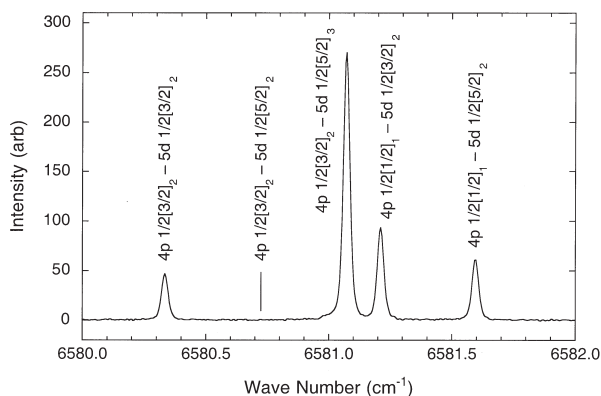
Fig. 4. Ne spectral lines at 15 191 Å ( 6581\text{ cm}^{-1} ). The five classifications shown were assigned to a single experimentally observed feature in Ref. [4]. On this intensity scale the strongest line in the spectrum has intensity 100 000.
