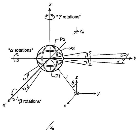
Fig. 3. Geometry for three-axis probe with center of probe in x - z plane. Varying the angle \alpha results in rotations of probes P1 and P2 about the y' -axis ("alpha rotations") while orientation of probe P3 with respect to the dipole remains unchanged. Varying the angle \beta results in rotations of probes P1 and P3 about the x' -axis ("beta rotations") while orientation of probe P2 remains unchanged. Varying the angle \gamma results in rotations of probes P2 and P3 about the z' -axis ("gamma rotations") while orientation of probe P1 remains unchanged.
