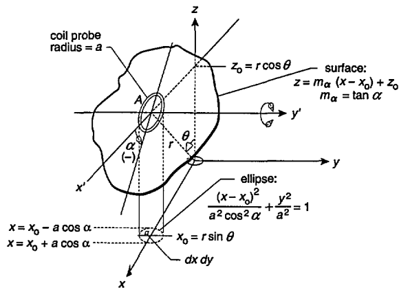
Fig. 2. Circular coil probe shown as part of a surface described by the equation z = m_\alpha(x - x_0) + z_0 . The rotation of the probe corresponds to changing the slope of the surface, m_\alpha . The projection of the probe cross sectional area onto the x - y plane will be an ellipse for \alpha \neq 0 . The range of \alpha is -90^\circ < \alpha < 90^\circ .
