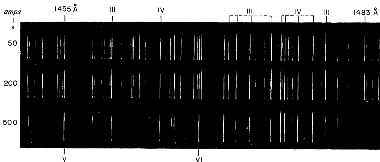
Figure 1. Tungsten spectra.
