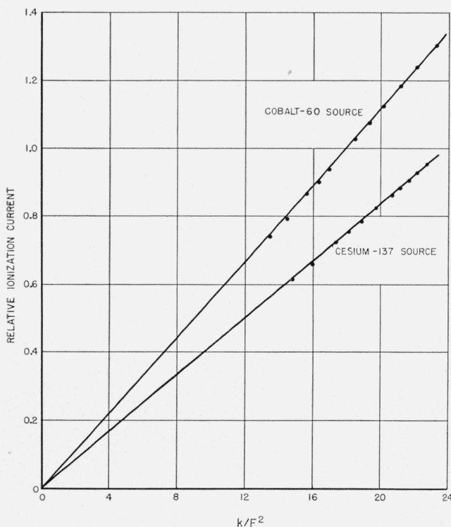
FIGURE 5. Inverse-square plot for the source-diaphragm distance ( F ).
