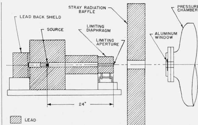
FIGURE 1. Diaphragm system.
