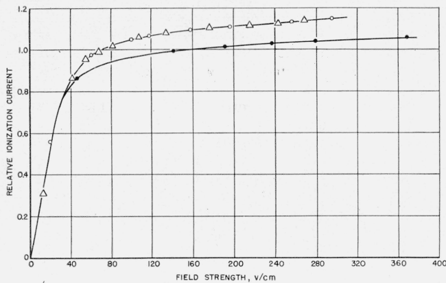
FIGURE 4. Field saturation curves for different plate separations. ●, 9.98 cm; ○, 23.96 cm; △, 35.14 cm.
