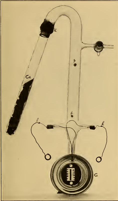
FIG. 1.— Vacuum thermopile
