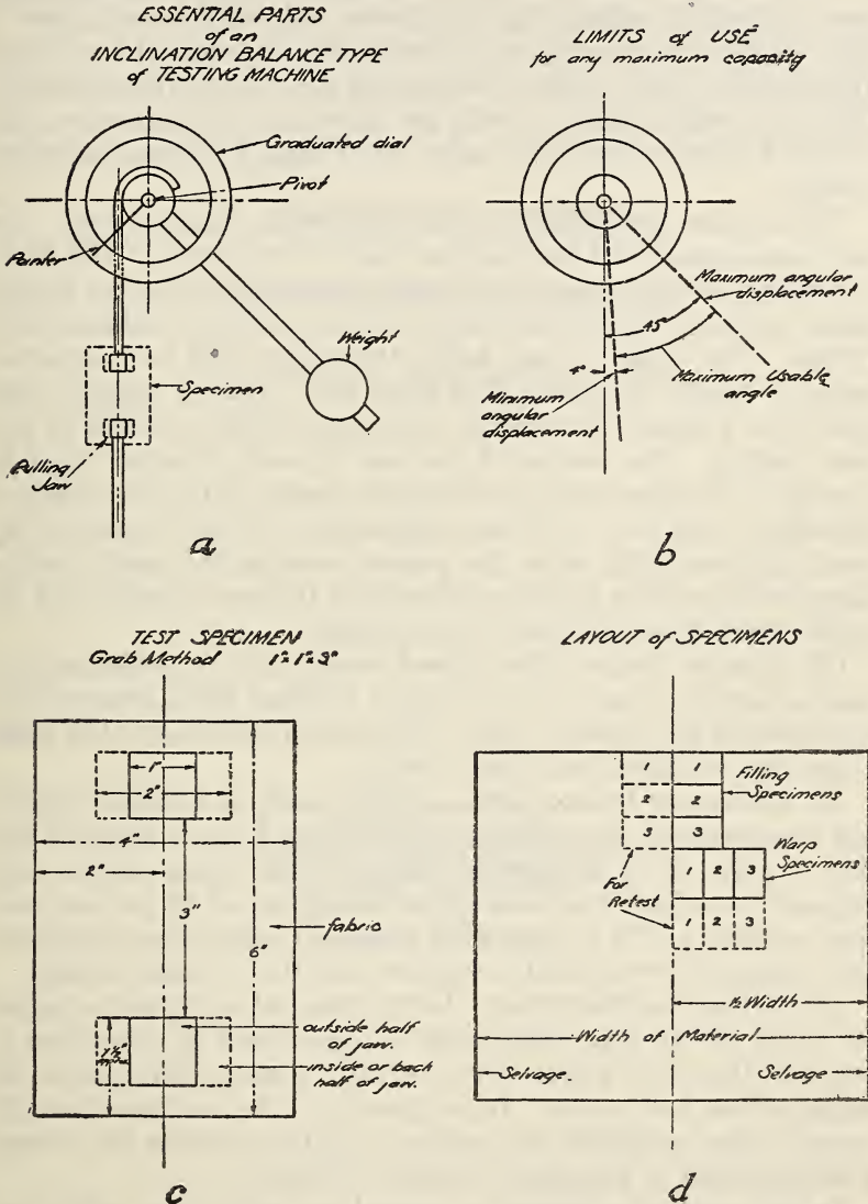
FIG. 1.—Type of machine, limits of use, layout and dimensions of specimens
