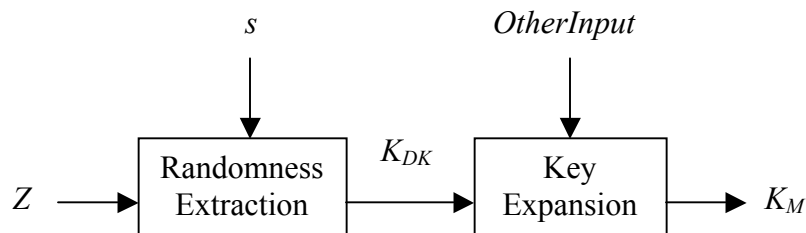
Figure 1: Extraction-then-Expansion Procedure
