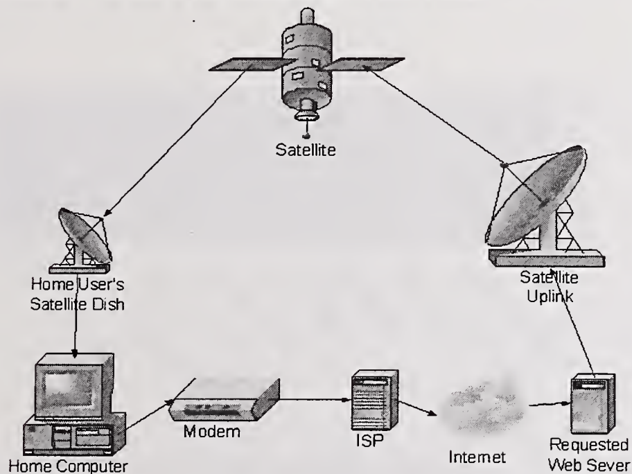
Figure 2.2: Satellite Broadband Network Architecture
