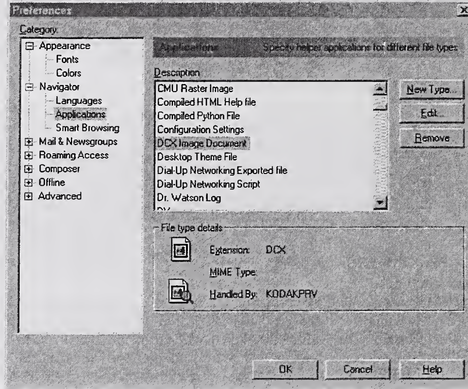
Figure 4.1: Netscape Plugins
