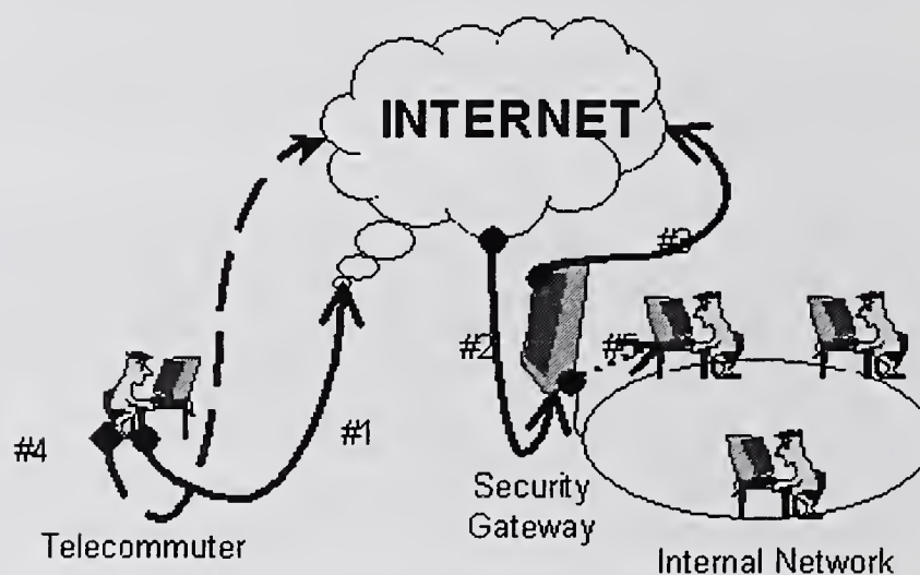
Figure 7.1: VPN Example
