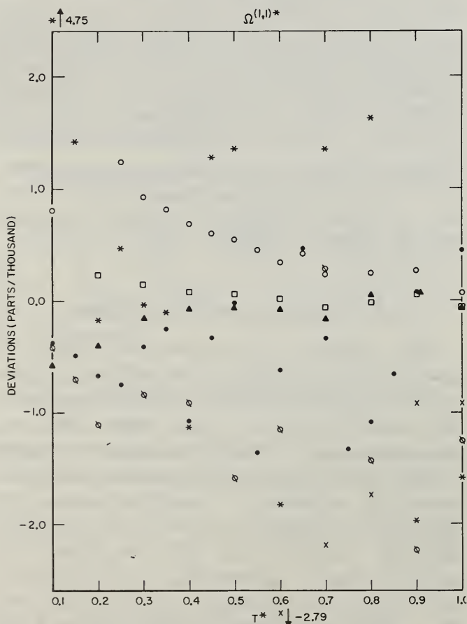
FIGURE 1. Deviations of published tables of \Omega^{(1,1)*} for the (12, 6) potential in the temperature range 0.1 \leq T^* \leq 1.0 .
