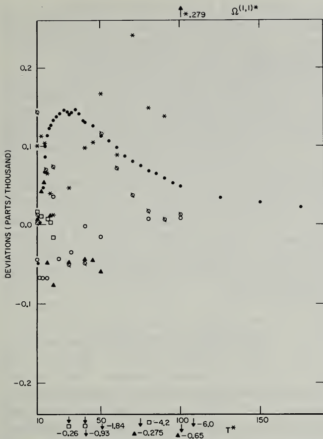
FIGURE 3. Deviations of published tables of \Omega^{(1,1)*} for the (12, 6) potential in the temperature range 10 \leq T^* \leq 200 .
