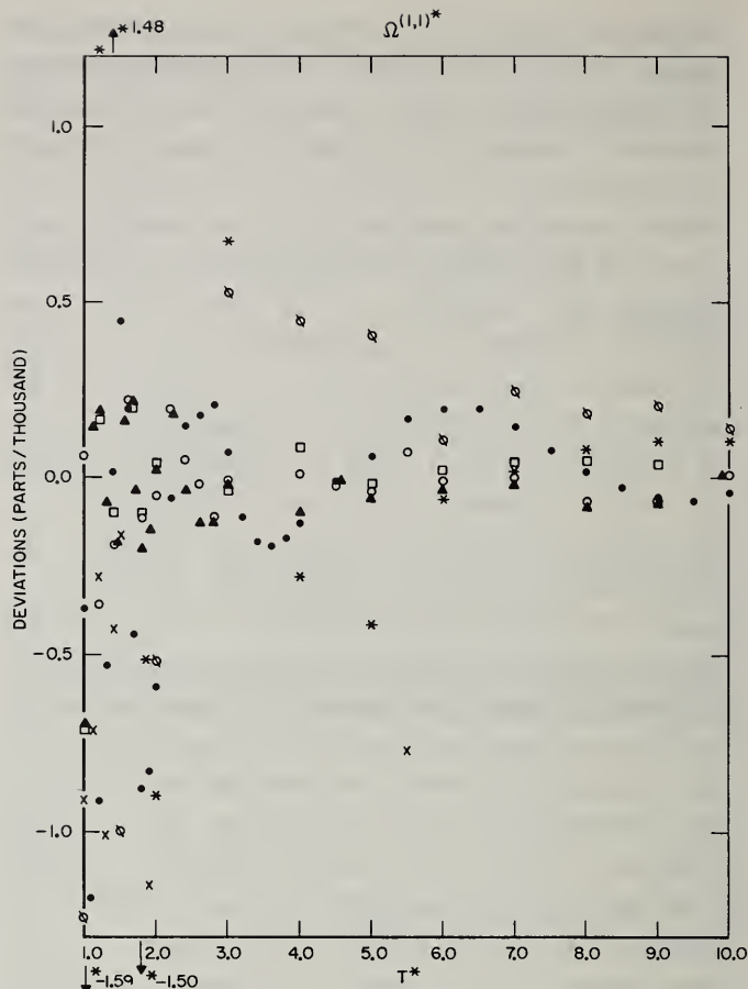
FIGURE 2. Deviations of published tables of \Omega^{(1,1)*} for the (12, 6) potential in the temperature range 1.0 \leq T^* \leq 10 .
